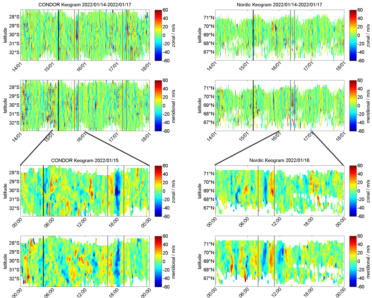
Figure 3. Latitudinal keograms of the vertical average zonal and meridional winds for both domains (upper panels). The lower panels represent shorter time sections of the first event above CONDOR and the one event at the Nordic Meteor Radar Cluster. Vertical lines are explained in the caption of Figure 2.
