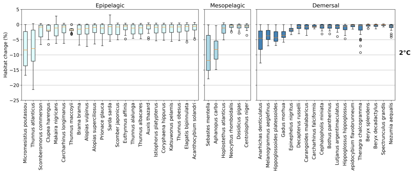
Figure C6 Habitat change (%) of contemporary (1995–2014) habitat volume for 2°C global warming, including 5 levels of AGI crit in every species' boxplot (number of datapoints n=5 AGI crit levels * 6 models = 30): AGI crit is taken as the minimum in-habitat AGI value, the 5 th percentile, the 10 th percentile, the 15 th percentile and the 20 th percentile, respectively. Note the different y-axis when
