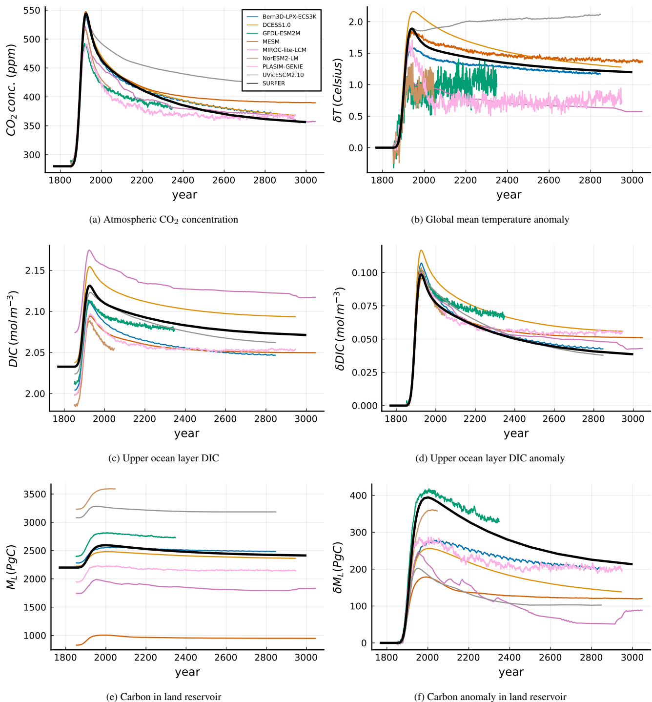
Figure 9. ZECMIP B1 experiment outputs of 6 EMICs, 2 ESMs and SURFER. From left to right, top to bottom: CO 2 concentration in the atmosphere, atmospheric global mean temperature anomaly, dissolved inorganic carbon in the upper layer, dissolved inorganic carbon anomaly in the upper layer, total of carbon in the land reservoir and carbon anomaly in land reservoir.
