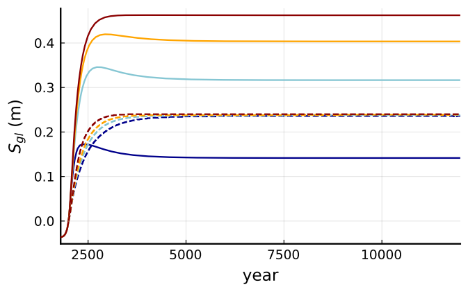
(c) Glacier contribution to sea level rise
