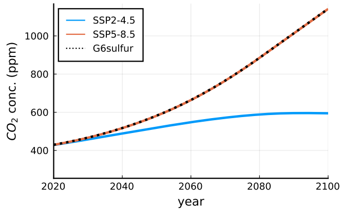
(a) Atmospheric CO 2 concentration
