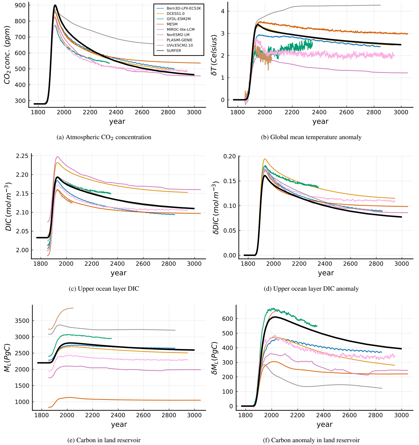
Figure 10. ZECMIP B3 experiment outputs of 6 EMICs, 2 ESMs and SURFER. From left to right, top to bottom: \text{CO}_2 concentration in the atmosphere, atmospheric global mean temperature anomaly, dissolved inorganic carbon in the upper layer, dissolved inorganic carbon anomaly in the upper layer, total of carbon in the land reservoir and carbon anomaly in land reservoir.
