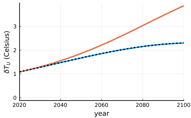
(c) Global mean temperature anomaly
