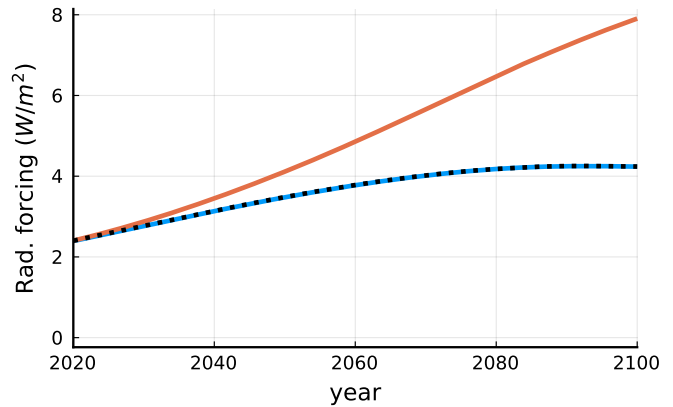
(b) Anthropogenic radiative forcing
