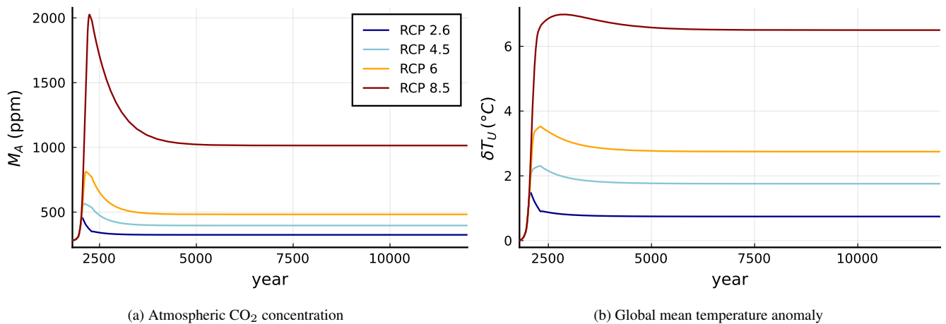
Figure 15. SURFER's long-term prediction for CO 2 concentration and global mean temperature anomaly when forced by extended RCP scenarios.
