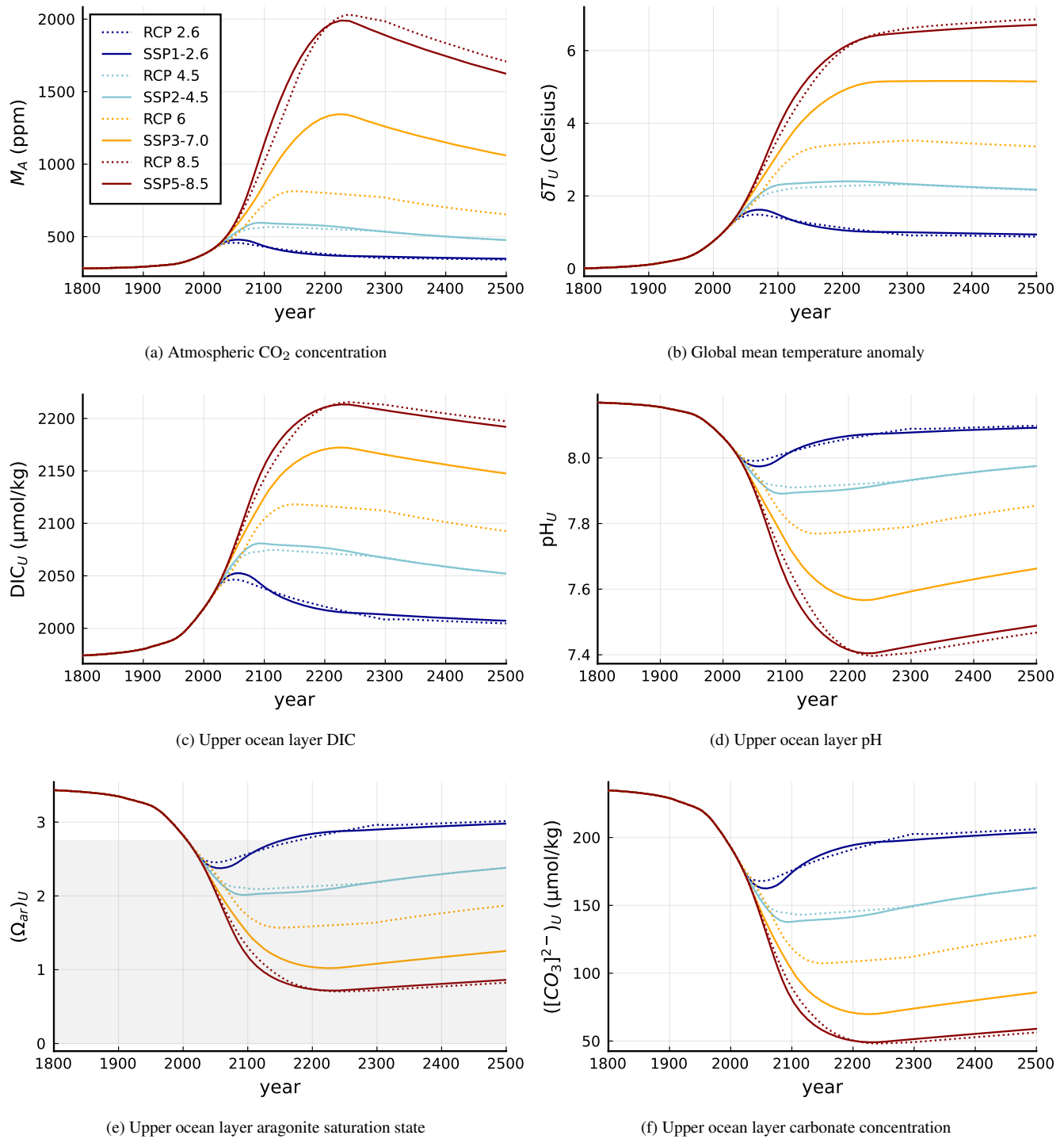
Figure 12. SURFER's output when forced by the extended RCPs and SSPs emission scenarios. From left to right, top to bottom: atmospheric CO 2 concentration, global mean temperature anomaly, Dissolved Inorganic Carbon in the upper layer, pH in the upper layer, aragonite saturation state in the upper layer and carbonate concentration in the upper layer.
