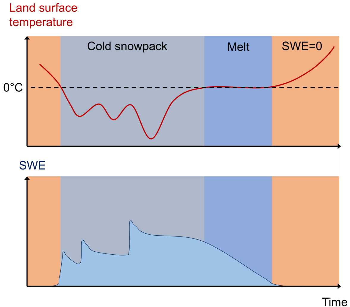
Figure 2: Schematic representation of the seasonal behavior of the LST.
