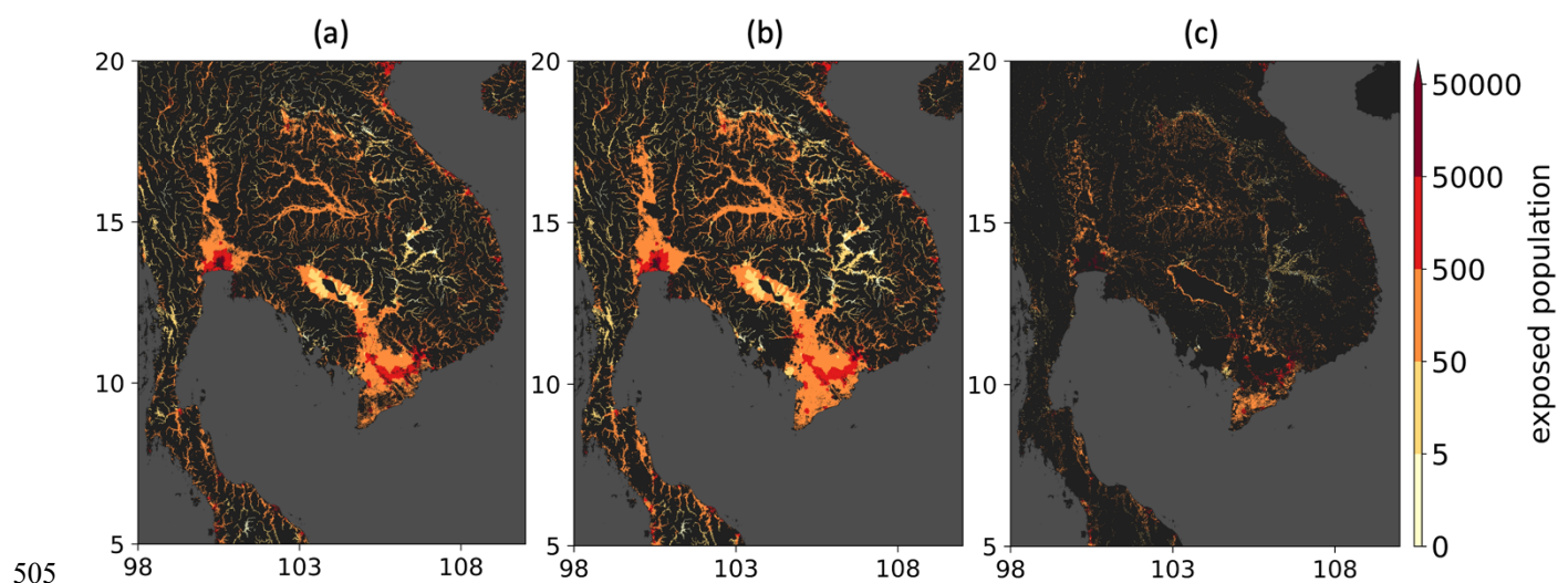
Figure 9: Affected population in the Chao Phraya River and Mekong River area based on the 100-year RP hazard map (obtained using IPSL-CM6A-LR). (a) Reference historical hazard map; (b) future-hazard map constructed using the lookup method; and (c) difference of (b)–(a), representing the population not currently affected by flooding that may be affected under the future climate.
