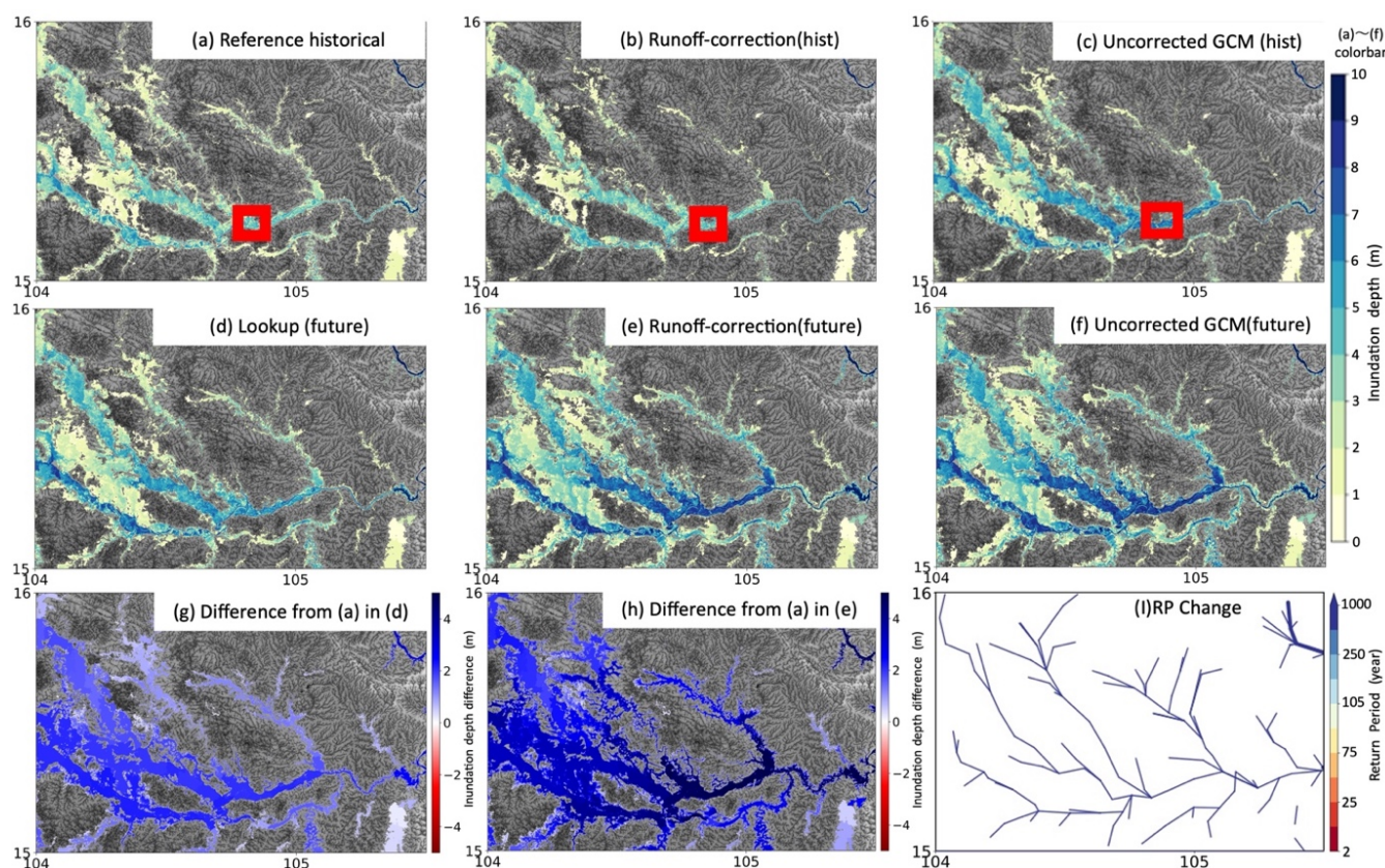
Figure 3: 100-year RP hazard map for the Chi-Mun River basin (using the IPSL-CM6A-LR CMIP6 GCM).
