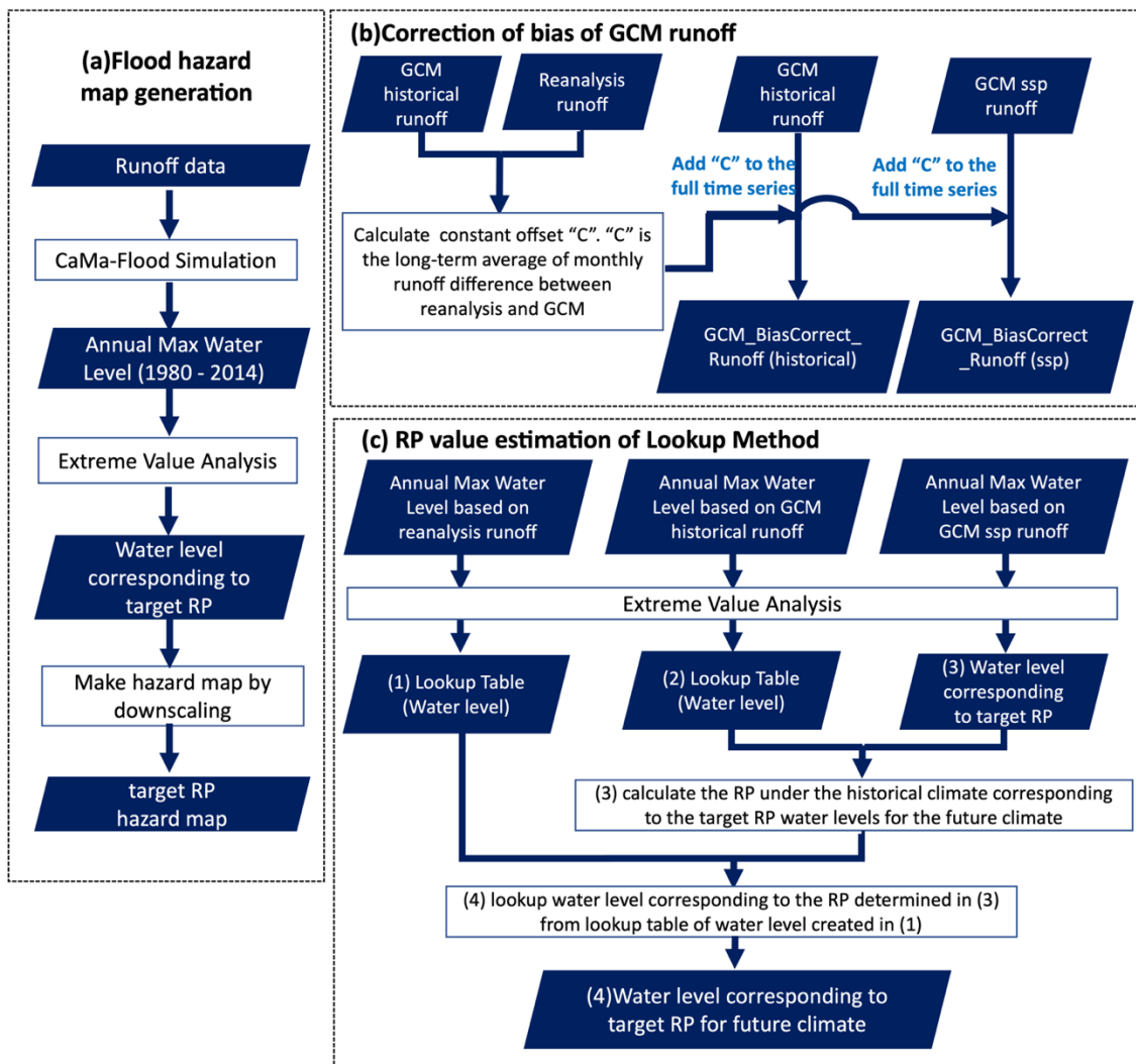
165 Figure 1: Simplified schematic diagrams of (a) flood-hazard map generation, (b) correction of bias of GCM runoff, and (c) RP value estimation via the lookup method.
