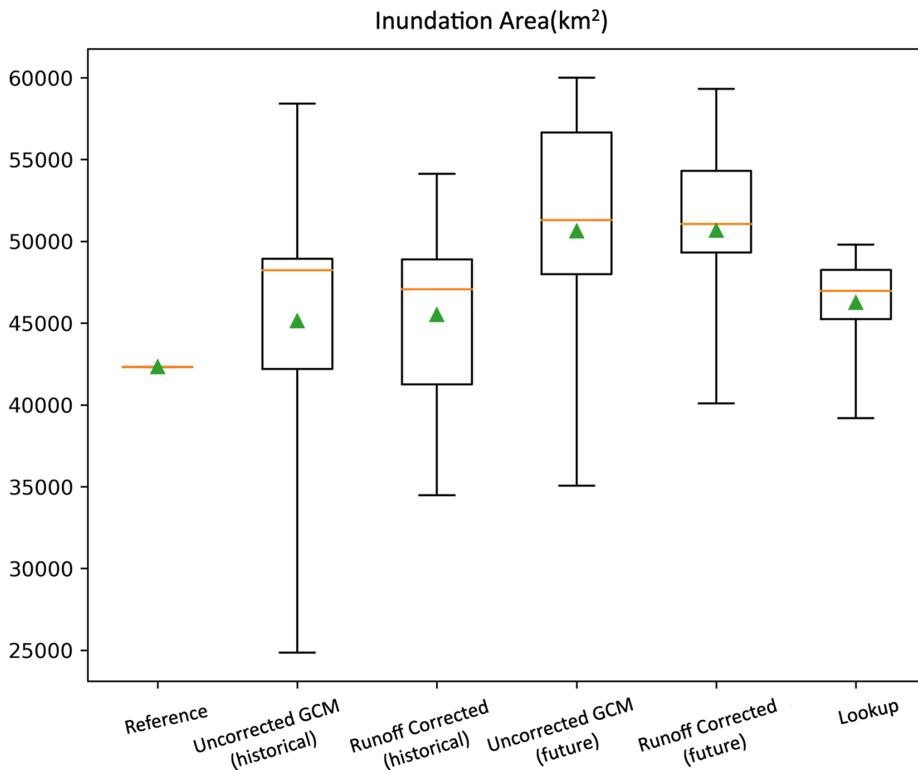
350 Figure 7: Box plot of inundated area (km 2 ) estimates near the Chao Phraya River obtained using the runoff-correction method and lookup method. Whiskers show minimum and maximum values, boxes show 25th and 75th percentile values, orange lines show the median (50th percentile) value and green triangles show the average value.
