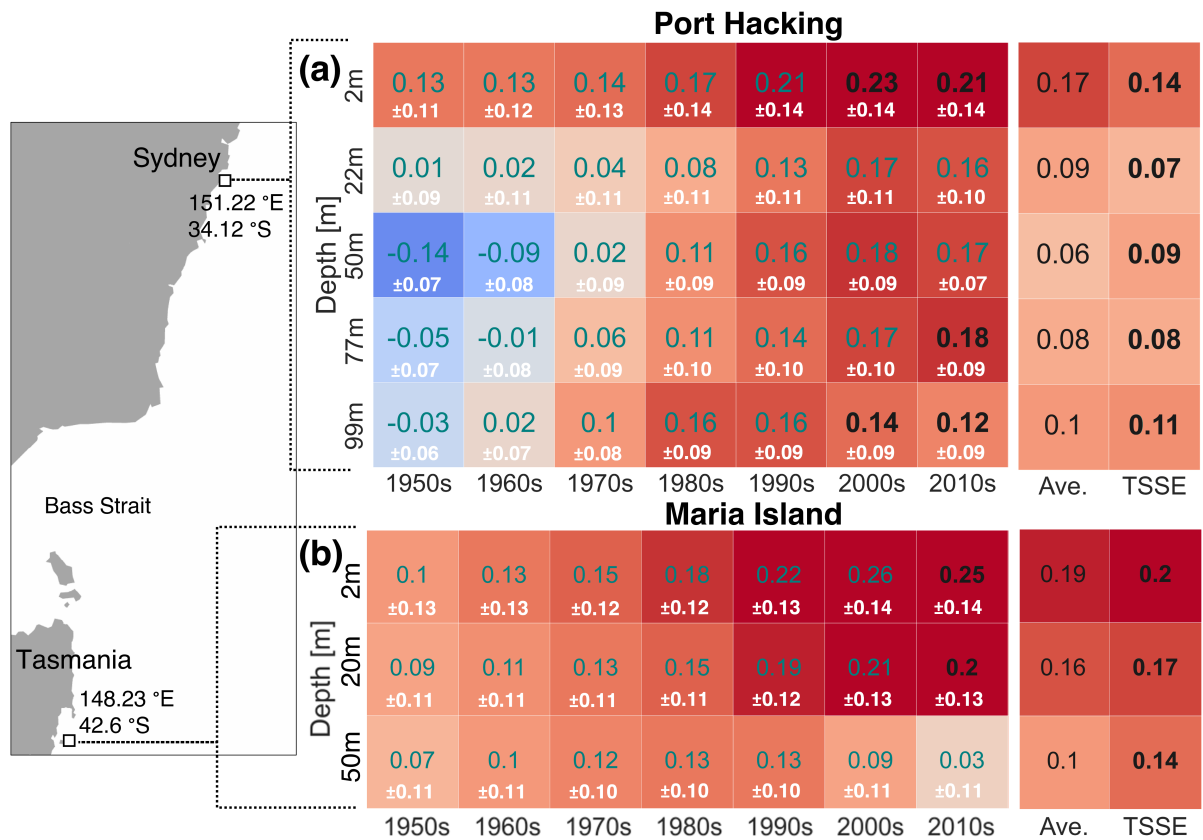
Figure 4. Temperature trends for multiple depths at (a) Port Hacking (NRSPHB) and (b) Maria Island (NRSMAI). Statistically significant (black bold text) and non-statistically significant statistically insignificant (gray grey text) average EEMD trend rates per decade ( ^{\circ}\text{C decade}^{-1} ), and the total time-average over all decades ('Ave.', black text) are shown. The uncertainty for each decade is listed beneath the average EEMD trend rates as white text. The statistically significant Theil-Sen Slope Estimator (TSSE) trend estimates ( ^{\circ}\text{C decade}^{-1} ) using data over the whole time period are also shown for each site. The locations of the sites are shown in the left panel. The total time-averaged EEMD estimates use both statistically significant and insignificant trend rates over the whole time period, and thus are taken as insignificant estimates. Decade trends are considered significant if 75 % or more of the trend during the selected decade are outside the 95 % confidence bounds.
