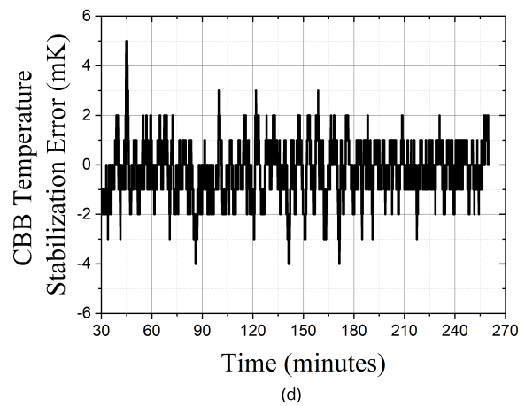
Figure 4. (a) Time evolution of the PT100 temperature for the HBB since the stabilisation controller is activated. (b) Difference between the HBB PT100 temperature and the target temperature ( 70^{\circ}\text{C} ) after the thermal stabilisation is reached. (c) Time evolution of the PT100 temperature for the CBB. (d) Difference between the CBB PT100 temperature and the target temperature ( 15^{\circ}\text{C} ), after the thermal stabilisation is reached.
