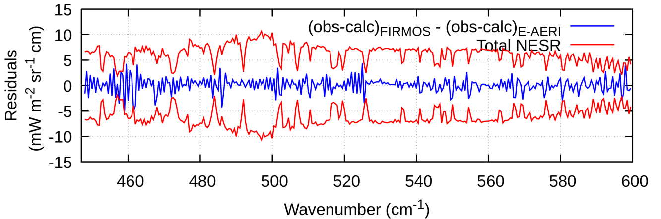
Figure 25. Differences of FIRMOS and E-AERI observed minus calculated residuals, R_{DIFF} (blue) as defined in Eq. 6, and quadrature sum of the NESR of the two instruments (red).
