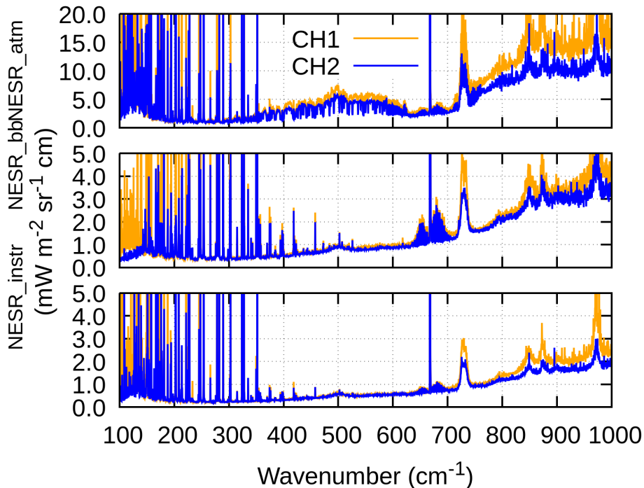
Figure 7. NESR of the calibrated spectra calculated from error propagation of Eq.3, in the case of a measurement cycle of N = 4 sky measurements and n = 2 for each calibration sources. NESR_atm (upper panel) is for the observation of the atmosphere in clear sky condition, NESR_bb (middle panel) is for the observation of a blackbody sources in laboratory, and NESR_instr (lower panel) is the instrumental component equal to \Delta S/F * \sqrt{(1/N)}
