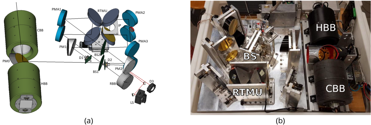
Figure 1. FIRMOS: (a) optical layout diagram, the blackbodies (HBB and CBB) are depicted in green, PM0 indicates the scene selection mirror. The roof-top mirrors unit (RTMU) is on the top right, IP is the internal pupil, in the centre BS1 and BS2 indicate the beam splitters. The whole optical path is folded on two levels using mirrors (PMA1, PMA2, PMA3, PM1, PM2). Also shown are the pyroelectric detectors (D1 and D2) the reference laser (LS) and its detector (D3), the reference (RBB) (b) picture of the inner structure of the instrument
