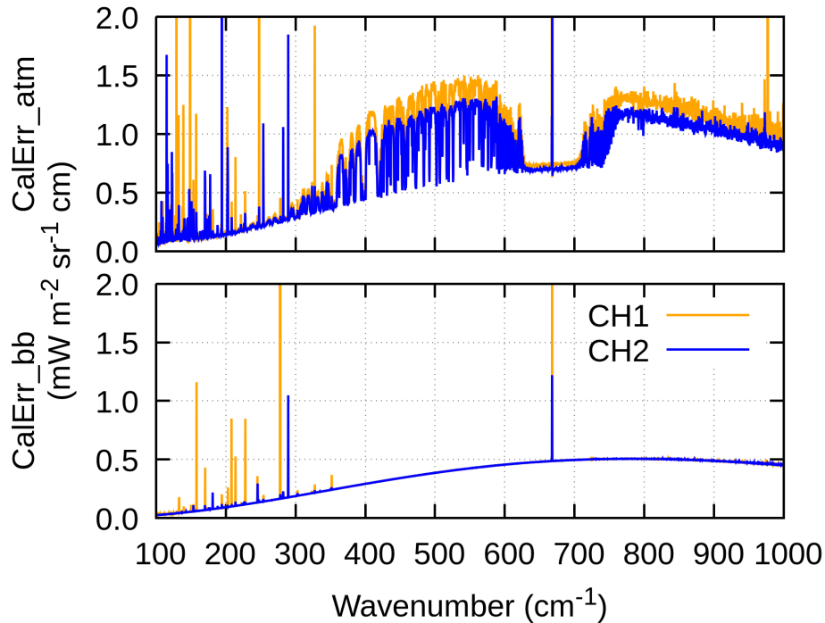
Figure 9. Calibration error calculated from a conservative estimation of 0.3 K uncertainty on the temperature measurement of each reference blackbody. CalErr_atm (upper panel) is for the observation of the atmosphere in clear sky condition, CalErr_bb (lower panel) is for the observation of a blackbody source in laboratory.
