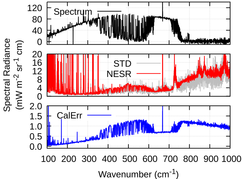
Figure 10. Calibrated spectrum (upper panel) and error estimates (NESR and STD middle, Calibration error lower panel) obtained from the weighted mean of the two output channels in a measurement cycle of four zenith observations in clear sky conditions on 25 January 2019 at 15:55 UTC.
