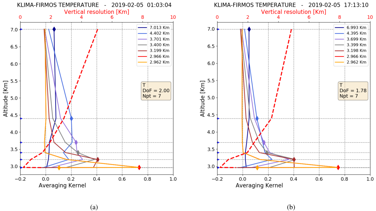
Figure 19. As in Figure 18 for the temperature profiles.
