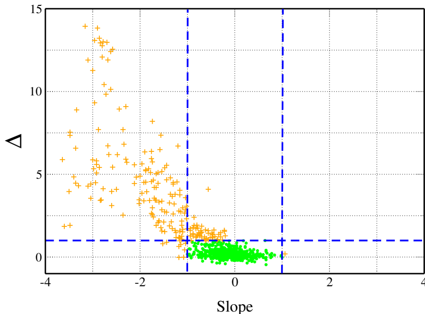
Figure 11. Plot of the \Delta ratio, as defined in Eq. 5, versus the normalised slope calculated using the 6 microwindows in the spectral range 786\text{-}961\text{ cm}^{-1} defined in the text. Blue dashed lines indicate the acceptance values and the green dots and orange crosses denote the spectra analysable and not analysable with KLIMA, respectively.
