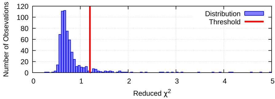
Figure 12. Distribution of the reduced \chi^2 using a bin width of 0.05. The red vertical line at 1.2 indicates the threshold corresponding to an evident minimum (close to zero cases) of the distribution.
