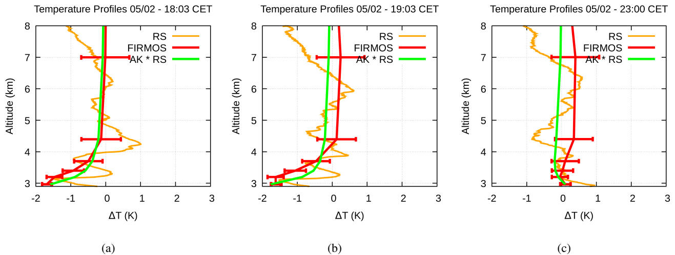
Figure 23. Comparison between the FIRMOS L2 temperature product (red curves, the error bars indicate the retrieval error) and radiosonde profiles (orange curves: raw data, the green curves are convolved with the FIRMOS AK). The profiles are shown as a difference with respect to the a-priori of the retrieval, for an effective interpretation. Each plot refers to a different radiosonde acquisition, the local time of the radiosonde launch is also reported.
