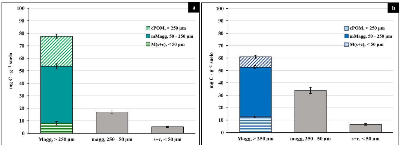
805 Figure 4. Distribution of organic C in stable aggregates and individual particles in soil under OPM (a) and CM (b) Magg: Macroaggregates; magg: microaggregates; mMagg: microaggregates within macroaggregates. s+c: silt+clay fraction; cPOM: coarse particulate organic matter >250 μm and sand particles. The error bars represent the standard error, which is the standard deviation divided by the square root of the sample size. All aggregate fractions are significantly different ( p < 0.05 ) between OPM and CM, with the exception of s+c and mMagg.
