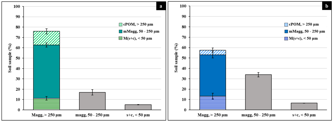
Figure 3. Size-distribution of stable aggregates and individual particles in the soil under OPM (a) and CM (b) Magg: Macroaggregates; magg: microaggregates; mMagg: microaggregates within macroaggregates. s+c: silt+clay fraction; cPOM: coarse particulate organic matter >250 μm and sand particles. The error bars represent the standard error, which is the standard deviation divided by the square root of the sample size. All aggregate fractions are significantly different ( p < 0.05 ) between OPM and CM, with the exception of mMagg.
