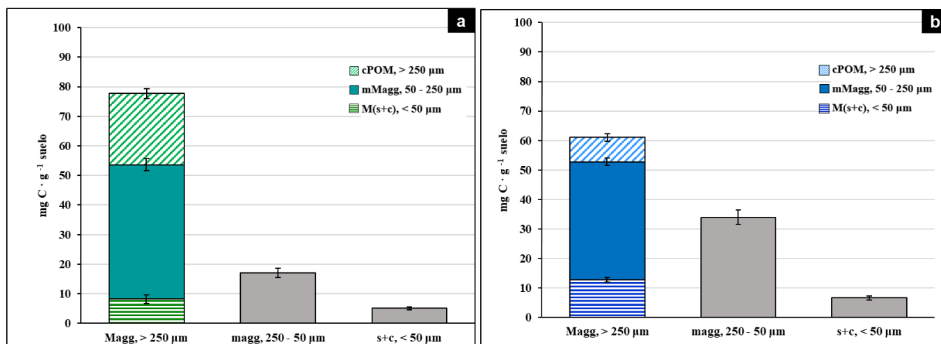
Figure 4. Distribution of organic C in stable aggregates and individual particles in soil under OPM (a) and CM (b) Magg: Macroaggregates; magg: microaggregates; mMagg: microaggregates within macroaggregates. s+c: silt+clay fraction; cPOM: coarse particulate organic matter >250 μm and sand particles. The error bars represent the standard error, which is the standard deviation divided by the square root of the sample size. All aggregate fractions are significantly different ( p < 0.05 ) between OPM and CM, with the exception of s+c and mMagg.
