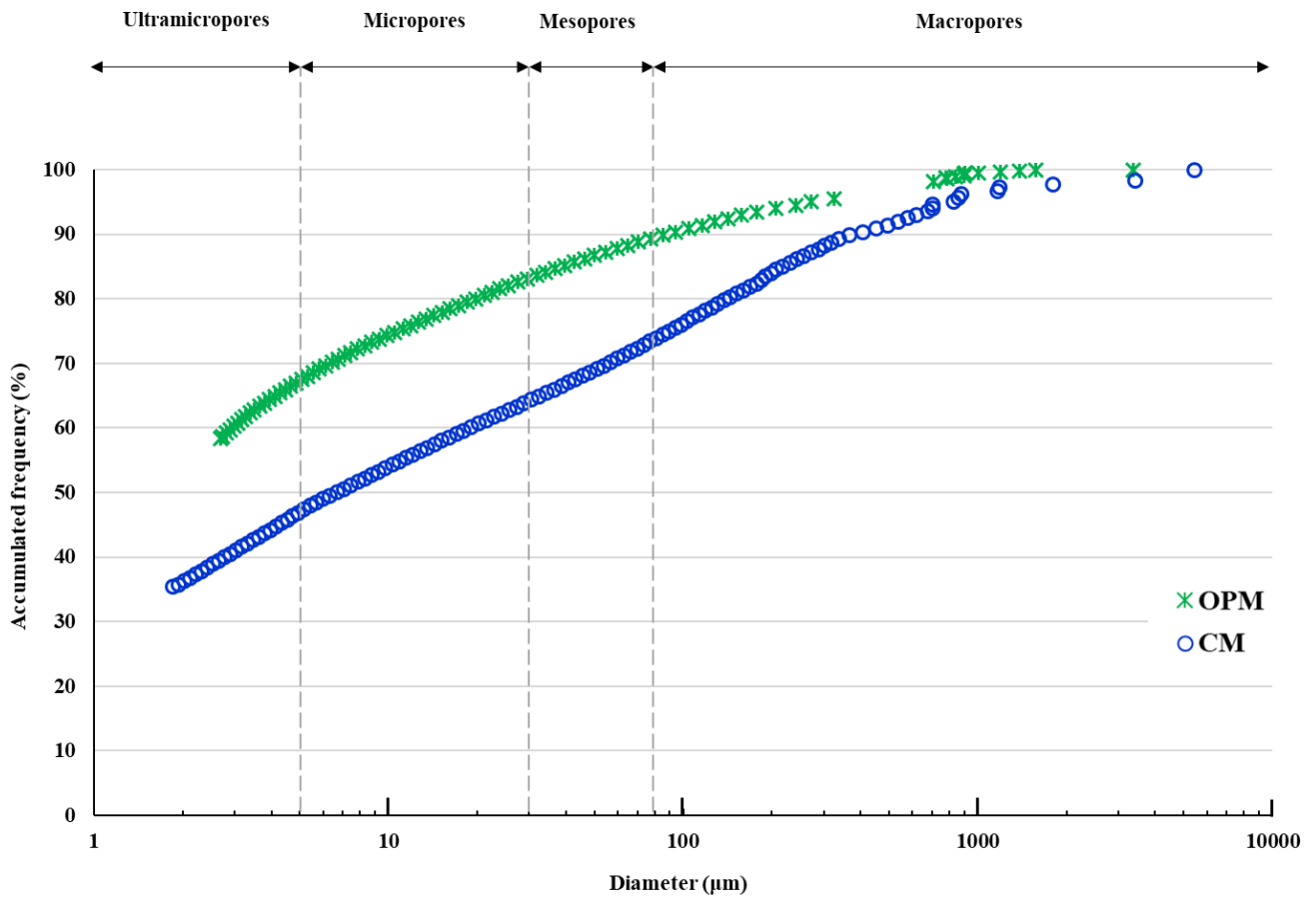
Figure 3. Accumulated frequency of pore sizes (mean of three replicates) of the soil under the two studied treatments (OPM and CM), and pore size classification (Weil and Brady, 2017). Note: X-axis in logarithmic scale.
