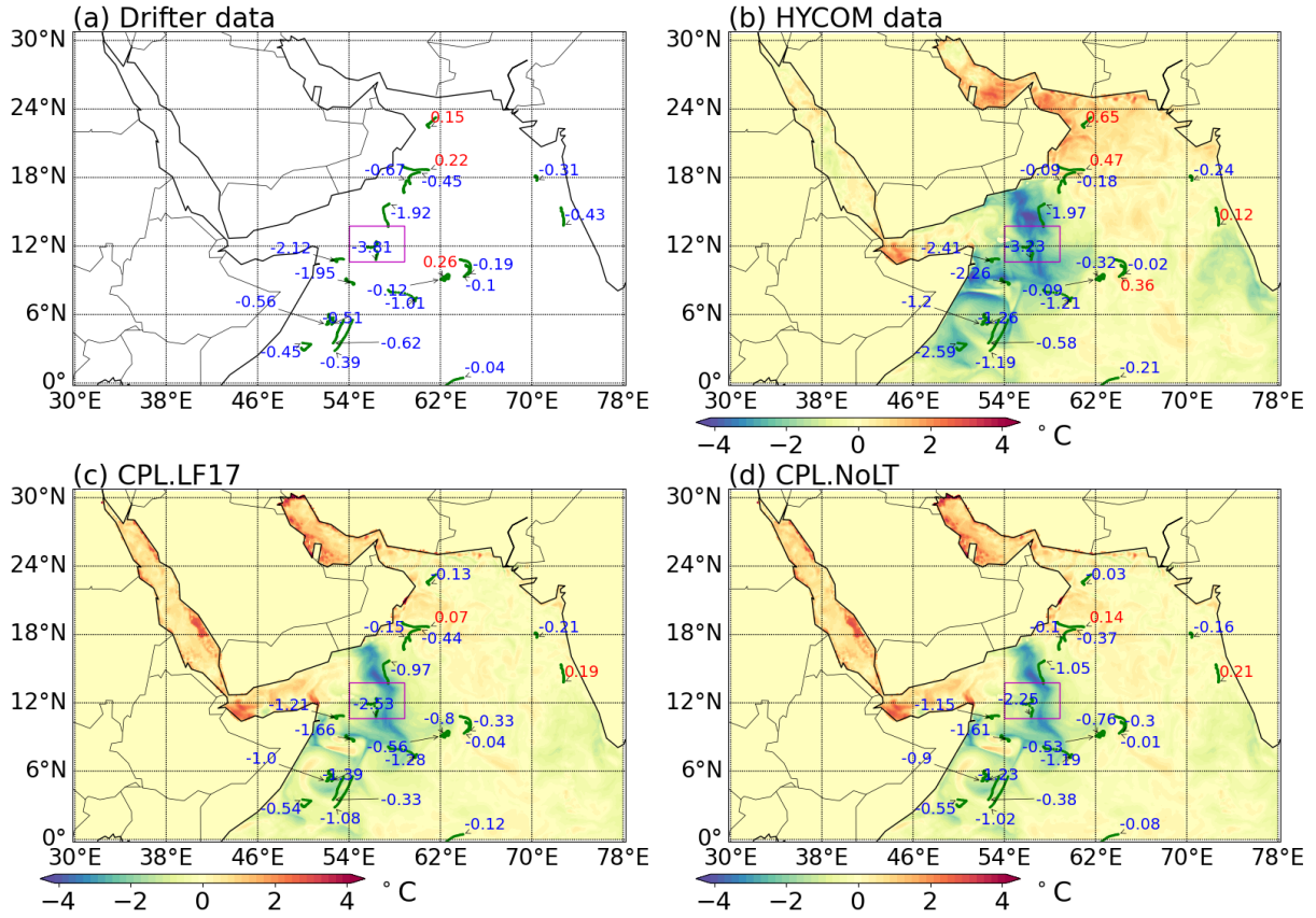
Figure 8. Evolution of the SST during the tropical cyclone event in comparison with drifter data. Panel (a) shows the SST changes during the event from drifter data; Panels (b-d) show the ensemble averaged SST changes from HYCOM, CPL.LF17, and CPL.NoLT, respectively. The red numbers indicate SST warming during the event; the blue numbers indicate SST cooling during the event.
