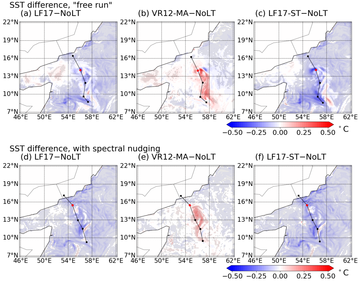
Figure 9. The snapshots of the ensemble averaged SST difference. Panels (a-c) show the SST difference between the simulations with Langmuir turbulence (CPL.LF17, CPL.VR12-MA, and CPL.LF17-ST) and without Langmuir turbulence (CPL.NoLT). Panels (d-f) show the same differences in the simulations with spectral nudging. The markers indicate the regions where the SST difference is significant ( P < 0.05 ).
