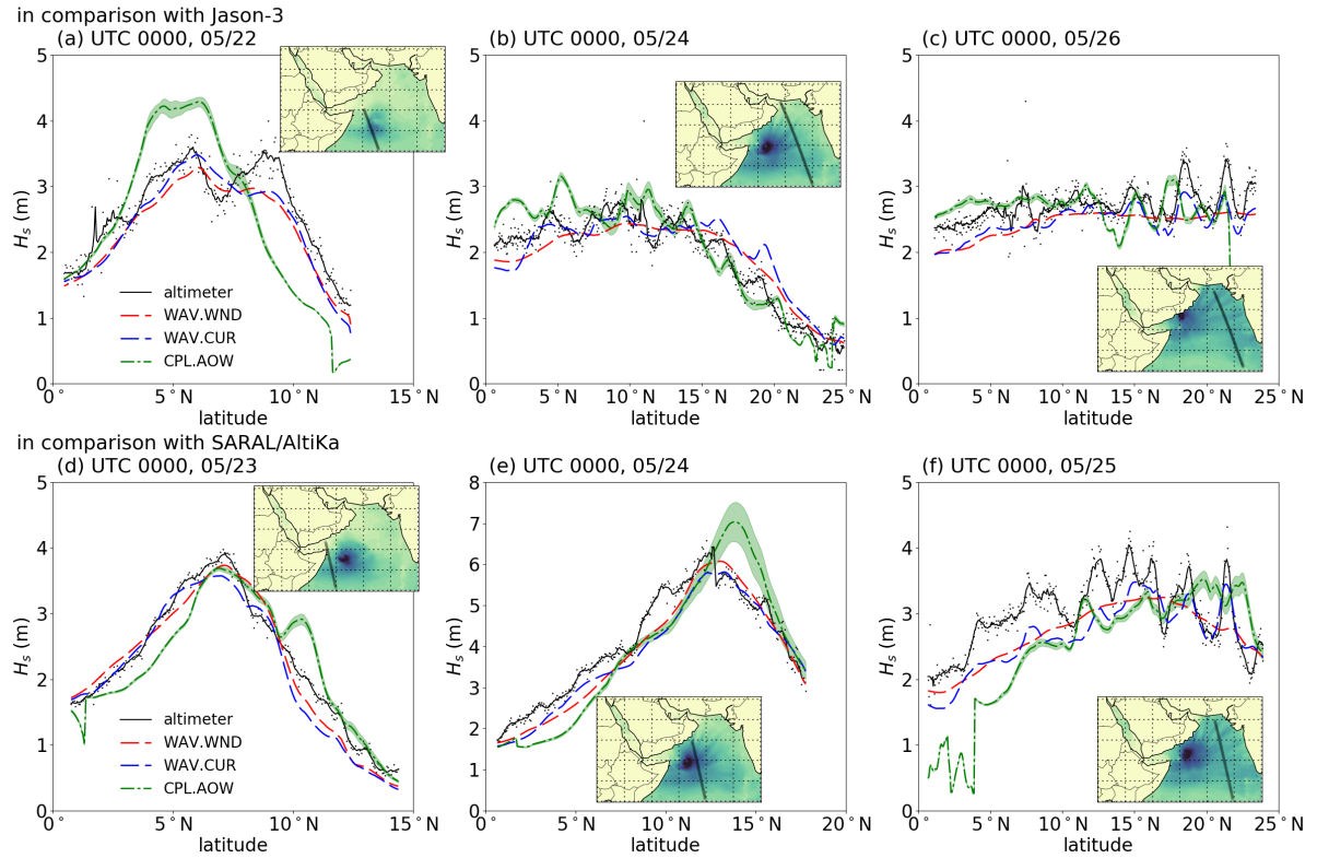
Figure A7. The ensemble averaged significant wave height in comparison with the altimeter data. Panels (a-c) show the comparison with Jason-3 data; Panels (d-f) show the comparison with SARAL data. The simulation results from Sun et al. (2022) are also presented. The shaded areas indicate the standard deviation of wave height in the ensemble simulations.
