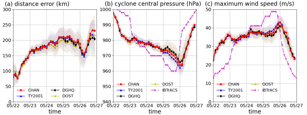
Figure A3. The characteristics of cyclone Mekunu obtained from the coupled simulations using different options to parameterize surface roughness. The solid lines indicate the ensemble averaged simulation results; the shaded areas indicate the standard deviation of the results. Panel (a) shows the distance errors in comparison with IBTrACS data; Panel (b) shows the cyclone central pressure; Panel (c) shows the maximum wind speed.
