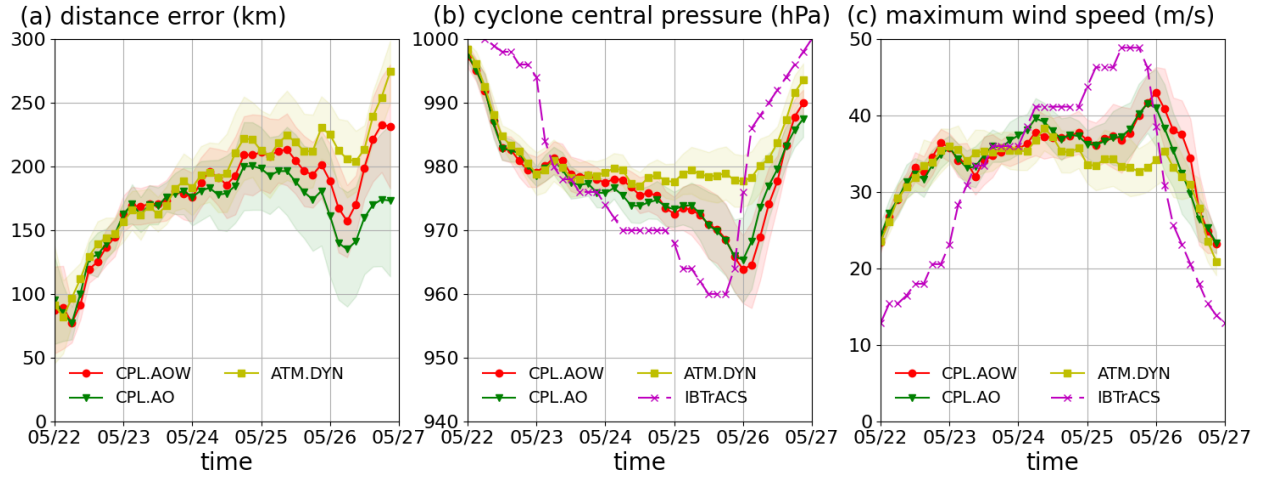
Figure 3. The characteristics of cyclone Mekunu obtained from the simulations plotted as functions of time. The solid lines indicate the ensemble averaged simulation results; the shaded areas indicate the standard deviation of the results. Panel (a) shows the distance errors in comparison with IBTrACS data; Panel (b) shows the cyclone central pressure; Panel (c) shows the maximum wind speed. The simulations start on May 20, but the results are not presented before the pressure starts to drop on May 22.
