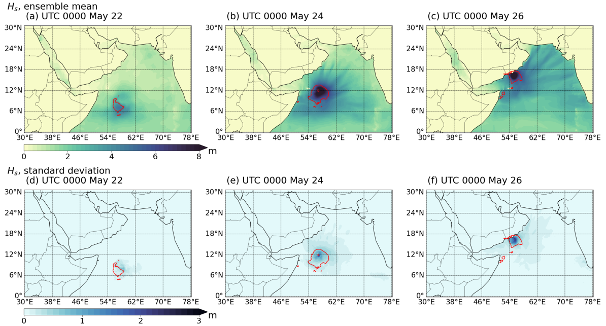
Figure 7. Snapshots of the significant wave height H_s at 00 UTC May 22 24, and 26, 2018. Panel (a-c) show the ensemble averaged H_s obtained from CPL.AOW; Panel (d-f) show the standard deviation of H_s of the ensembles from CPL.AOW. The 15 m/s contour of wind speed is used to highlight the location of the tropical cyclone.
