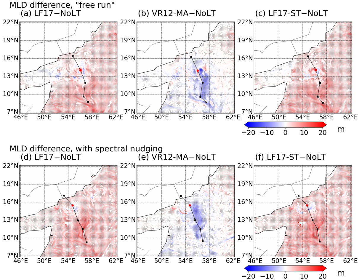
Figure 10. The snapshots of the ensemble averaged MLD difference. Panels (a-c) show the MLD difference between the simulations with Langmuir turbulence (CPL.LF17, CPL.VR12-MA, and CPL.LF17-ST) and without Langmuir turbulence (CPL.NoLT). Panels (d-f) show the same differences in the simulations with spectral nudging. The markers indicate the regions where the MLD difference is significant ( P < 0.05 ).
