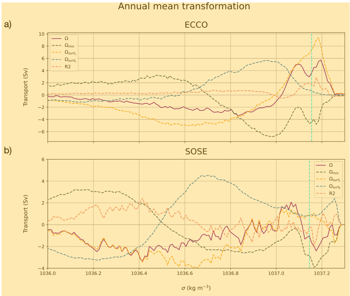
Figure 6. (a) Transformation term, \Omega (purple solid line), broken down into its sources of transformation: surface salt flux (orange dashed line); surface heat flux (blue dashed line); and mixing (slate grey dashed line). Residual due to numerical mixing is the pink dashed line in ECCO (a) and SOSE (b). The vertical dashed line demarcates the boundary of bottom water in each model ( 1037.155 \text{ kg m}^{-3} for ECCO, 1037.145 for SOSE, and 1037.175 \text{ kg m}^{-3} for SODA).
