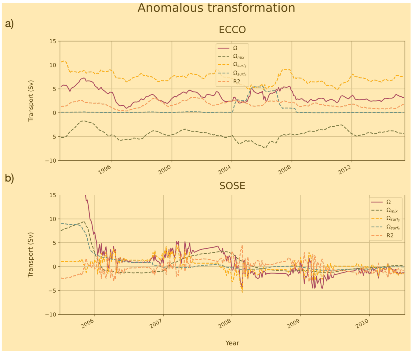
Figure 11. Anomalous transformation term, \Omega (purple solid line), broken down into its sources of transformation: surface salt flux (orange dashed line); surface heat flux (blue dashed line); and mixing (slate grey dashed line). R2 is the pink dashed line.
