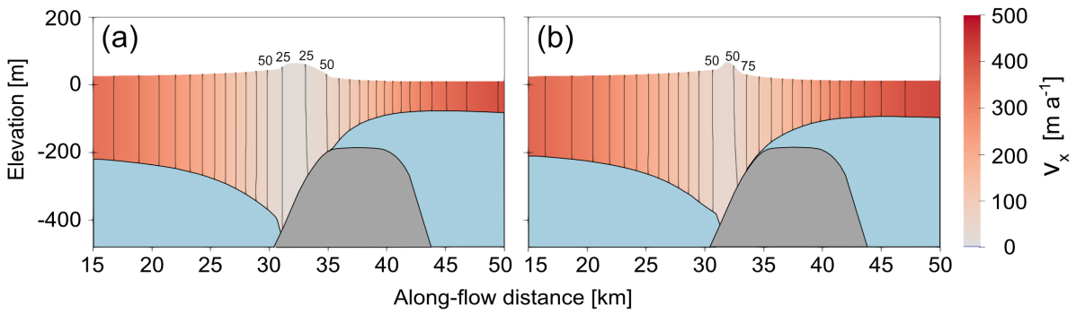
Figure 12. An along-flow cross-section of the ice rumple at t = 8000 years in the case of (a) the low basal friction and (b) the high intermediate basal friction. The contours show lines of equal velocity in the x -direction and are spaced 25 \text{ m a}^{-1} apart.
