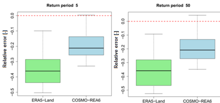
305 Figure 5: Comparison of the selected precipitation characteristics between ERA5-Land and COSMO-REA6 for rainfall intensities \geq 1.0 mm.
