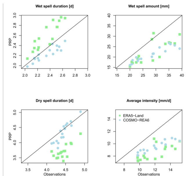
305 Figure 5: Comparison of the selected precipitation characteristics between ERA5-Land and COSMO-REA6 for rainfall intensities \geq 1.0 mm.
