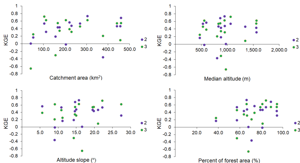
Figure 9: KGE scores against catchment characteristics for configurations 2 and 3 (Table 3).
