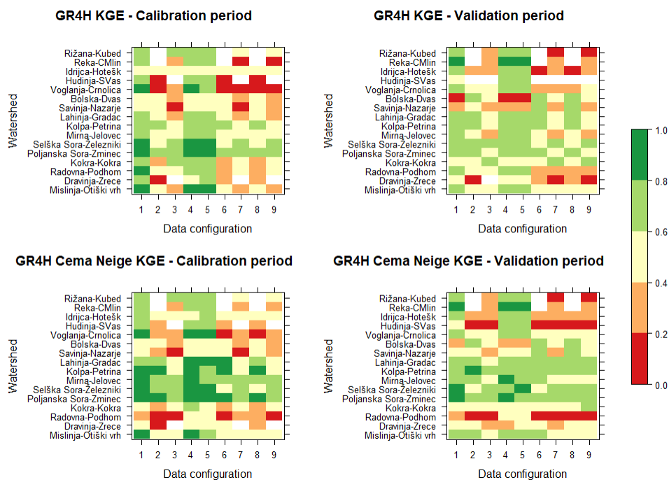
Figure 8: KGE scores for rainfall-runoff simulations per configuration for each catchment (initial model variable calibration). KGE values are distributed in five classes. White cells indicate negative values.
