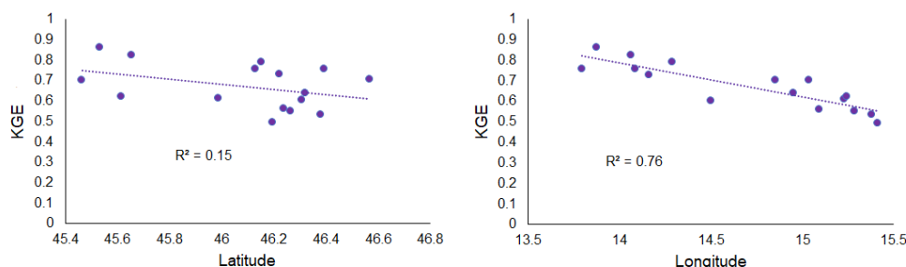
Figure 12: KGE scores (configuration 2 – GR4H – Calibration period), relative to longitude and latitude.
