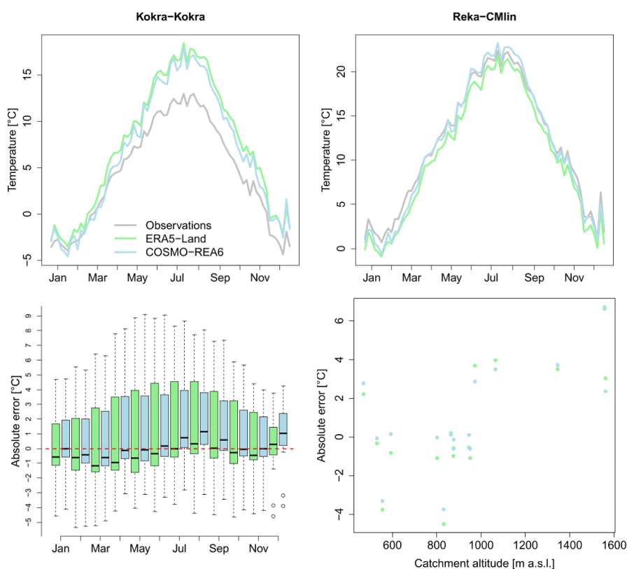
Figure 7: Top left and right: Median of daily temperature value smoothed via moving window of 5 days length for two selected catchments. Bottom left: Box plots of median monthly values for all considered catchments. Bottom right: Mean of monthly absolute error medians in dependence of catchment altitude.
