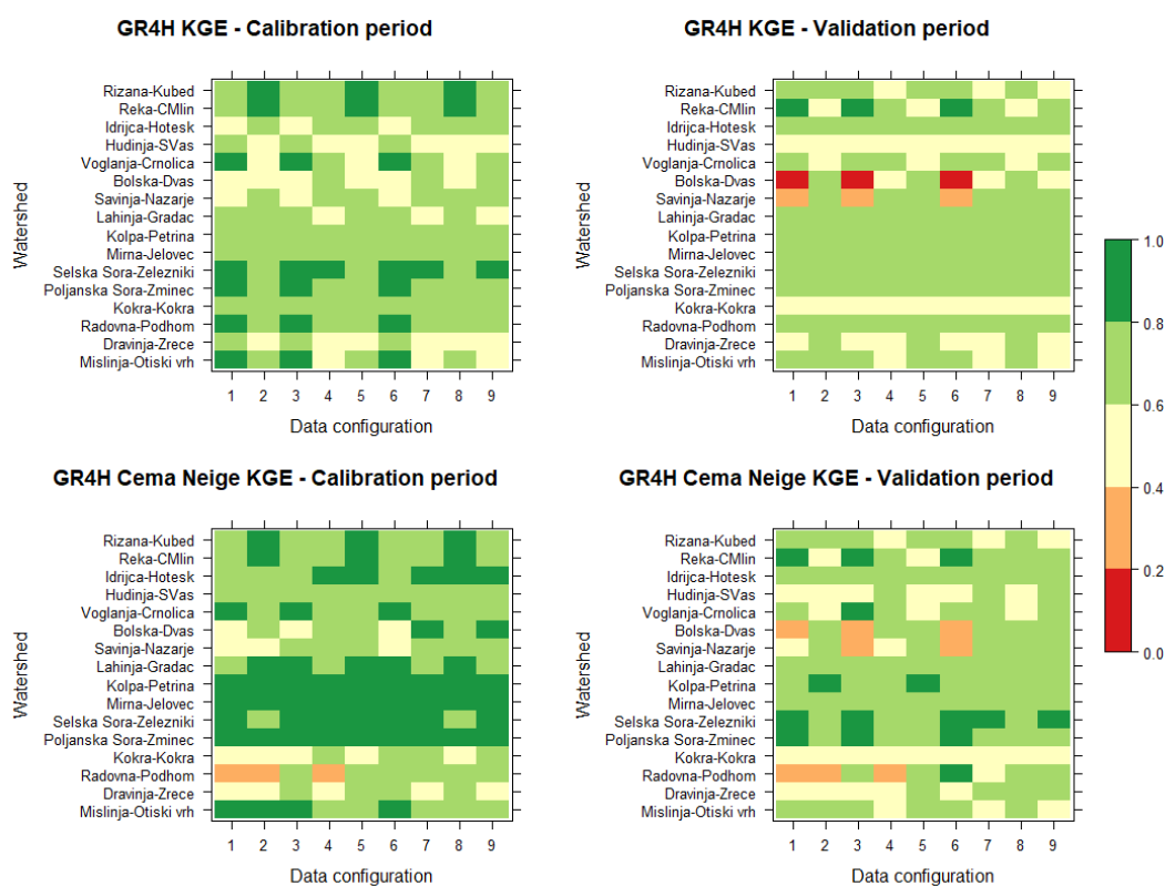
415 Figure 11: KGE scores for rainfall-runoff simulations per configuration for each catchment (sequential model variable calibration). KGE values are distributed in five classes.
