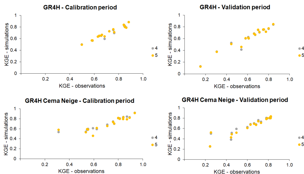
Figure 10: KGE values of reanalysis temperature against observed temperature for configurations 4 and 5.
