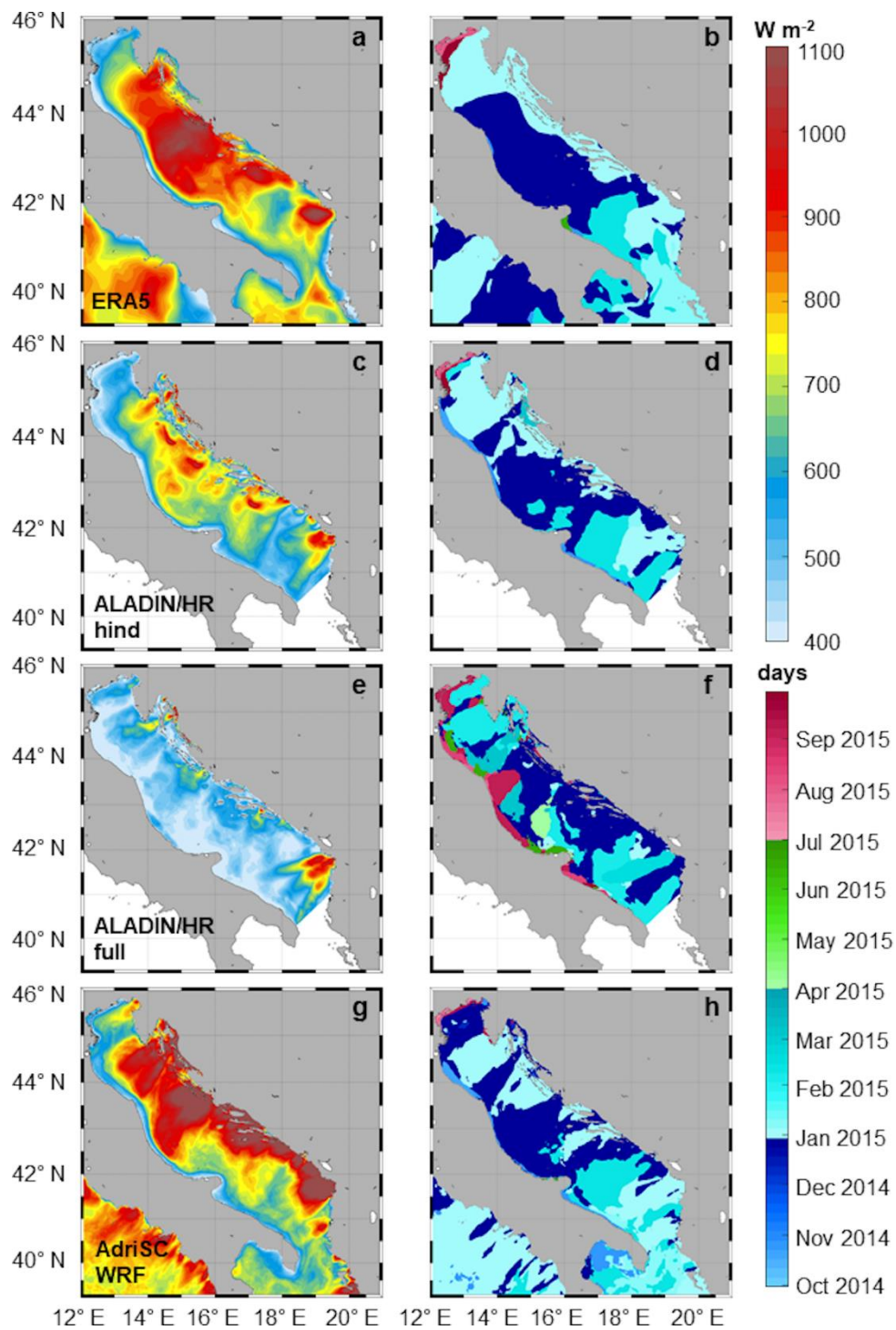
965 Figure 4: Spatial distribution of maximum upward turbulent heat fluxes and their corresponding timing for (a, b) ERA5, (c, d) ALADIN/HR-hind, (e, f) ALADIN/HR-full and (g, h) AdriSC-WRF.
