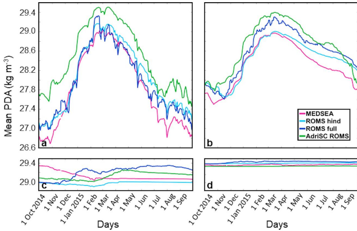
975 Figure 7: Time series of daily bottom PDAs averaged over four subdomains: (a) northern Adriatic, (b) Kvarner Bay, (c) Jabuka Pit and (d) deep Adriatic for the 2014-2015 period and four simulations.
