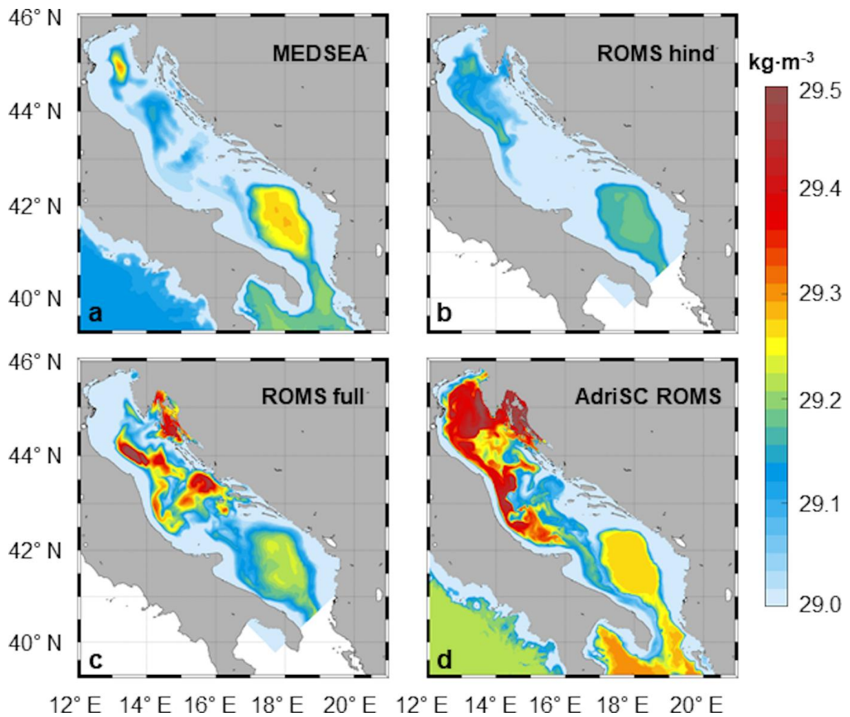
985 Figure 10: Spatial distribution of bottom PDAs on 1 April 2015 for (a) MEDSEA, (b) ROMS-hind, (c) ROMS-full and (d) AdriSC-ROMS simulations.
