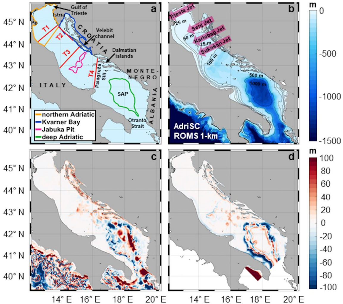
Figure 1. (a) Models domain with geographical locations, transects and subdomains, (b) AdriSC-ROMS 1 km bathymetry, (c) difference between AdriSC-ROMS 1 km and MEDSEA 1 km bathymetry, (d) difference between AdriSC-ROMS 1 km and ROMS 1 km bathymetry.
