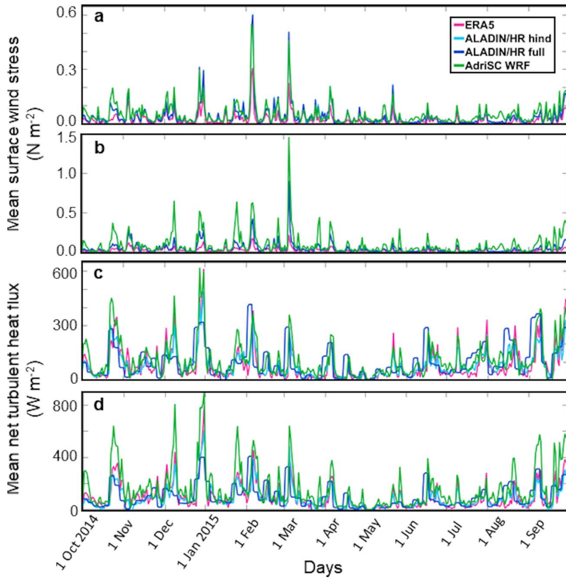
970 Figure 6: Time series of daily wind stresses and upward turbulent heat fluxes averaged over two subdomains: (a, c) northern Adriatic and (b, d) Kvarner Bay for the 2014-2015 period and four simulations.
