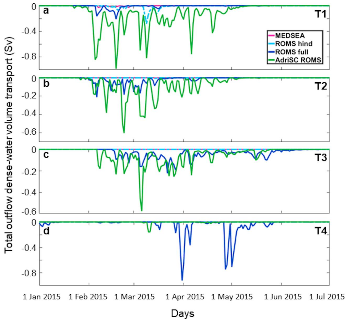
Figure 13: Daily volume transport rates of dense water outflow with PDA higher than 29.2 \text{ kg m}^{-3} integrated over transect (a) 995 T1, (b) T2, (c) T3 and (d) T4.
