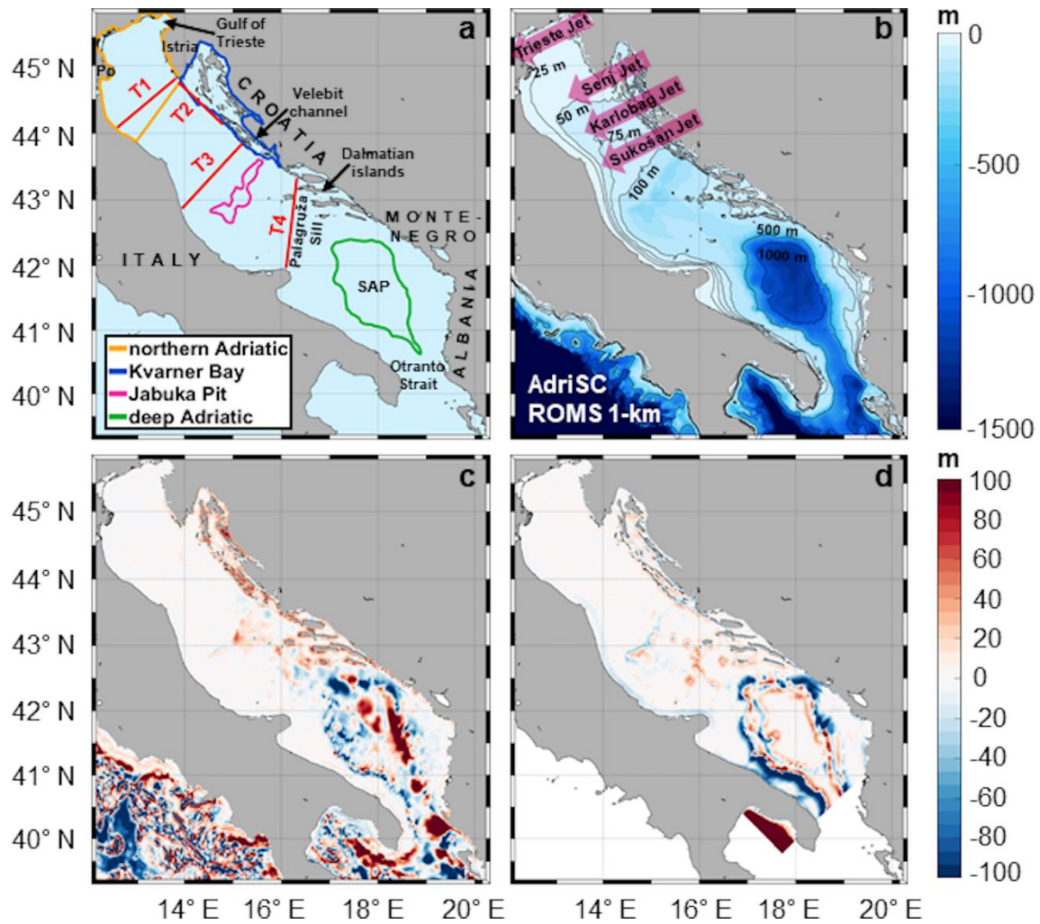
950 Figure 1. (a) Models domain with geographical locations, transects and subdomains, (b) AdriSC-ROMS 1 km depths, (c) difference between AdriSC-ROMS 1 km and MEDSEA 1 km bathymetry, (d) difference between AdriSC-ROMS 1 km and ROMS 1 km bathymetry.
