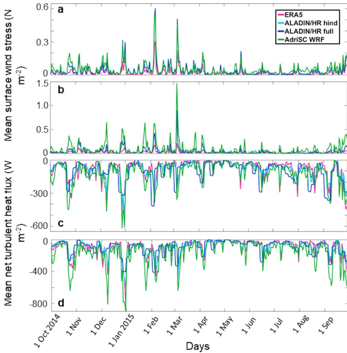
Figure 6: Time series of daily turbulent fluxes and wind stresses averaged over two subdomains: (a, c) northern Adriatic and (b, d) Kvarner Bay for the 2014-2015 period and four simulations.
