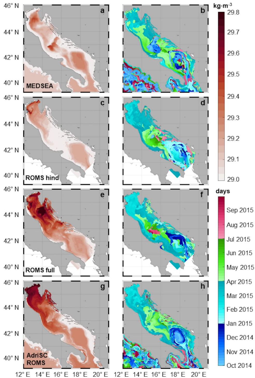
965 Figure 5. Spatial distribution of maximum bottom PDAs and their corresponding timing for (a, b) MEDSEA, (c, d) ROMS-hind, (e, f) ROMS-full and (g, h) AdriSC-ROMS.
