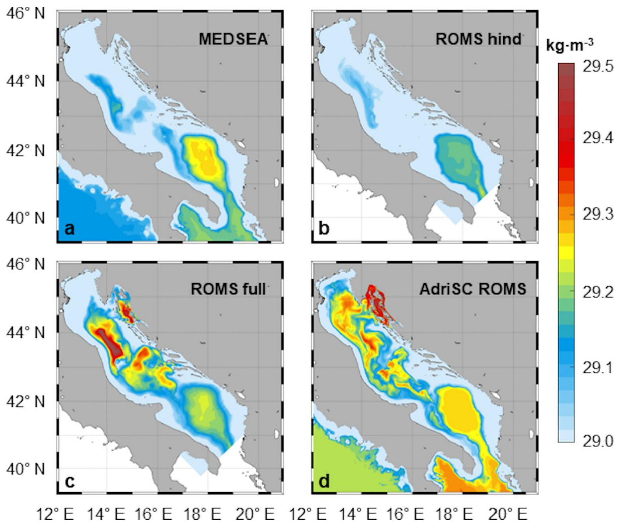
985 Figure 11: Spatial distribution of bottom PDAs on 1 May 2015 for (a) MEDSEA, (b) ROMS-hind, (c) ROMS-full and (d) AdriSC-ROMS simulations.
