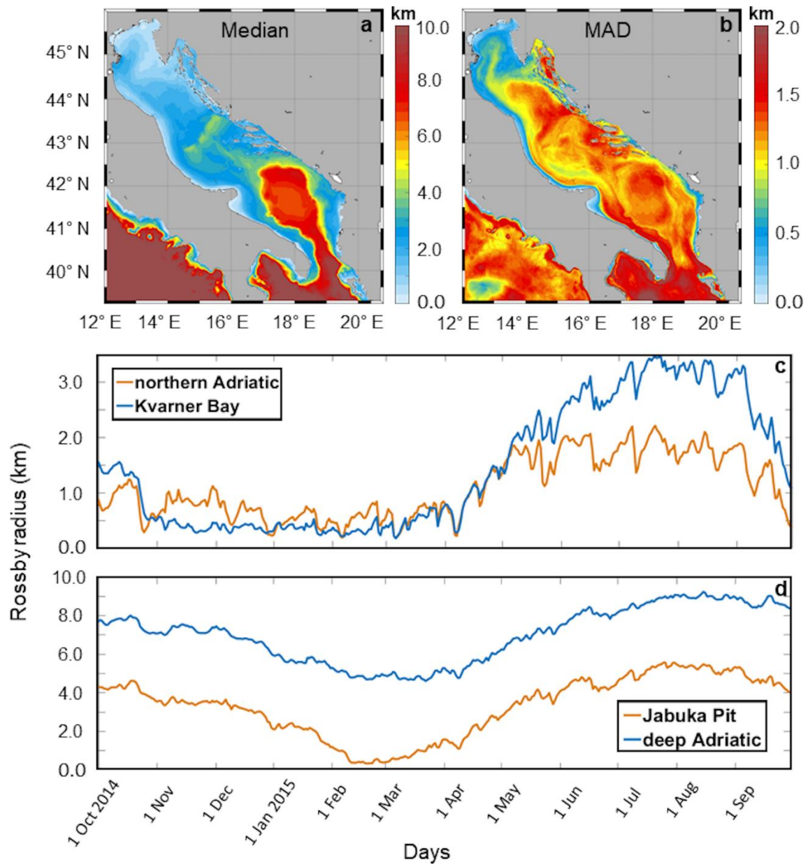
995 Figure 14: Median and MAD of the first baroclinic Rossby radius of deformation for the AdriSC-ROMS domain (a, b) and time series of the Rossby radius for the northern Adriatic and Kvarner Bay (c) as well as for the Jabuka Pit and deep Adriatic subdomain (d).
