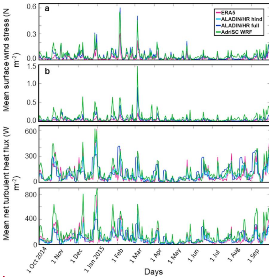
Figure 6: Time series of daily wind stresses and upward turbulent heat fluxes averaged over two subdomains: (a, c) northern Adriatic and (b, d) Kvarner Bay for the 2014-2015 period and four simulations.
