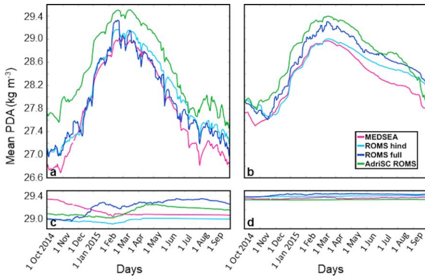
Figure 7: Time series of daily bottom PDAs averaged over four subdomains: (a) northern Adriatic, (b) Kvarner Bay, (c) Jabuka Pit and (d) deep Adriatic for the 2014-2015 period and four simulations.
