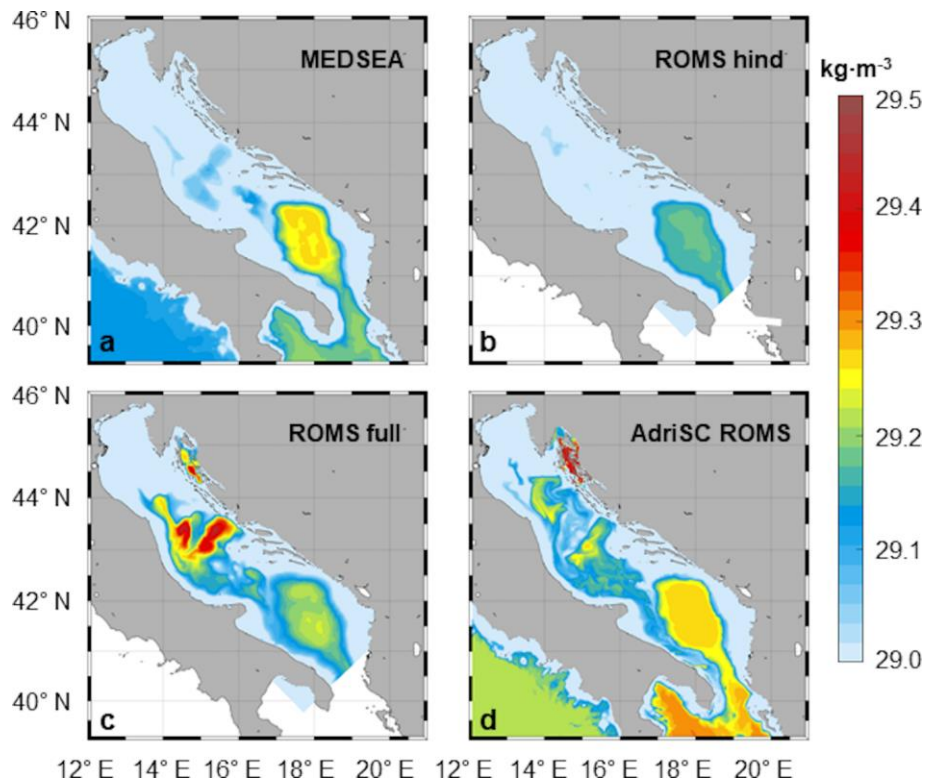
1205 Figure 12: Spatial distribution of bottom PDAs on 1 June 2015 for (a) MEDSEA, (b) ROMS-hind, (c) ROMS-full and (d) AdriSC-ROMS simulations.
