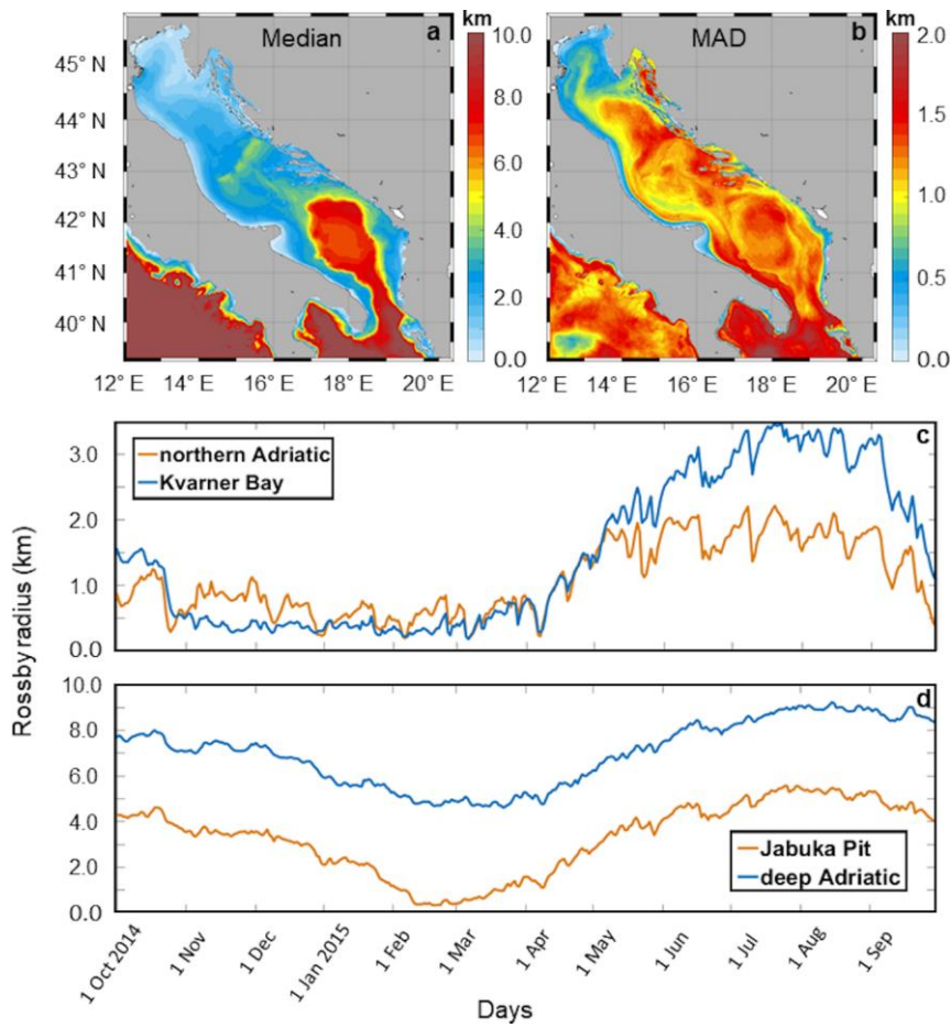
Figure 14: Median and MAD of the first baroclinic Rossby radius of deformation for the AdriSC-ROMS domain (a, b) and time series of the Rossby radius for the northern Adriatic and Kvarner Bay (c) as well as for the Jabuka Pit and deep Adriatic subdomain (d).
