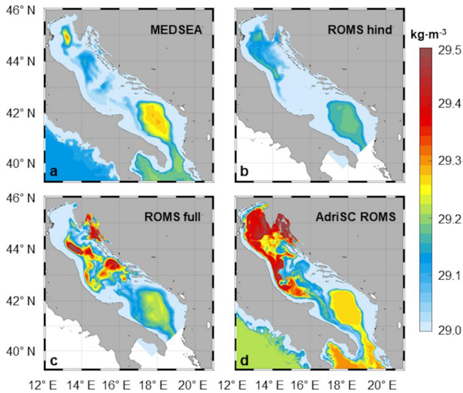
1200 Figure 10: Spatial distribution of bottom PDAs on 1 April 2015 for (a) MEDSEA, (b) ROMS-hind, (c) ROMS-full and (d) AdriSC-ROMS simulations.
