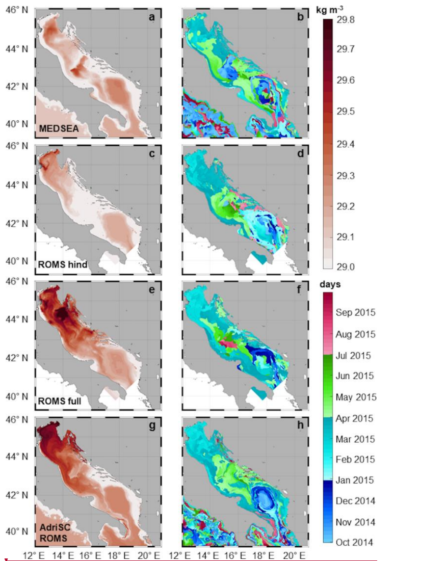
Figure 5. Spatial distribution of maximum bottom PDAs and their corresponding timing for (a, b) MEDSEA, (c, d) ROMS-hind, (e, f) ROMS-full and (g, h) AdriSC-ROMS.
