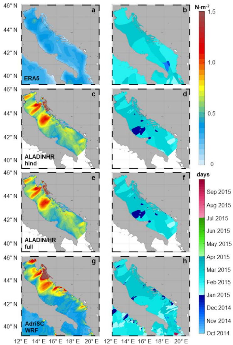
1490 Figure 3: Spatial distribution of maximum surface wind stresses and their corresponding timing for (a, b) ERA5, (c, d) ALADIN/HR-hind, (e, f) ALADIN/HR-full and (g, h) AdriSC-WRF.
