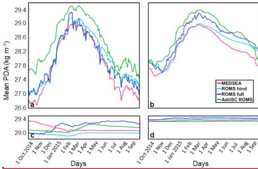
1505 Figure 7: Time series of daily bottom PDAs averaged over four subdomains: (a) northern Adriatic, (b) Kvarner Bay, (c) Jabuka Pit and (d) deep Adriatic for the 2014-2015 period and four simulations.
