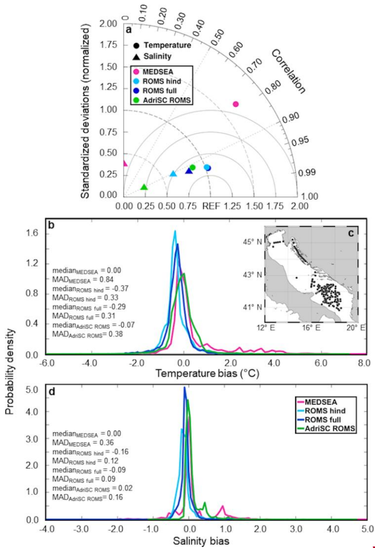
1480 Figure 2: Comparison of the results of the four simulations against CTD observations in the form of (a) a Taylor diagram, (b) probability density functions of the biases between the model results and in situ (b) temperature and (d) salinity observations as well as (c) a map with the locations of CTD observations (black dots).
