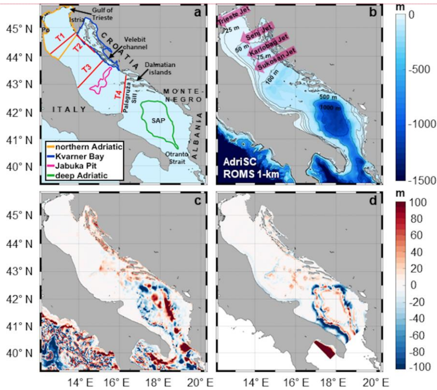
1475 Figure 1. (a) Models domain with geographical locations, transects and subdomains, (b) AdriSC-ROMS 1 km depths, (c) difference between AdriSC-ROMS 1 km and MEDSEA 1 km bathymetry, (d) difference between AdriSC-ROMS 1 km and ROMS 1 km bathymetry.
