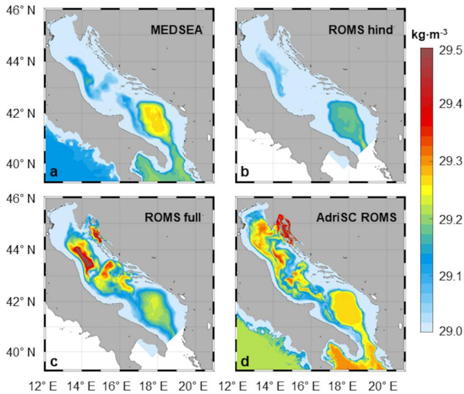
1520 Figure 11: Spatial distribution of bottom PDAs on 1 May 2015 for (a) MEDSEA, (b) ROMS-hind, (c) ROMS-full and (d) AdriSC-ROMS simulations.
