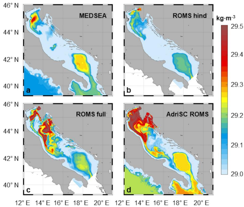
1515 Figure 9: Spatial distribution of bottom PDAs on 1 March 2015 for (a) MEDSEA, (b) ROMS-hind, (c) ROMS-full and (d) AdriSC-ROMS simulations.
