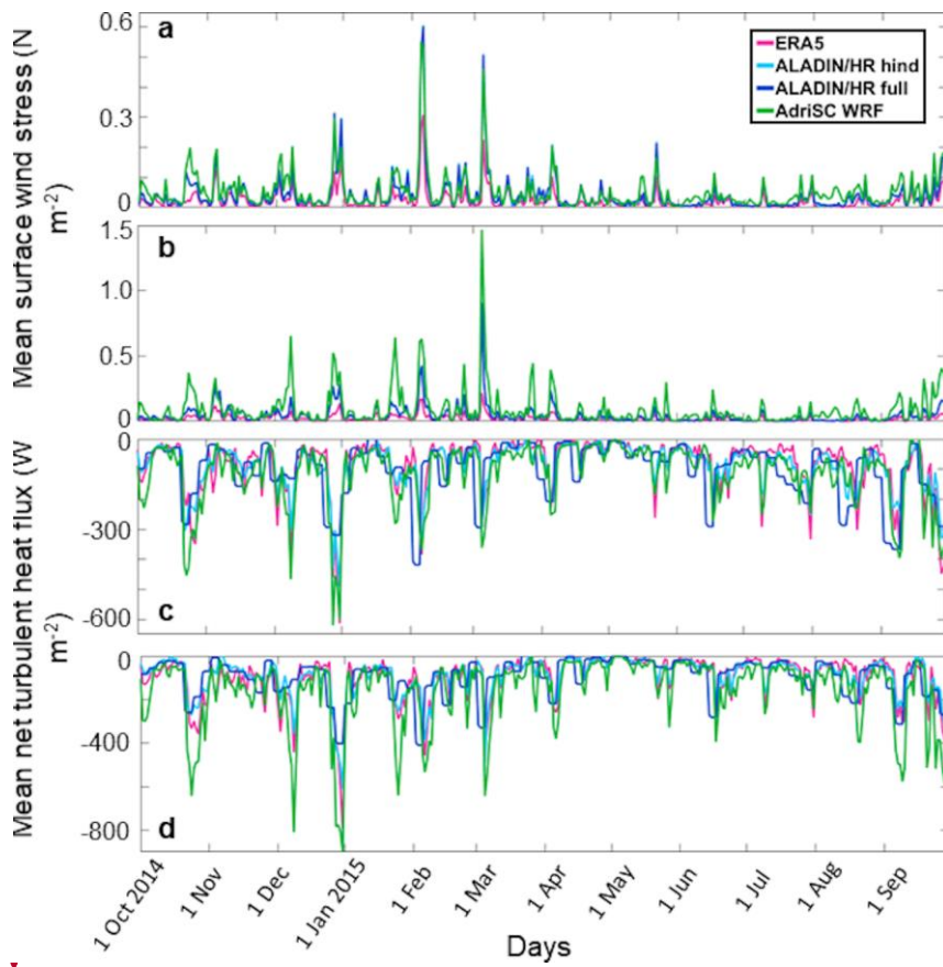
1500 Figure 6: Time series of daily turbulent fluxes and wind stresses averaged over two subdomains: (a, c) northern Adriatic and (b, d) Kvarner Bay for the 2014-2015 period and four simulations.
