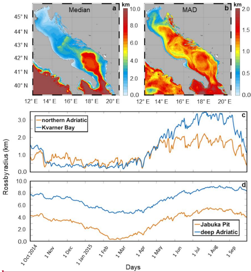
530 Figure 14: Median and MAD of the first baroclinic Rossby radius of deformation for the AdriSC-ROMS domain (a, b) and time series of the Rossby radius for the northern Adriatic and Kvarner Bay (c) as well as for the Jabuka Pit and deep Adriatic subdomain (d).
