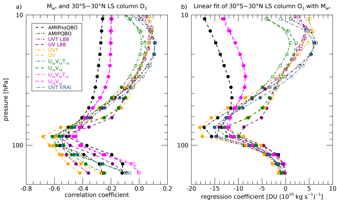
Figure S1: Same as Fig. 4, but for lower stratospheric column ozone computed over 30°S to 30°N.
