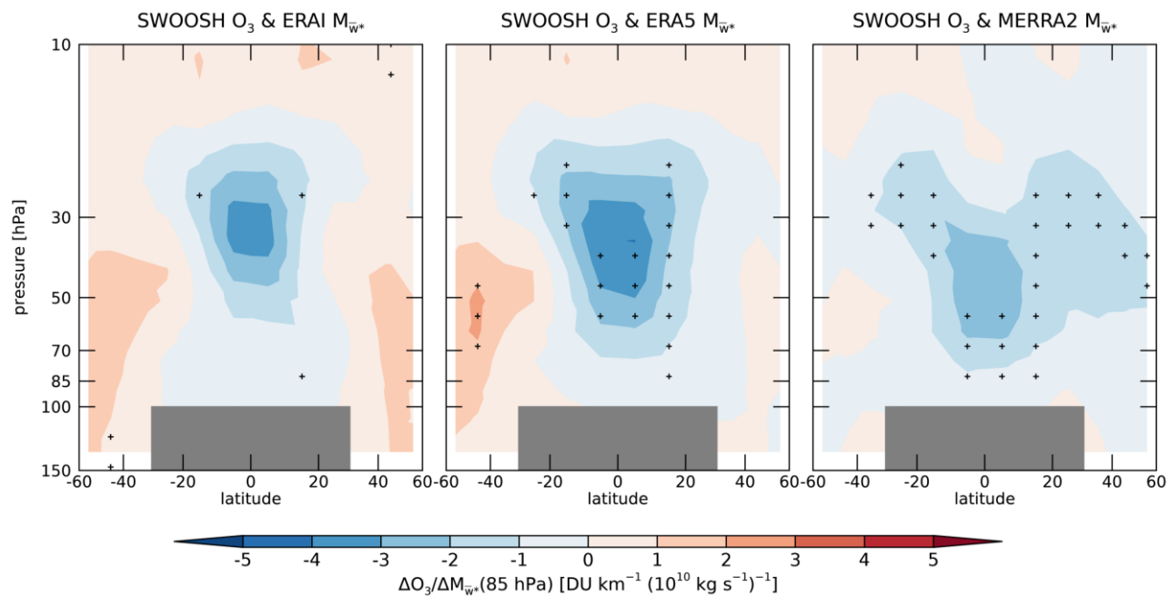
5 Figure S2: As in Fig. 5, but including all reanalyses.
