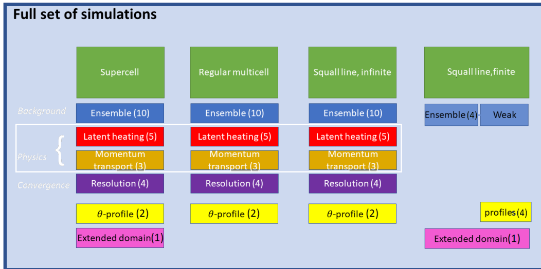
Figure 1. Overview of all CM1 experiments done in this study. The four scenarios have been introduced-represented in Section 2.2 and perturbations-the columns of the display have been introduced in this Section (Section 2.3)2.2. The-These green boxes with white caption show each of the four prototypes of convection that we use, with a list of experiment groups following in the column below each of them. Below the column header, the perturbations applied to each scenario are represented, which are discussed in the order of display (downward; Section 2.3). Here, white text represents the regular basis set of perturbation experiments applied to the first three modes of convection and black fonts represent irregularities among the experiments, tailored at specific modes of convection and robustness testing. In the last column "weak" denotes the ensemble band corresponding with-to the other three scenarios and "profiles" denote the wide ensemble band, which correspond better-with-to \theta -profile perturbations in the other three scenarios ( Section-Sections 2.3.1 and 2.3.3 ).
