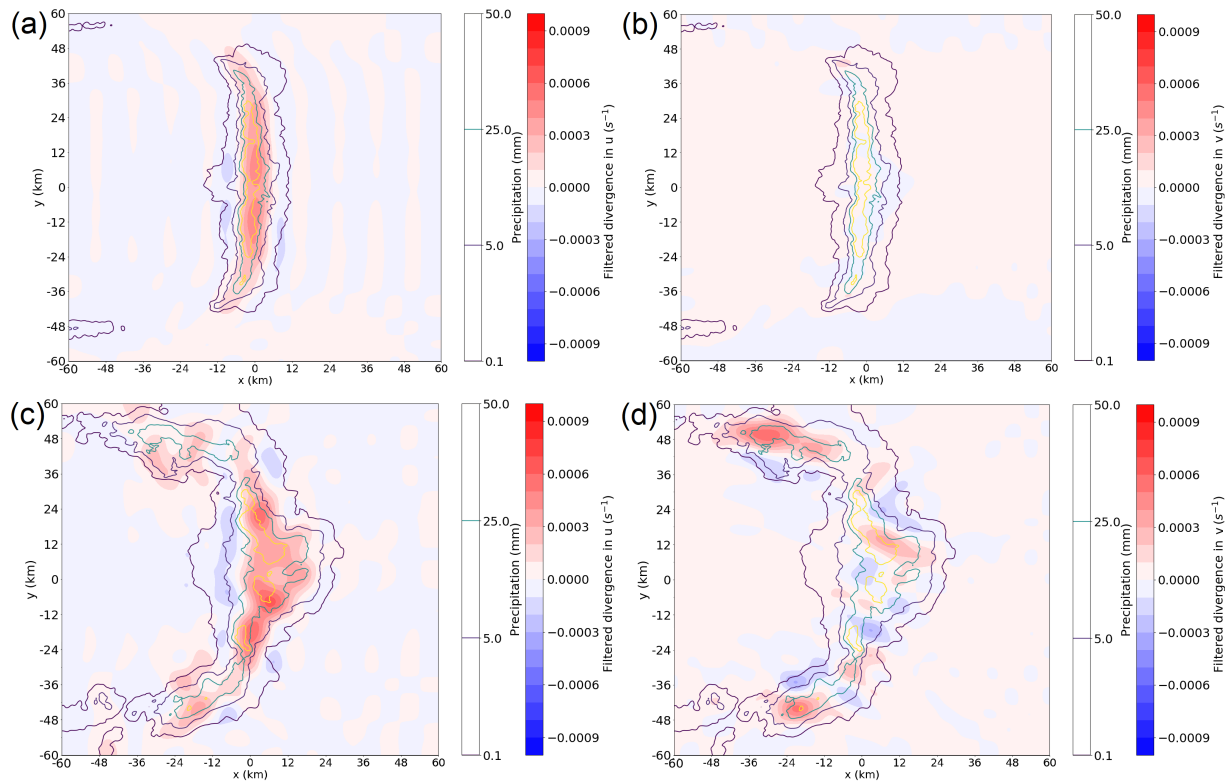
Figure 6. Spatial distribution of filtered divergence over altitudes 7-14 km for a finite squall line during (a, b) first and bottom (c, d) time interval. Wavelengths that fit more than 20 times in the domain have been removed with a discrete cosine transform. Contours indicate the accumulated precipitation pattern during each of the two time intervals (0.1, 5, 25, 50 mm, as displayed in one of the two colour bars). Both the zonal (a, c) and the meridional component (b, d) are displayed separately.
