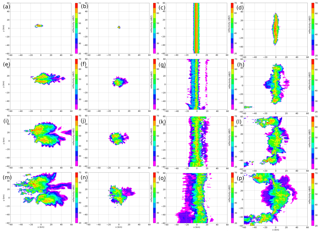
Figure 2. Simulated radar reflectivity at 3 km height in the control simulation for each of the four modes of convection: from left to right Supercell (a, e, i, m), regular multicell (b, infinite-length f, j, n), infinite-length squall line (c, g, k, o) and finite-length-finite-length squall line (d, h, l, p). From top to bottom time increases: 30 min (top row, a, b, c, d), 60 min (second row, e, f, g, h), 90 min (third row, i, j, k, l) and 120 min (bottom row, m, n, o, p).
