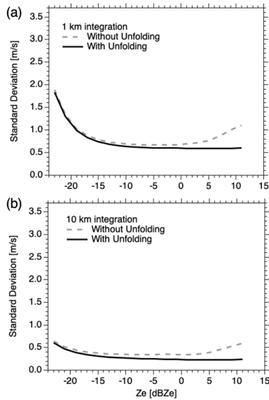
165 Figure 4. Standard deviation of random error of simulated Doppler velocities for PRF of the low mode (higher PRF) as a function of Z_e for (a) 1 km integration and (b) 10 km integration. The solid lines denote the results with unfolding correction.
