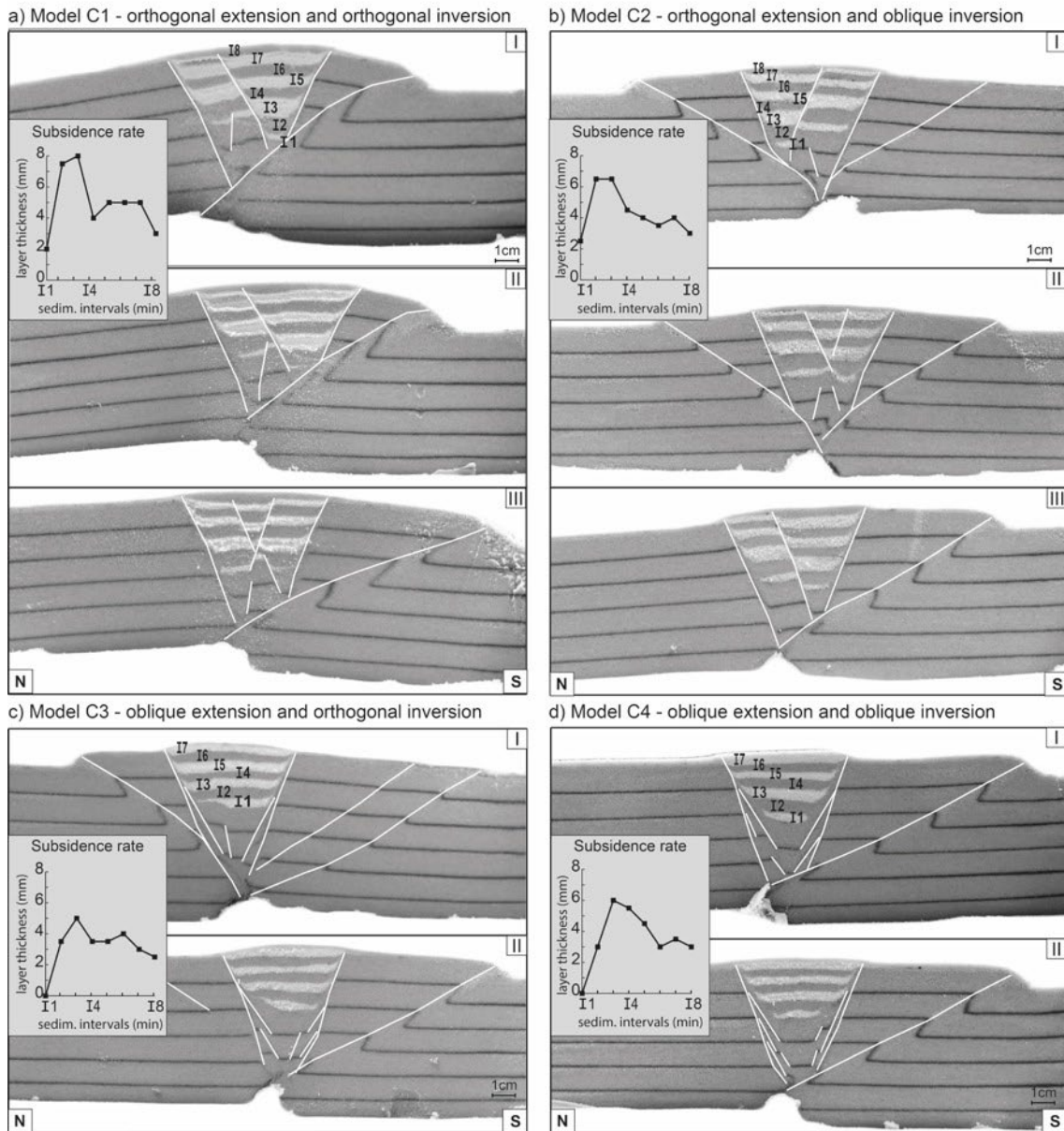
410 Figure 7: a), b), c) and d) Sections of experiments with sedimentation and measurements on models showing the influence of extension obliquity on sedimentation and subsidence rate. Section locations are shown in Figs. 5 and 8. Syn-rift sedimentation units always start with feldspar sand (white) and are divided into 8 intervals of 15 minutes of extension, except for the oblique divergence models C3 and C4, where I1 and I2 are represented in the same unit. I1 = 15 min, I2 = 30 min, I3 = 45 min, I4 = 60 min, I5 = 75, I6 = 90 min, I7 = 105 min, I8 = 120 min (after the initiation of rifting). Section orientations are indicated at the bottom section of each model.
