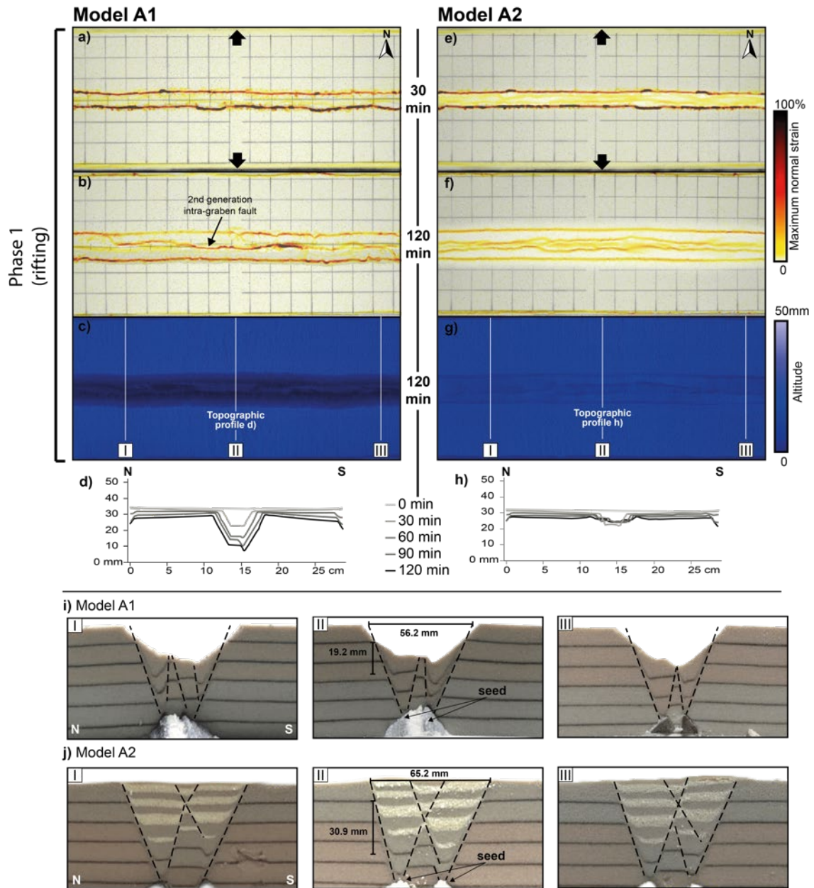
Figure 3: Evolution of deformation during rifting for models A1 (no sedimentation) and A2 (with sedimentation). a), b), e) and f) display top view maximum normal strain results for early and late-stage rifting, respectively, c) and g) show top views of digital elevation models at the end of rifting. d) and h) Topographic profiles for every 30 minutes of rifting. Vertical exaggeration = 4. Note that topography is shown prior to syn-rift sedimentation for that interval. i-j) Sections for Model A1 and Model A2, respectively. Section locations are indicated in (c) and (g). Graben geometry measurements are indicated in the middle sections (i ii and j ii ).
