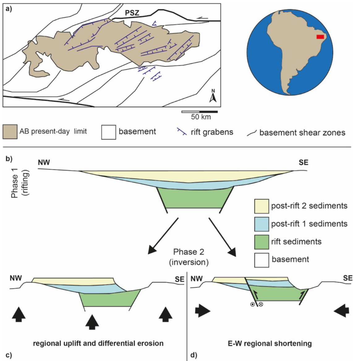
Figure 1: a) Structural geology of the study area and present-day Araripe Basin (AB). NE-SW striking rift-related structures (in blue) and Precambrian basement shear zones (in black), modified after Camacho and de
