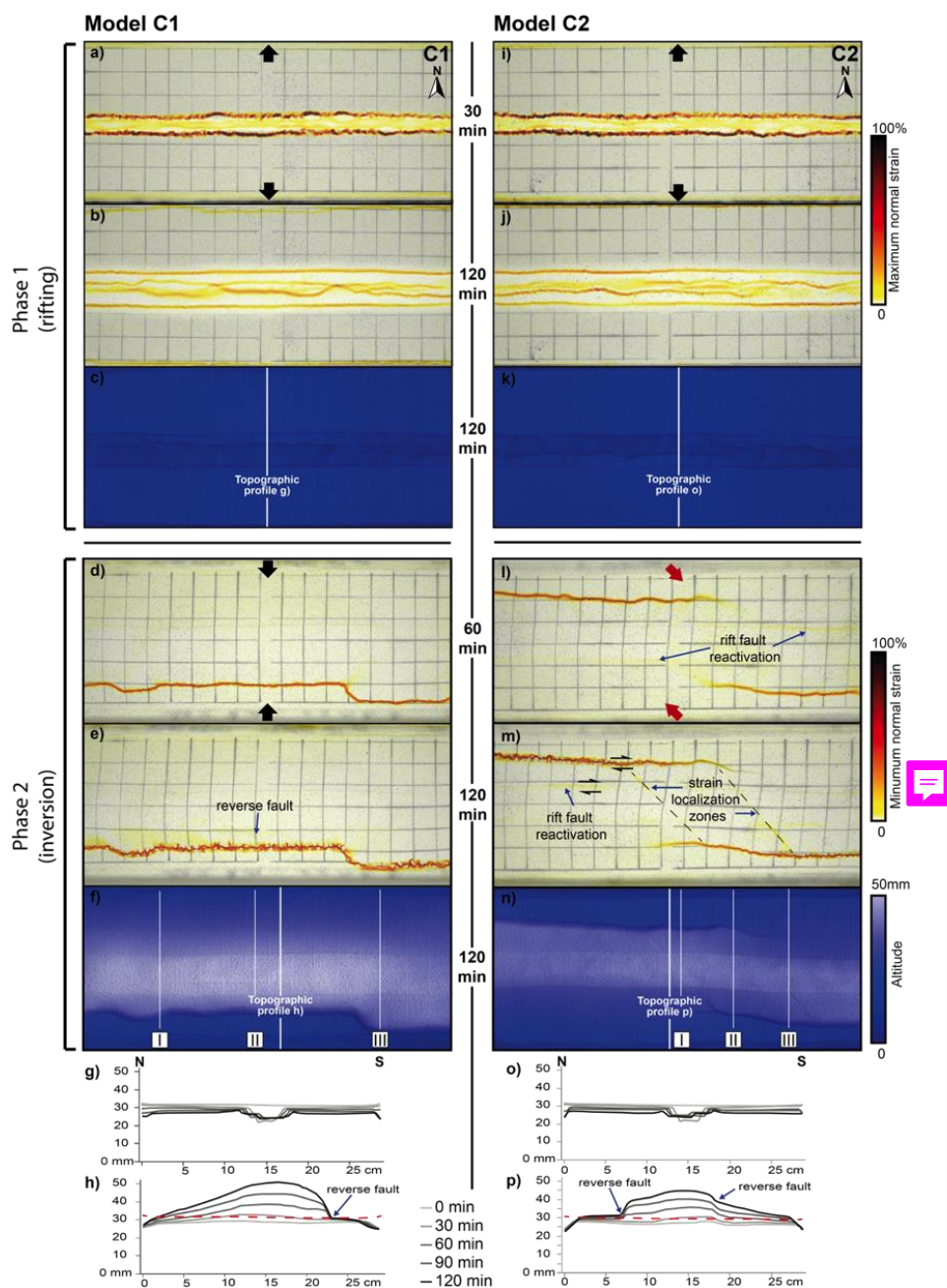
Figure 6: Evolution of deformation during rifting and inversion for Models C1 and C2. a) and b) displays top view model DIC analysis for Maximum normal strain at early and late rifting stage. c) Digital elevation model for late rifting stage. d) and e) displays top view model DIC analysis for Minimum normal strain. f) Digital elevation model for late inversion stage. g) Topographic profiles for every 30 minutes of rifting phase. h) Topographic profiles for every 30 minutes of inversion phase.
