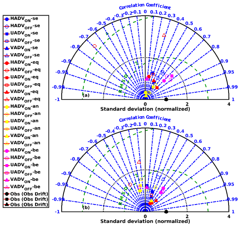
675 Figure A.3: Taylor diagrams comparing seasonal variations of horizontal/zonal/meridional heat advection (HADV/UADV/VADV) from observations (gridded advection named Obs (a); Lagrangian advection named Obs Drift (b)) and model (online advection for ON and offline advection for OFF) in Senegal, Equatorial, Angola and Benguela boxes (blue, red, yellow and magenta colors respectively).
