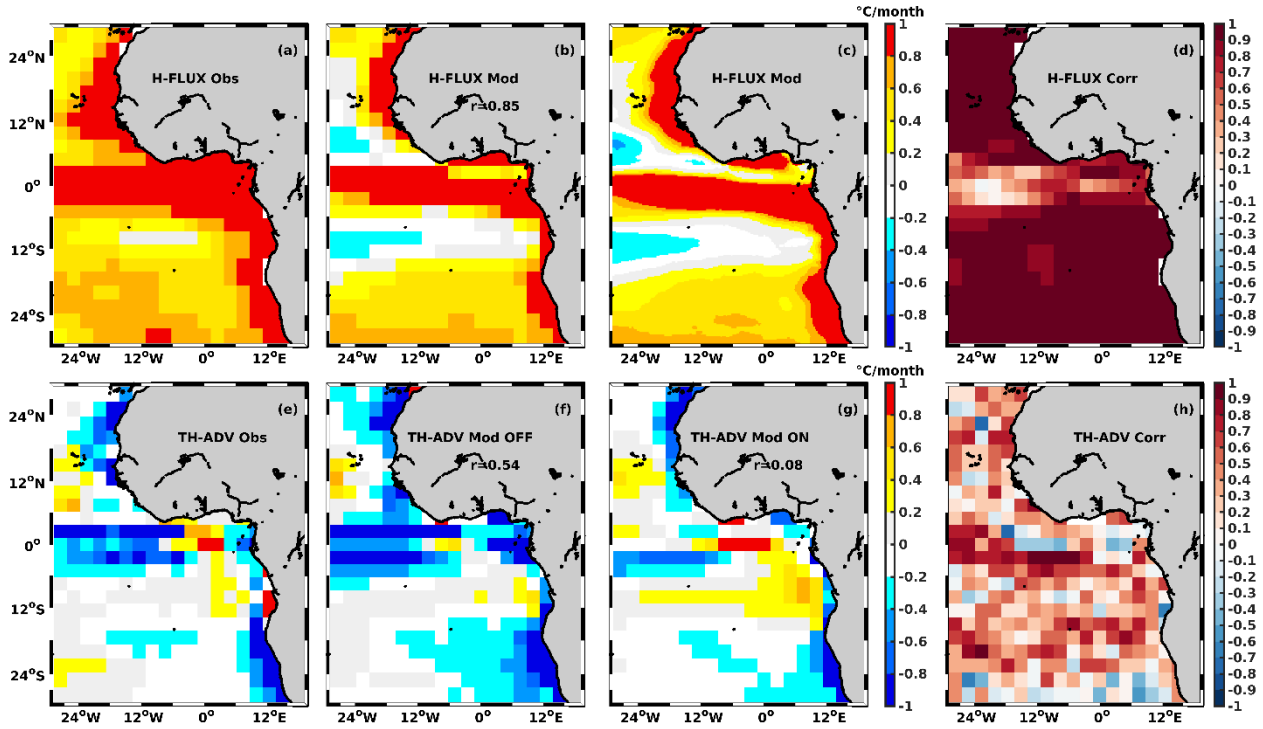
Figure 4: Mean heat flux from PREFCLIM (a), NEMO re-sampled at PREFCLIM 2.5° resolution (b) or at original 0.25° resolution (c), and seasonal correlation between PREFCLIM and NEMO heat flux (d). Mean horizontal heat advection from PREFCLIM (e), NEMO offline (f) or online computation re-sampled to 2.5° resolution (g), and seasonal correlation between PREFCLIM and NEMO offline advection (h). r in (b), (f) and (g) indicates the spatial correlation between PREFCLIM and NEMO, which is 95% significant when r > 0.12 . The temporal correlation of seasonal cycles in (d) and (h) is 95% significant when r > 0.58 .
