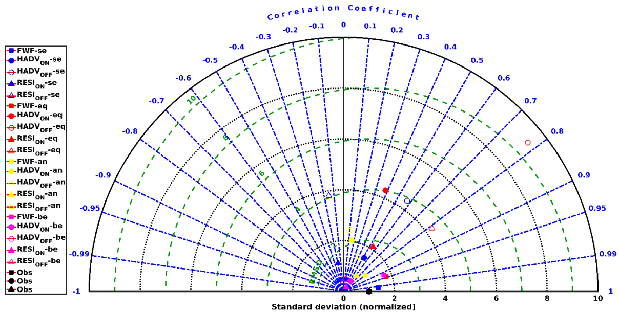
485 Figure 9: Taylor diagram of global terms of salt budget in selected regions. Freshwater flux, horizontal advection (gridded advection for observations and online advection for model), and (pseudo-) residuals are represented by squares, circles, triangles respectively. Empty circles and triangles are offline advection and associated (pseudo-) residuals. Senegal, Benguela, Equatorial and Angola regions are designed by blue, red, yellow and magenta colors respectively. Correlations are 95% significant when r > 0.58 .
