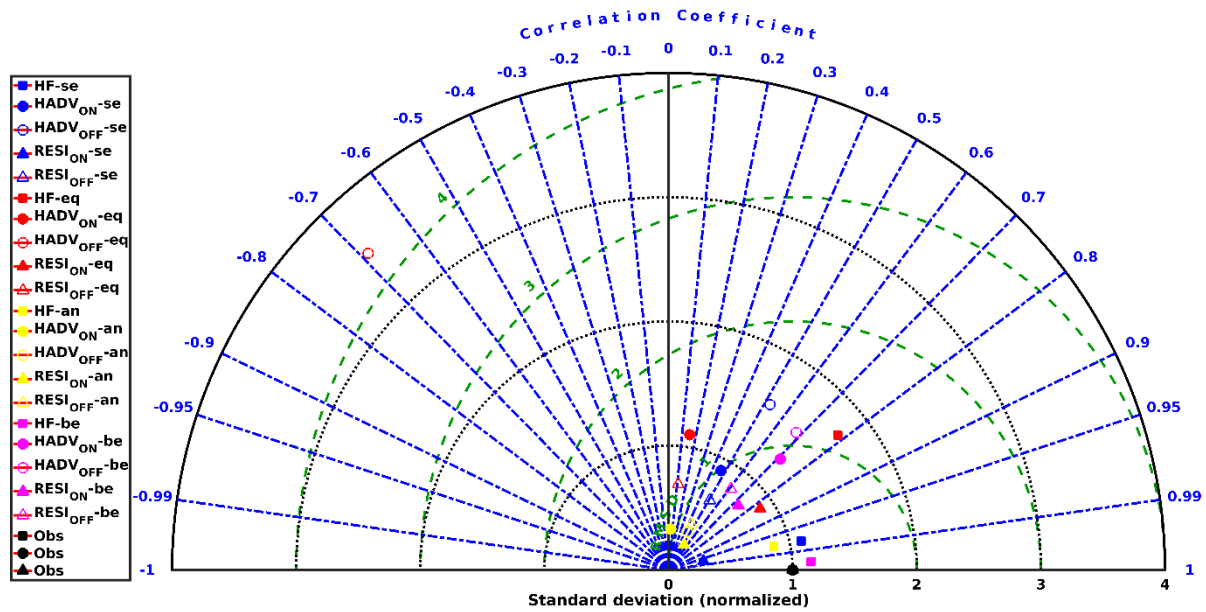
Figure 6: Taylor diagram of global terms of heat budget in selected regions. Heat flux, horizontal advection (gridded advection for observations and online advection for model), and (pseudo-) residuals are represented by squares, circles, triangles respectively. Empty circle and triangle are offline advection and associated (pseudo-) residuals. Senegal, Benguela, Equatorial and Angola regions are designed by blue, red, yellow and magenta colors respectively. Correlations are 95% significant when r > 0.58 .
