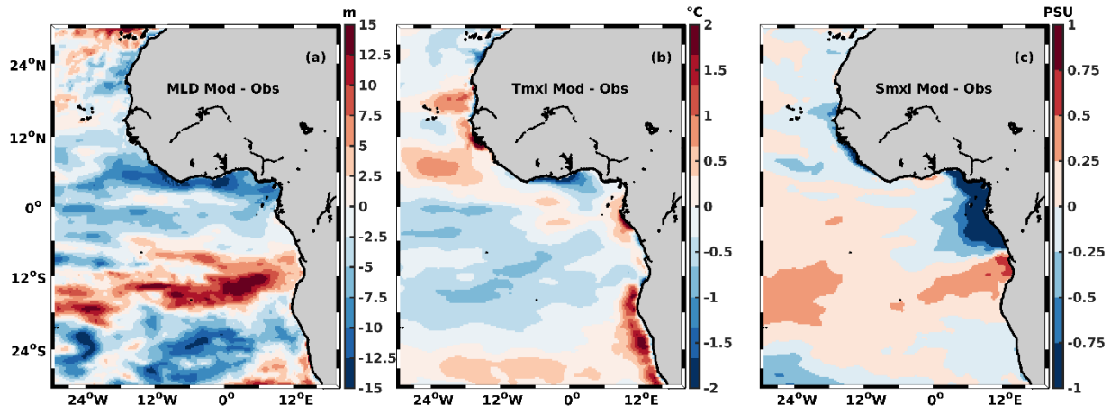
670 Figure A.1: Difference between observations and model in mixed-layer depth (a), mixed-layer temperature (b) and mixed-layer salinity (c).
