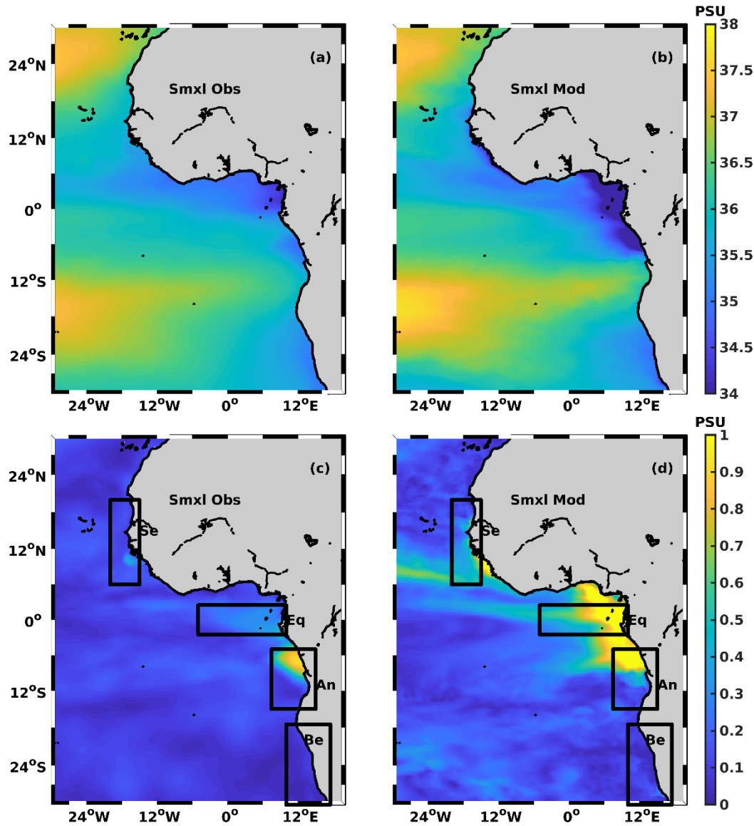
255 Figure 3: Annual mean (a and b) and standard deviation (c and d) of mixed-layer salinity from observations (left: a and c) and model (right: b and d). The rectangles in the bottom panels correspond to the 4 boxes of study.
