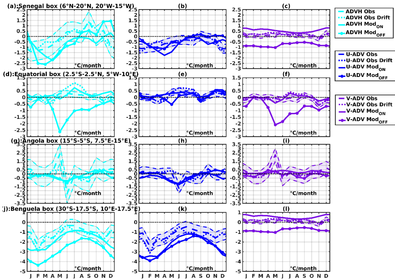
680 Figure A.4: Seasonal cycle of horizontal (cyan), zonal (blue), and meridional (purple) heat advection from observations (dashed line for gridded advection and dotted line for Lagrangian advection) and model (full line for online and full dotted line for offline) in selected boxes. All others terms are in °C per month.
