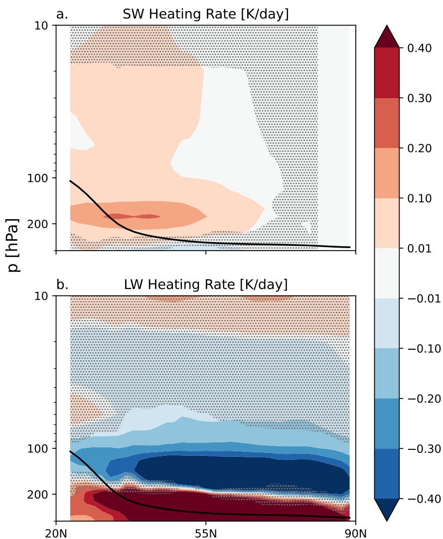
Figure C1. Five-year northern hemisphere zonal mean SW and LW heating rate anomalies in K/day for the r0.01 high-seeding case (emissions radius of 0.01 \mu\text{m} and a mass emissions scaling factor of 1000) for the period November to February. The black line denotes the WMO-defined tropopause and the blue dashed line is the 238 K temperature contour. The stippling denotes insignificant data points at the 95% confidence level according to the independent t-test controlled by the false discovery rate method.
