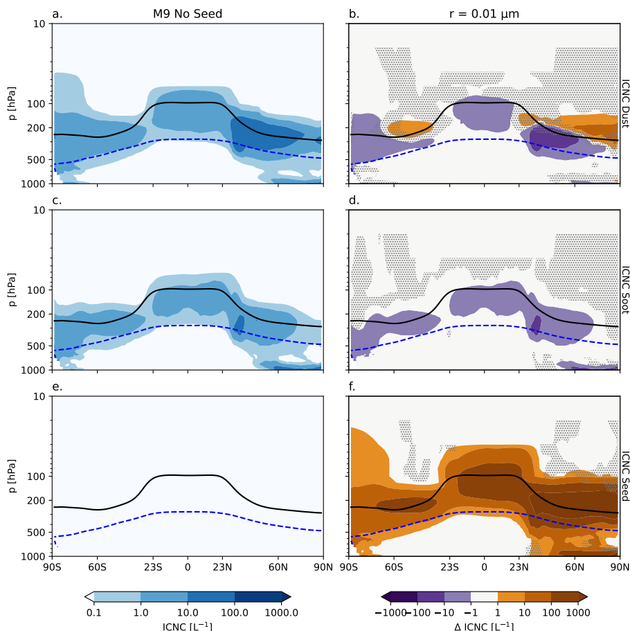
Figure B1. Five-year annual zonal mean in-situ cirrus heterogeneous nucleation ice sources in L^{-1} for the unseeded reference case in the first column, and the anomalies for the seeding scenario r_{0.01} high-seeding (emissions radius of 0.01 \mu\text{m} and a mass emissions scaling factor of 1000) in the second column. Each row represents a heterogeneous nucleation source for mineral dust (first row), soot (second row), and seeding particles (third row). The black line denotes the WMO-defined tropopause and the blue dashed line is the 238 K temperature contour. The stippling denotes insignificant data points at the 95% confidence level according to the independent t-test controlled by the false discovery rate method.
