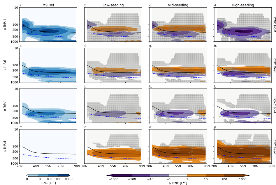
Figure 8. Five-year northern hemisphere wintertime zonal mean in-situ cirrus ice sources in L^{-1} for homogeneous nucleation and the sources of heterogeneous nucleation for the unseeded reference case in the first column, and the anomalies for seeding with a factor of 10 (low-seeding, second column), 100 (mid-seeding, third column), and 1000 (high-seeding, fourth column). The first row shows the homogeneous nucleation source. The second, third, and fourth rows each represent a heterogeneous nucleation source for mineral dust (second row), soot (third row), and seeding particles (fourth row). The black line denotes the WMO-defined tropopause and the blue dashed line is the 238 K temperature contour. The stippling denotes insignificant data points at the 95% confidence level according to the independent t-test controlled by the false discovery rate method.
