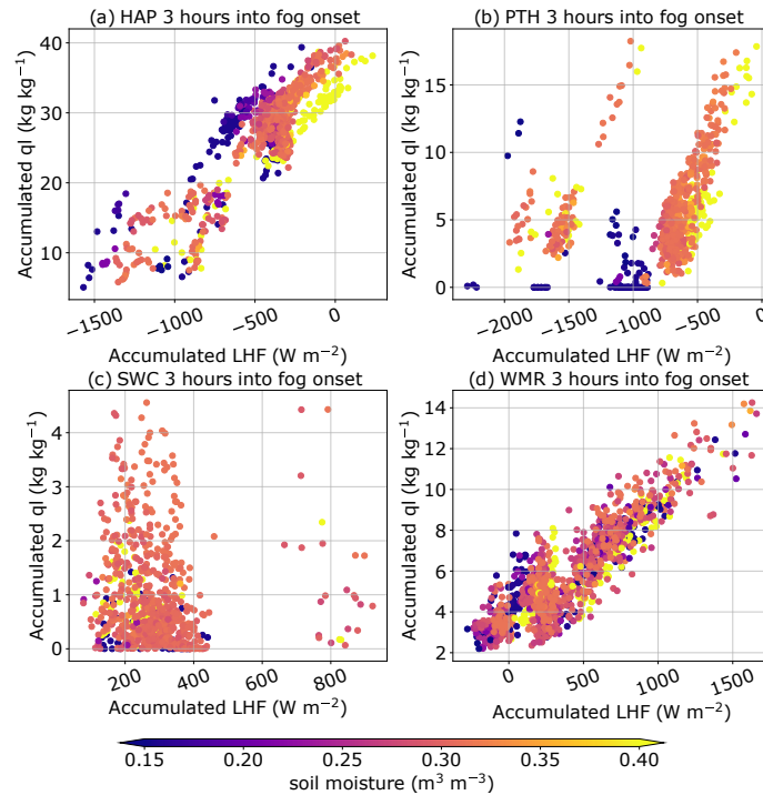
Figure 12. Scatter plots showing accumulated latent heat flux (LHF) against accumulated q_l coloured by soil moisture for (a) HAP, (b) PTH, (c) SWC, and (d) WMR. Data samples were obtained from each grid point at 1 km scale for all simulations. The accumulation period is 3 hours into fog onset.
