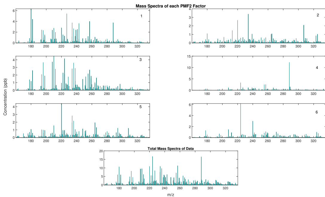
Figure 1. Mass spectra profiles of the six PMF2 factors labeled by order, as well as the total mass spectra concentration of the data.
