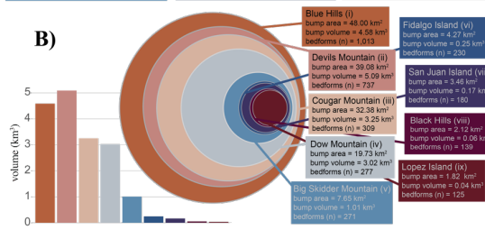
Figure 1: (A) Site overview across the Puget Lowland with inset reference of CIS glaciation (14 kya; Ehlers et al., 2010). Site maps for i) the Blue Hills, ii) Devils Mountain, iii) Cougar Mountain, iv) Dow Mountain, v) Big Skidder Mountain, vi) Fidalgo Island, vii) San Juan Island, viii) the Black Hills, and ix) Lopez Island. Streamlined subglacial bedforms are mapped upstream (gray polygons), on top of (black polygons), and downstream (blue polygons) of bed bumps (small white outlines) within larger site regions (large white outlines). (B) Relative volume and surface area of bed bump sites.
