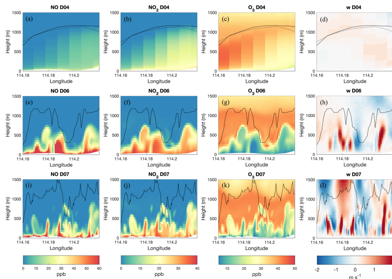
575 Figure 12. Vertical distribution of simulated NO (first column), NO 2 (second column), O 3 (third column) mixing ratios (ppbv), and vertical wind velocity (w; fourth column) along a busy east-west road near the Mong Kok station (Argyle Street, see Fig. 3b) at 13:00 LT for the D04 (first row), D06 (second row), and D07 (third row) cases. The black solid lines represent the calculated PBLH, and the black dash line the PBLH from the model output for the mesoscale domain, which is calculated in the YSU PBL scheme.
