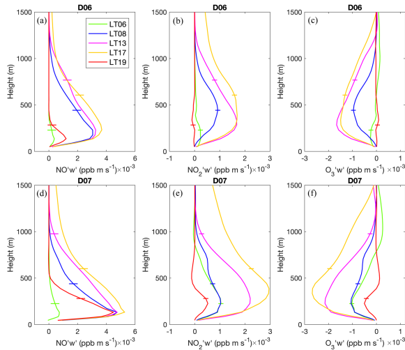
Figure 15. Horizontally averaged hourly mean profiles of the vertical fluxes of NO (left), NO_2 (middle), and O_3 (right) in selected regions highlighting the diurnal cycle on August 1, 2018.
