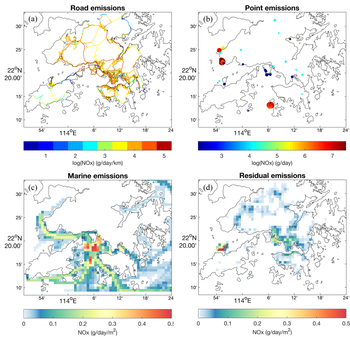
Figure 2. Emission maps of NO x provided by HKEPD for the Hong Kong region from road (a), point (b), marine (c), and residual (d) sources. The road emissions are shown as line sources for every road with the unit of g day -1 km -1 . For simplification, all the roads, including those above and below ground, are added in one layer at the surface. The point sources include power plants, industries, crematoriums, and
