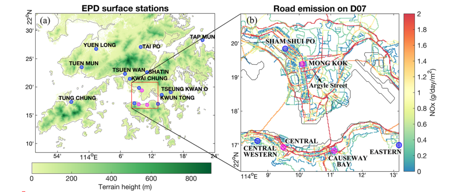
Figure 3. Locations of the surface monitoring stations represented on the map of the Hong Kong topography (a) and the road emissions interpolated to D07 domain grids (b). The blue circles represent the general stations and the magenta circles the roadside stations.
