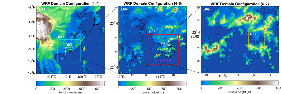
Figure 1. Setup of the seven one-way nested WRF domains and a representation of the topography adopted in the model.
