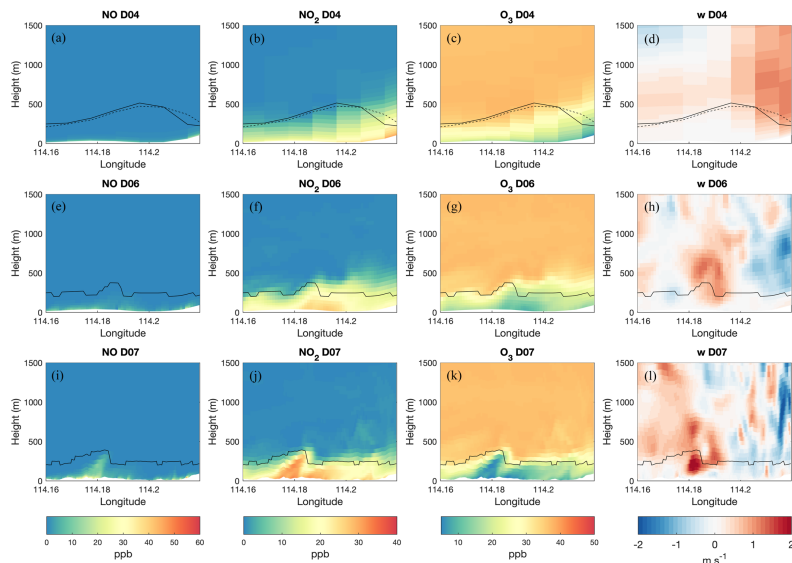
Figure 11. Vertical distribution of simulated NO (first column), NO 2 (second column), O 3 (third column) mixing ratios (ppbv), and vertical wind velocity ( w ; fourth column) along a busy east-west road near the Mong Kok station (Argyle Street, see Fig. 3b) at 6:00 LT for the D04 (first row), D06 (second row), and D07 (third row) cases. The black solid lines represent the calculated PBLH, and the black dash line the PBLH from the model output for the mesoscale domain, which is calculated in the YSU PBL scheme.
