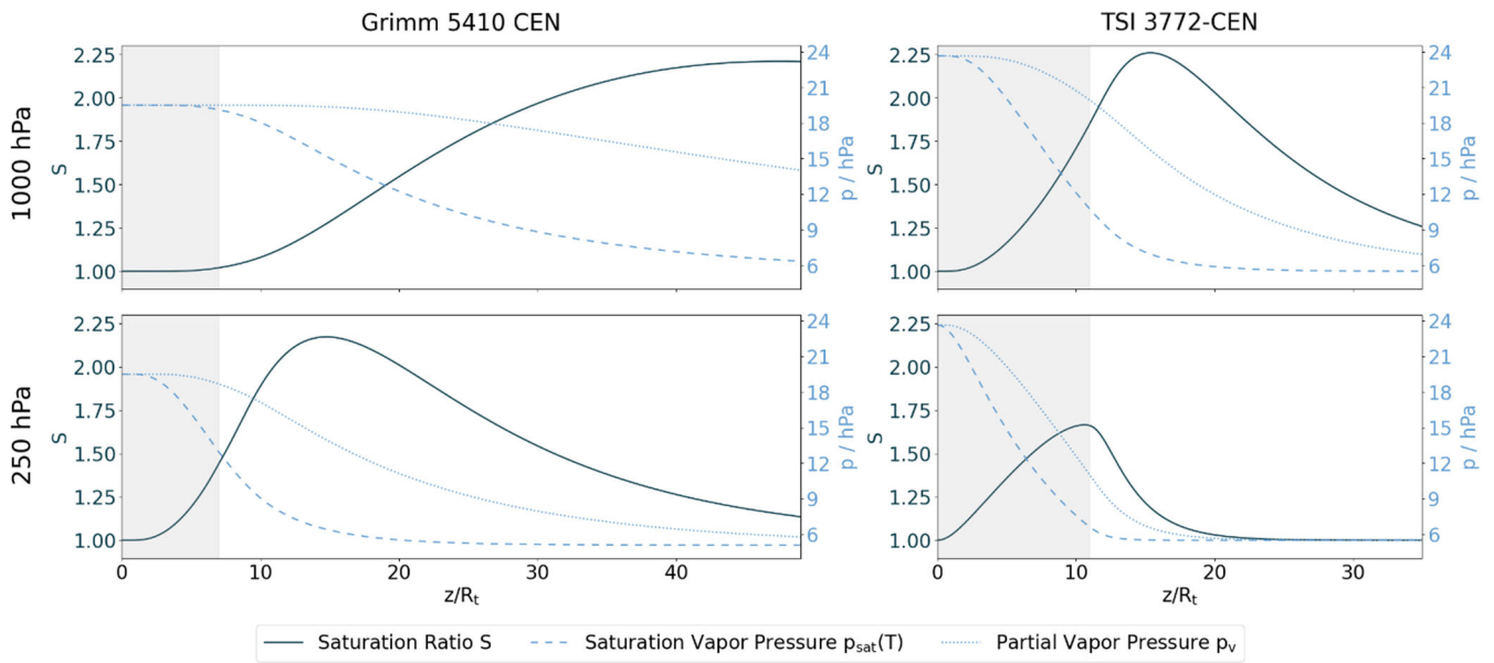
840 Figure 5: Centerline profiles of the saturation ratio S , the saturation vapor pressure and the partial vapor pressure of butanol resulting from the CPC's insulator and condenser simulations (see Figure 4). The left column shows the results for the Grimm 5410 CEN CPC and the right column for the TSI 3772-CEN CPC. The upper row represents the 1000 hPa case, the lower row the 250 hPa one. The x-axis represents the normalized length z' = z/R_t and is set to the same scale for both CPC-models. The insulator part is shaded in grey. The y-axis of the saturation ratio S is on the left side, for the vapor pressures on the right one.
