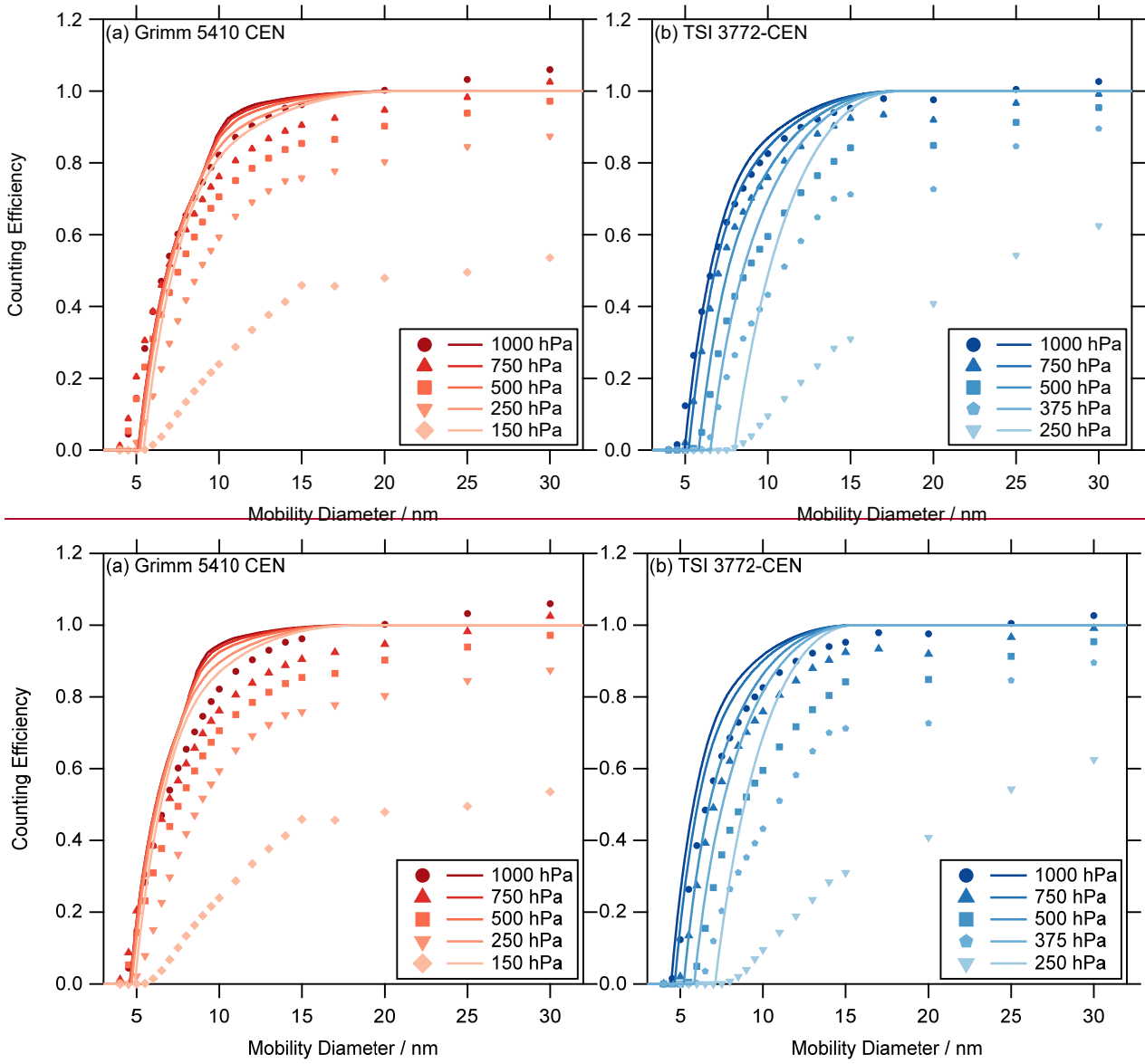
Figure 6. Activation efficiency \eta_a curves (lines) ((a) Grimm 5410 CEN and (b) TSI 3772-CEN) calculated from the simulations (Figure 4) for the different pressure stages. The markers are for reference and represent the results of the measured counting efficiencies (Figure 3).
