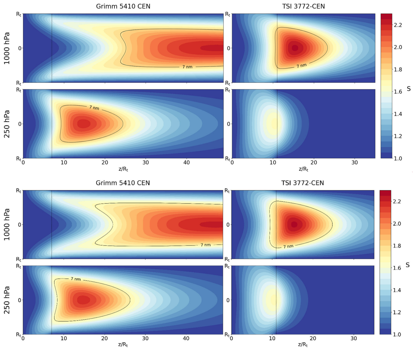
Figure 4: Simulated saturation ratio S of the CPC's insulator and condenser. The left column shows the results for the Grimm 5410 CEN CPC and the right column for the TSI 3772-CEN CPC. The upper row represents the 1000 hPa case, the lower row the 250 hPa one. The x-axis represents the normalized length z' = z/R_t and is set to the same scale for both CPC-models. The length of the insulator is marked with a vertical dashed line. The black 7-nm-line encloses the area where the supersaturation is sufficient to activate particles with a Kelvin diameter of at least 7 nm (Eq. (9)). The centerline profiles (at r = 0 ) of the saturation ratio and the corresponding vapor pressures are presented in Figure 5.
