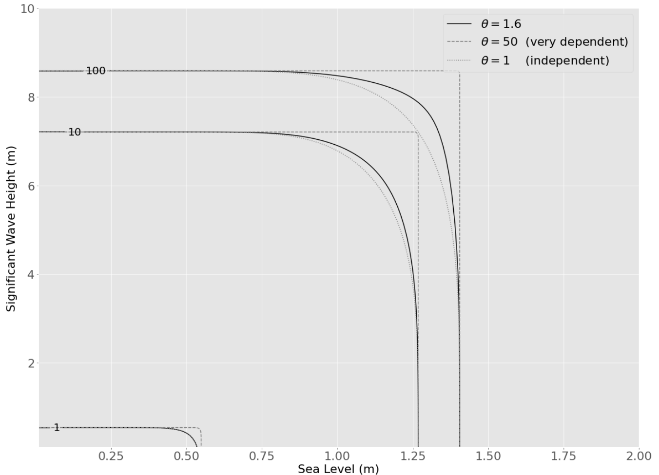
Figure 4. Return period (in years on the contour lines) of an event composed of a couple (N, H_0) or with a higher value of N or H_0 , noted as RP(E(N > x || H_0 > y)) with the interdependence factor having a value of \theta \approx 1.6 \theta \approx 1.23 (full line). The independent copula (dotted lines) and the high-dependence copula (dashed lines) are also displayed for reference.
