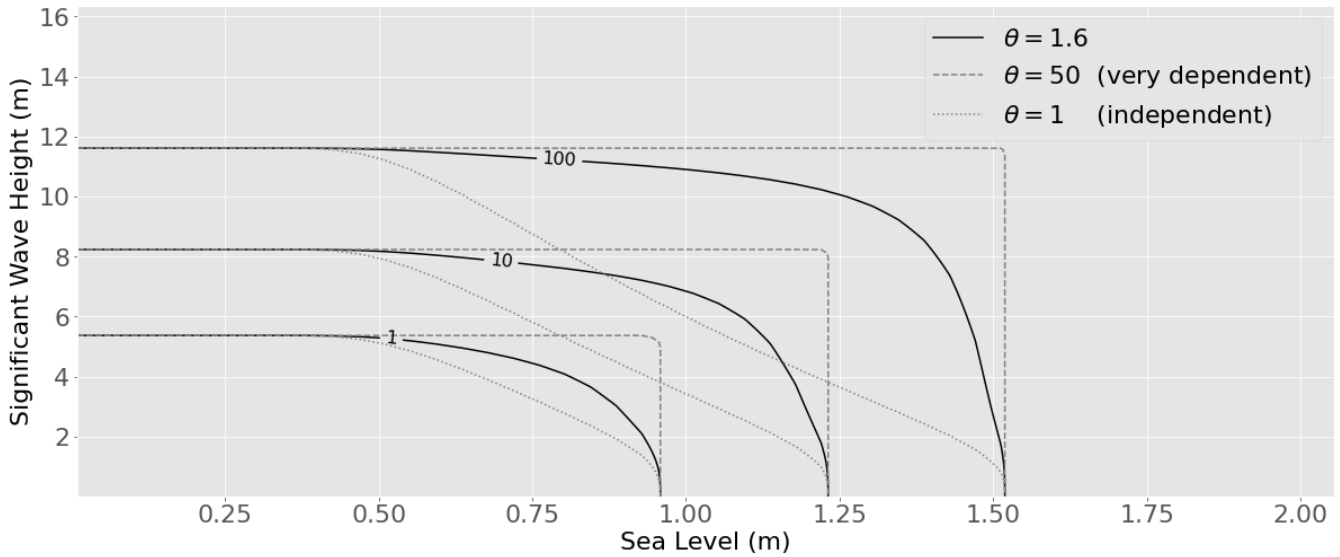
Figure 5. Return period (in years on the contour lines) of an event composed of a couple (N, H_0) or with a higher value of N or H_0 , noted as RP(E(N > x | H_0 > y)) with the interdependence factor having a value of \theta \approx 1.6 (full line). The independent copula (dotted lines) and the high-dependence copula (dashed lines) are also displayed for reference.
