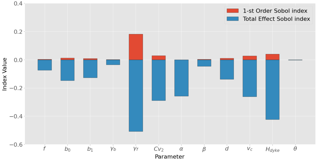
Figure 7. Value of the 1st-order sensitivity (in red) and total effect (in blue) indices for each tested parameter.
