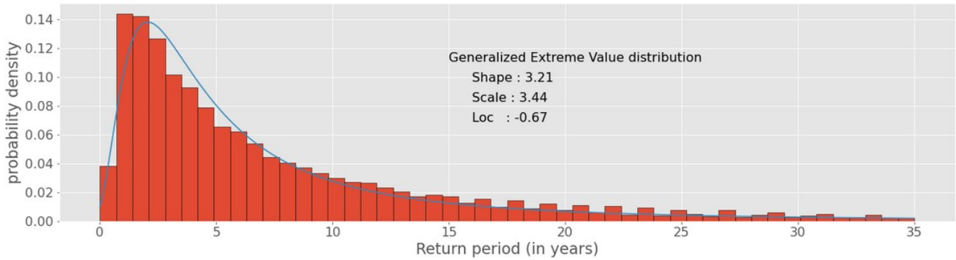
Figure 8. Distribution of the return periods of an event able to provoke some amount of erosion to landward slope at the dyke with random variation of the parameters in Table ??-1 according to their respective range of variation. The distribution is determined by three parameters : the localization is the beginning of the distribution at y = 0 , the scale determines how the distribution stretches vertically and the shape controls the skewness of the distribution or how steep the decrease is after the initial peak.
