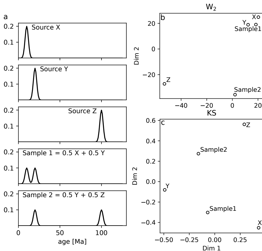
Figure 3. Mixing of discrete endmembers a) Three theoretical, unimodal source age distributions with peaks at 10, 20 and 100 Ma, and two mixture samples. Sample 1 is an equal mixture of X and Y and Sample 2 a mixture of Y and Z. b) Metric MDS map of the three sources and the mixtures using W_2 distance. c) Same as panel b for KS distance. This is a scenario where KS distance may be preferable to W_2 .
