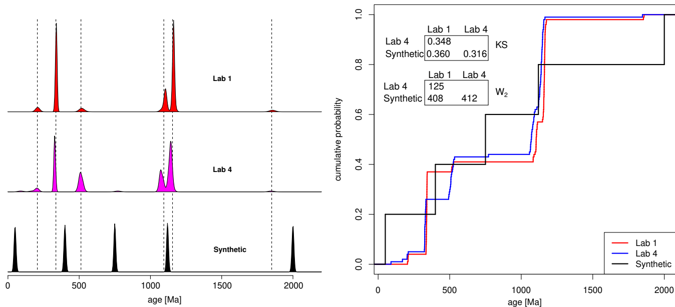
Figure 6. Comparing samples from an inter-laboratory calibration study. KDEs (left) and ECDFs (right) of two samples from the inter-laboratory comparison study of (Košler et al., 2013), plus a purposefully misaligned synthetic sample. Dashed lines mark the true ages of the detrital mixture. According to the KS-statistic, the age distribution produced by Lab 4 is more similar to the synthetic distribution than it is to the distribution produced by Lab 1, despite the absence of any shared age components. The W_2 distance correctly deems the distribution produced by Lab 4 to be closer to that of Lab 1 than to the synthetic mixture.
