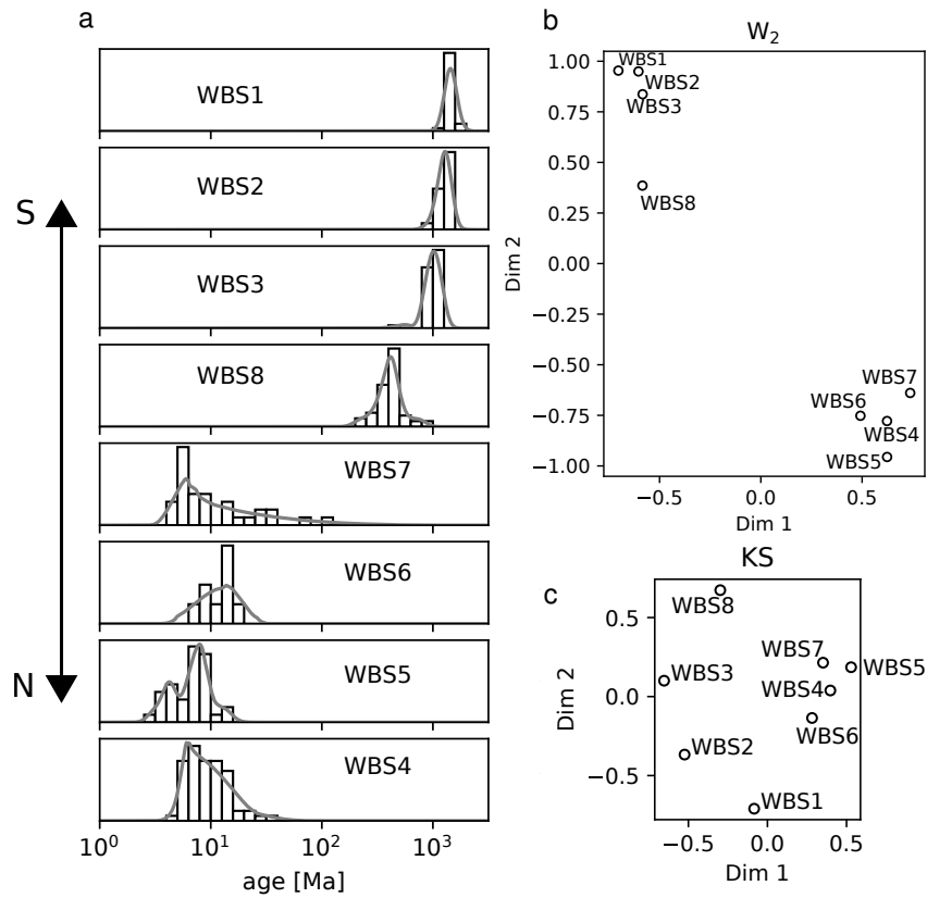
Figure 5. Analysing thermochronological data using W_2 and KS distances. a) KDEs for a detrital mica ^{40}\text{Ar}/^{39}\text{Ar} dataset of Wobus et al. (2003) arranged from south to south-north across a physiographic transition of the central Himalaya in Nepal. Note the logarithmic scale. b) The MDS configuration using W_2 , following a log transform ( stress = 0.02 ). c) MDS map using KS statistic ( stress = 0.18 ). In this example, W_2 performs better than the KS distance at identifying the geographic trend.
