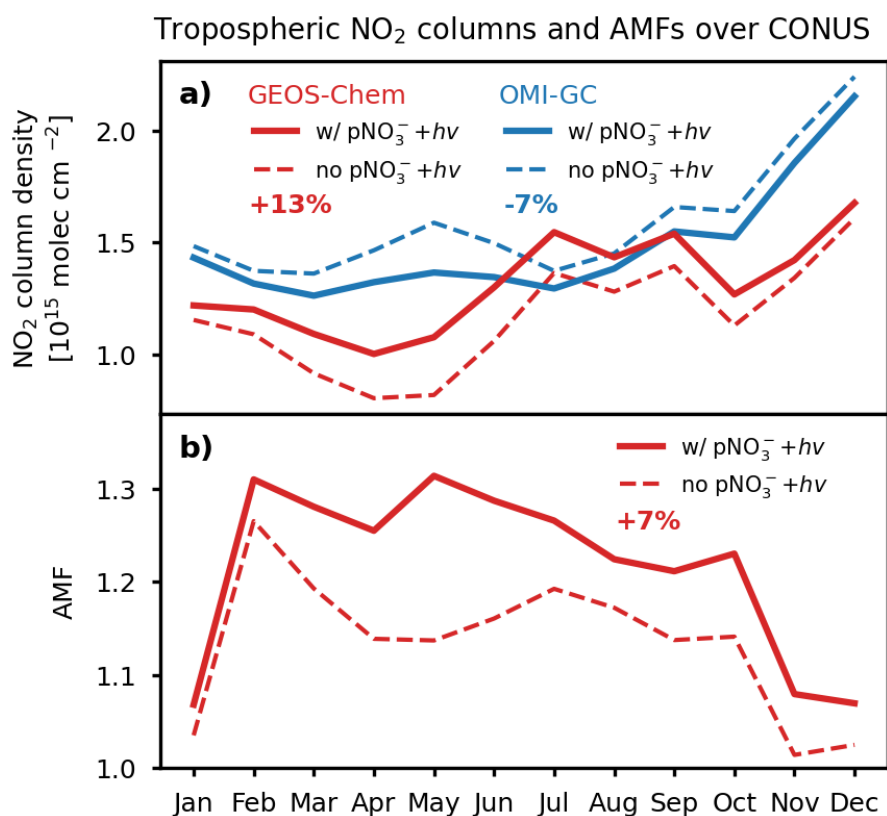
250 Figure 4: Sensitivity to particulate nitrate photolysis of tropospheric \text{NO}_2 vertical column densities (VCDs) simulated by GEOS-Chem and retrieved from OMI satellite observations over CONUS. The top panel shows 2017 monthly mean GEOS-Chem \text{NO}_2 VCDs with and without nitrate photolysis, and the OMI retrieval using GEOS-Chem shape factors (OMI-GC) with and without nitrate photolysis. The bottom panel shows the monthly mean air mass factor (AMF) for OMI tropospheric
