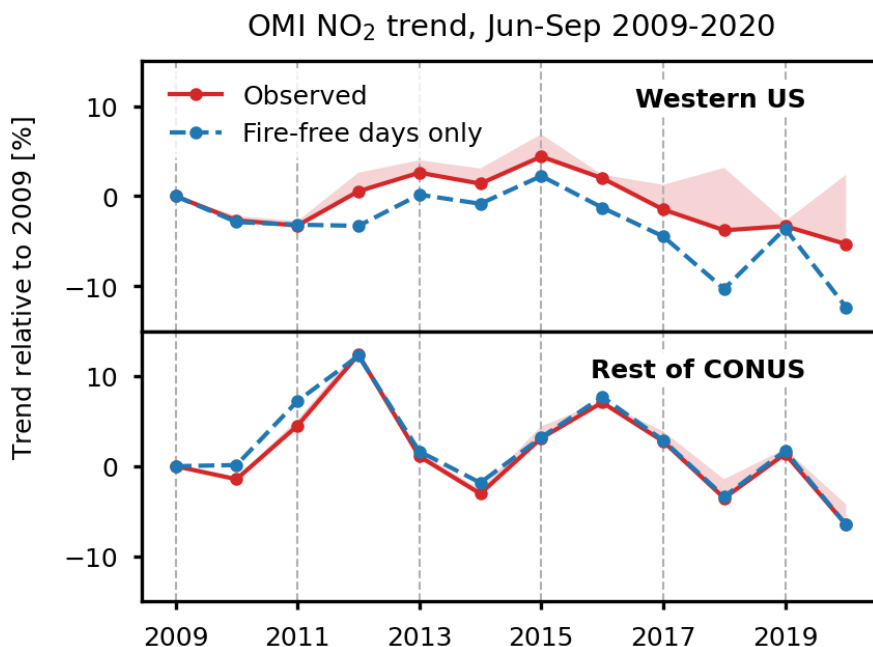
335 Figure 7: Trends of OMI tropospheric NO 2 VCDs over the western US and the rest of CONUS for June-September 2009-2020, examining the effects of fires. Trends are shown relative to 2009. The overall trend from the OMI observations (OMNO2 retrieval) is shown in red, and the trend for the subset of fire-free days is shown as dashed. Fire-free days are identified from the NOAA HMS product (see text). The red envelope shows the effect of a 50% bias correction of the OMI NO 2 retrieval on fire-affected days. The western US domain is defined as (130°-114° W, 30°-50° N).
