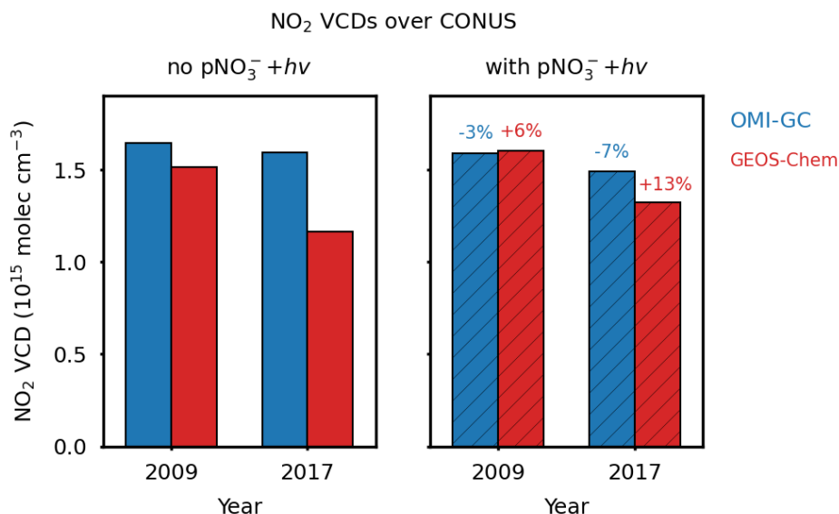
Figure 5. Changes in NO 2 vertical column densities (VCDs) over the contiguous United States (CONUS) between 2009 and 2017 as observed by OMI (OMI-GC) and simulated by GEOS-Chem. Values are annual means averaged spatially over CONUS. The OMI-GC retrievals use GEOS-Chem vertical shape factors and are therefore sensitive to the relative vertical distribution of NO 2 simulated by GEOS-Chem. The left panel shows results for the standard GEOS-Chem simulation without particulate nitrate photolysis, and the right panel shows results from the simulation with particulate nitrate photolysis. The percent changes resulting from the addition of particulate nitrate photolysis are indicated on top of each bar.
