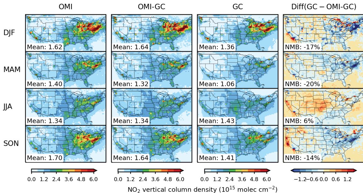
220 Figure 3: Seasonal mean tropospheric NO 2 vertical column densities (VCDs) over CONUS in 2017. From left to right are the OMNO 2 OMI retrievals with AMFs computed using the GMI NO 2 vertical profiles (OMI), the OMI retrievals with AMFs computed using the GEOS-Chem NO 2 vertical profiles (OMI-GC), the GEOS-Chem simulation (GC) sampled along the OMI orbit tracks and for successful OMI retrievals , and the difference between GC and OMI-GC. Mean values over CONUS and normalized mean bias (NMB) between GC and OMI-GC are given inset.
