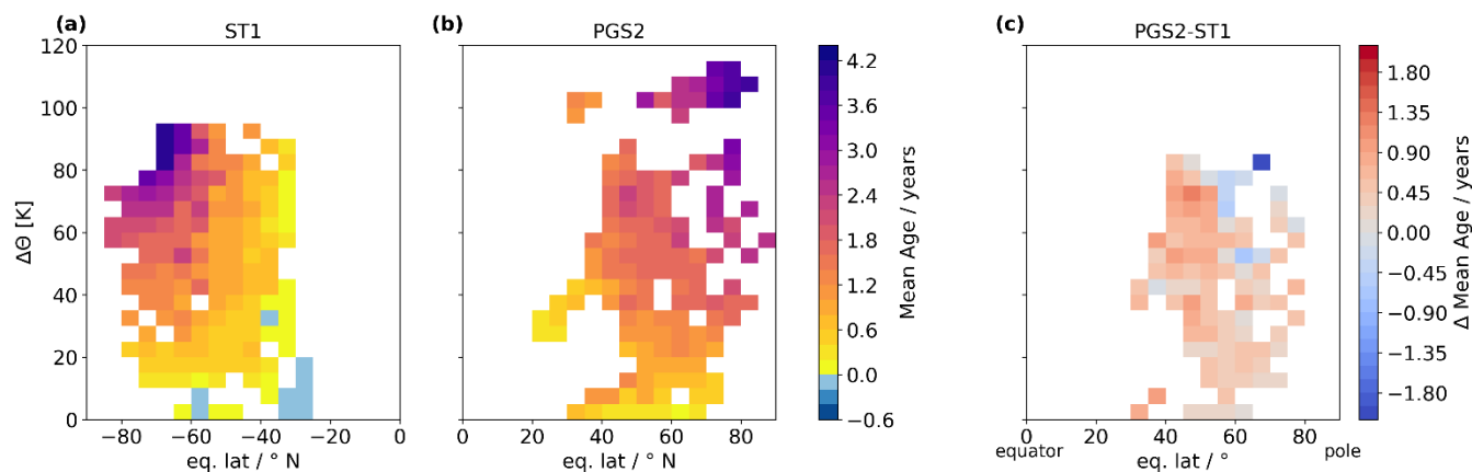
305 Figure 4. Comparison of mean age latitude-altitude distributions during SouthTRAC phase 1 (ST1) (a), PGS phase 2 (PGS2) (b). The hemispheric difference based on these two campaign phases is shown in panel (c). Altitude is given in \Delta\theta . Horizontally, data are sorted by eq. lat.
