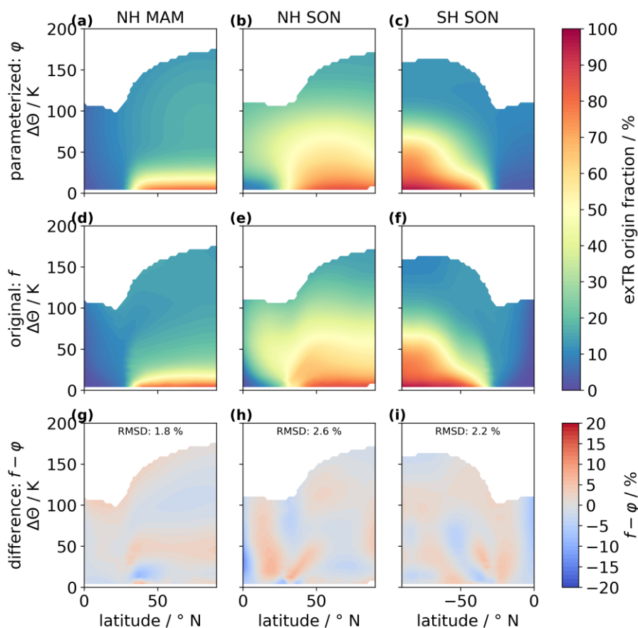
155 Figure 1. Comparing seasonal hemispheric extra tropical origin fractions parameterization ( \varphi , top row) and original CLaMS fractions from simulations from Hauck et al. (2020) ( f , middle row). The difference is shown in the bottom row. Only three selected season-hemisphere combinations are shown here (NH MAM, left column; NH SON, middle column; SH SON, right column). The remaining distributions are shown in Fig. S1. Vertical coordinates are given in potential temperature above the 2 PVU tropopause ( \Delta\theta ).
