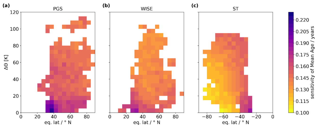
395 Figure 5. Latitude-altitude distribution of sensitivities of mean age from the exTR-TR method to uncertainties in all considered input parameters. Calculated for PGS (a), WISE (b) and SouthTRAC (c) campaign. Altitude is given in \Delta\theta . Horizontally, data are sorted by eq. lat.
