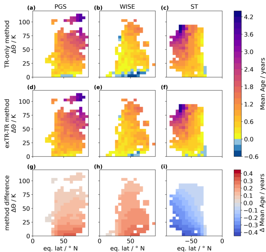
280 Figure 3. Comparison of methods to derive mean age in the LMS during PGS (left column), WISE (middle column) and SouthTRAC (right column). Results are shown for the TR-only method (top row) and the new exTR-TR method (middle row). The absolute differences between both methods are shown in the bottom row. Altitude is given in \Delta\theta . Horizontally, data are sorted by eq. lat.
