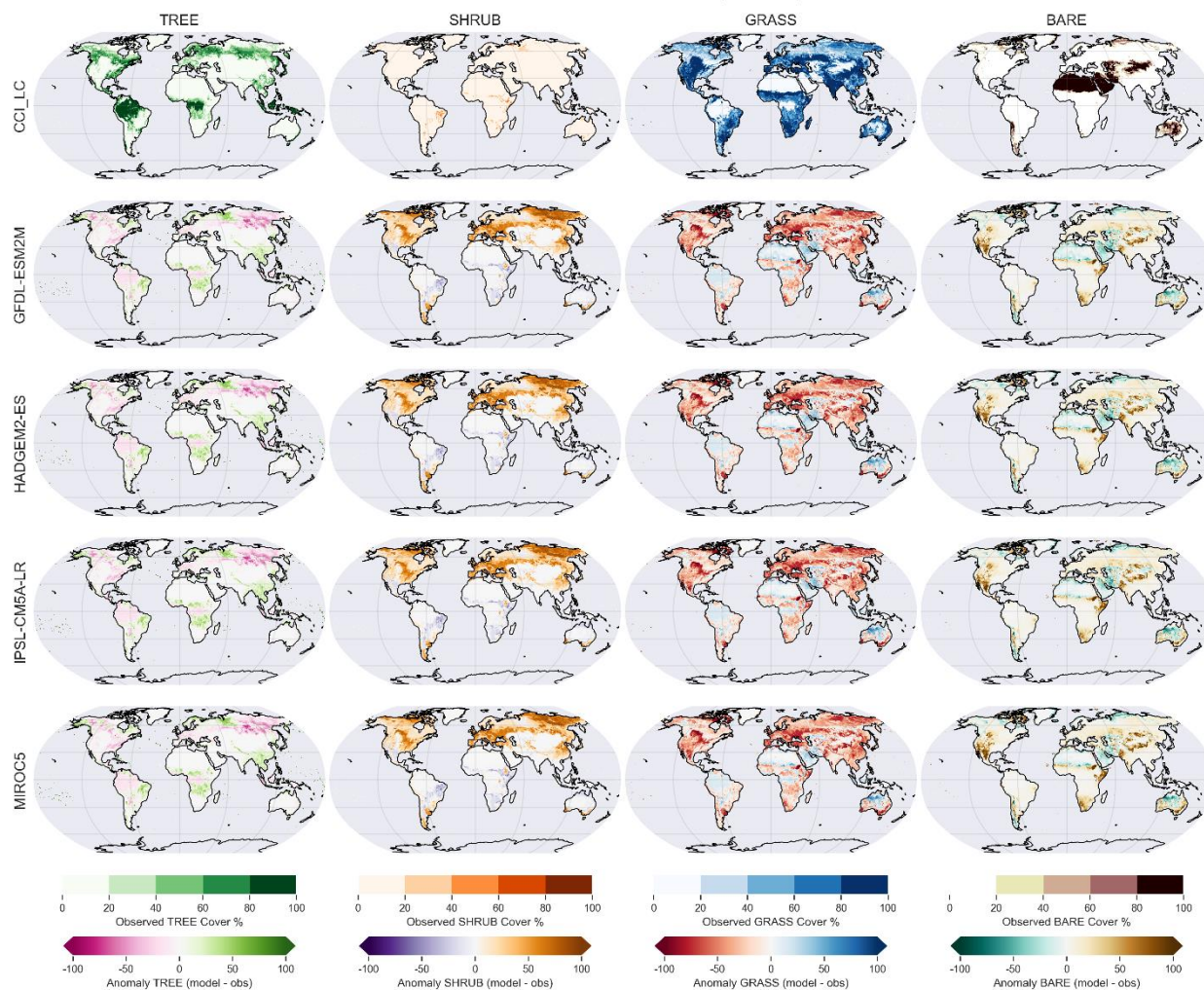
Figure 4: Observed vegetation fractional cover, derived from ESACCI Land Cover (v2.0.7) for 2010 (K. L. Harper et al., 2022), for (left to right) tree, shrub, grass and unvegetated (bare) fraction. Subsequent rows show the difference between model (without fire) and ES CCI observations for each set of driving data.
