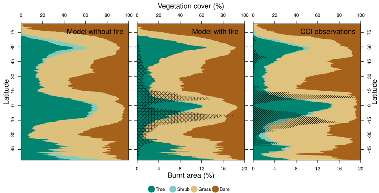
680 Figure 6: Modelled vegetation cover without fire (left) and with fire (middle) compared to observations from ESA CCI Land Cover and Fire (right). Dark green, light green, light brown, dark brown indicates tree, shrub, grass and unvegetated fraction of the latitude band. Shaded transition between colours indicates ensemble range, which is quite narrow indicating agreement across ensemble members. Black hashing indicates burnt area, with observations taken from MODIS CCI v5.1 (Chuvieco et al., 2018). In “Model with fire”, burnt area from the 4 driving models is shown by hatching at 4 different angles.
