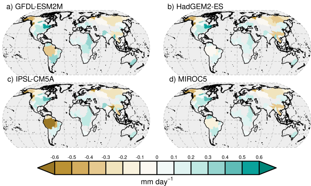
650 Figure 1: Multi-year mean bias of catchment scale runoff simulated by JULES driven by 4 sets of climate driving data compared to runoff derived from (Dai, 2021). Number of years of observations contributing to the multi-year mean varies depending on catchment, however, observations within the period 1980-2006 were accepted. ISIMIP2b forcing data derived from 4 CMIP5 GCMs: GFDL-ESM2M; HadGEM2-ES; IPSL-CM5A-LR; MIROC5.
