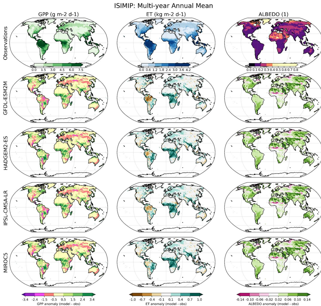
Figure 3: Multi-year annual mean for GPP (column 1), Evapotranspiration (Column 2) and Albedo (column 3) for observations (row 1) and subsequent rows show the anomaly compared with observations for each set of ISIMIP2b forcing data derived from: GFDL-ESM2M (row 2), HADGEM2-ES (row 3), IPSL-CM5A-LR (row 4) and MIROC5 (row 5). Observations are downloaded from iLAMB ( https://www.ilamb.org/doc/ilamb_fetch.html ) and the datasets shown are GBAF for GPP (Jung et al., 2011), GLEAM for ET (Miralles et al., 2011) and GEWEX.SRB for Albedo (Stackhouse et al., 2011).
