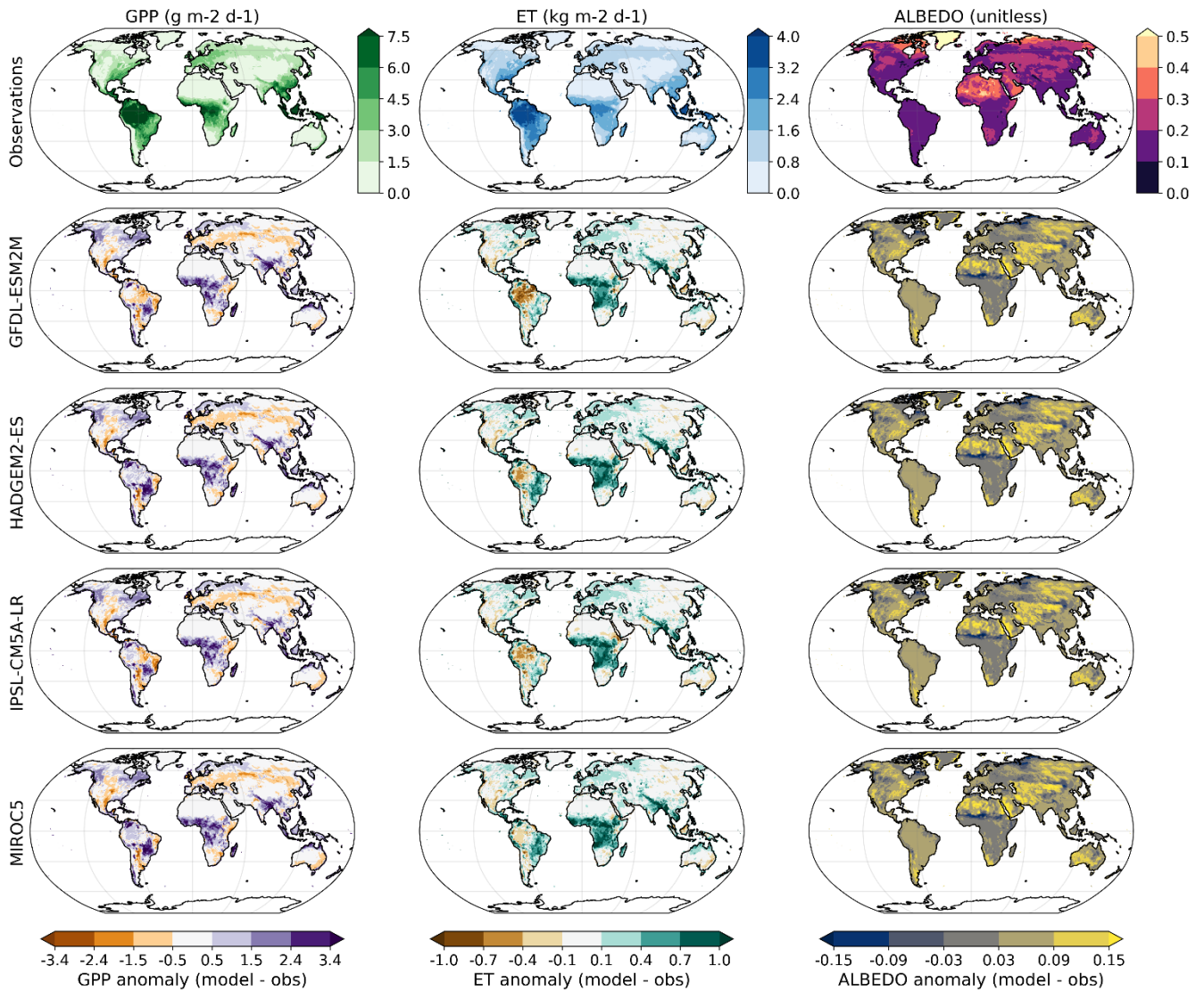
Figure 3: Multi-year annual mean for GPP (column 1), Evapotranspiration (Column 2) and Albedo (column 3) for observations (row 1) and subsequent rows show the anomaly compared with observations for each set of ISIMIP2b forcing data derived from: GFDL-ESM2M (row 2), HADGEM2-ES (row 3), IPSL-CM5A-LR (row 4) and MIROC5 (row 5). Observations are downloaded from iLAMB ( https://www.ilamb.org/doc/ilamb_fetch.html ) and the datasets shown are GBAF for GPP (Jung et al., 2011), GLEAM for ET ((Miralles et al., 2011) and GEWEX.SRB for Albedo (Stackhouse et al., 2011).
