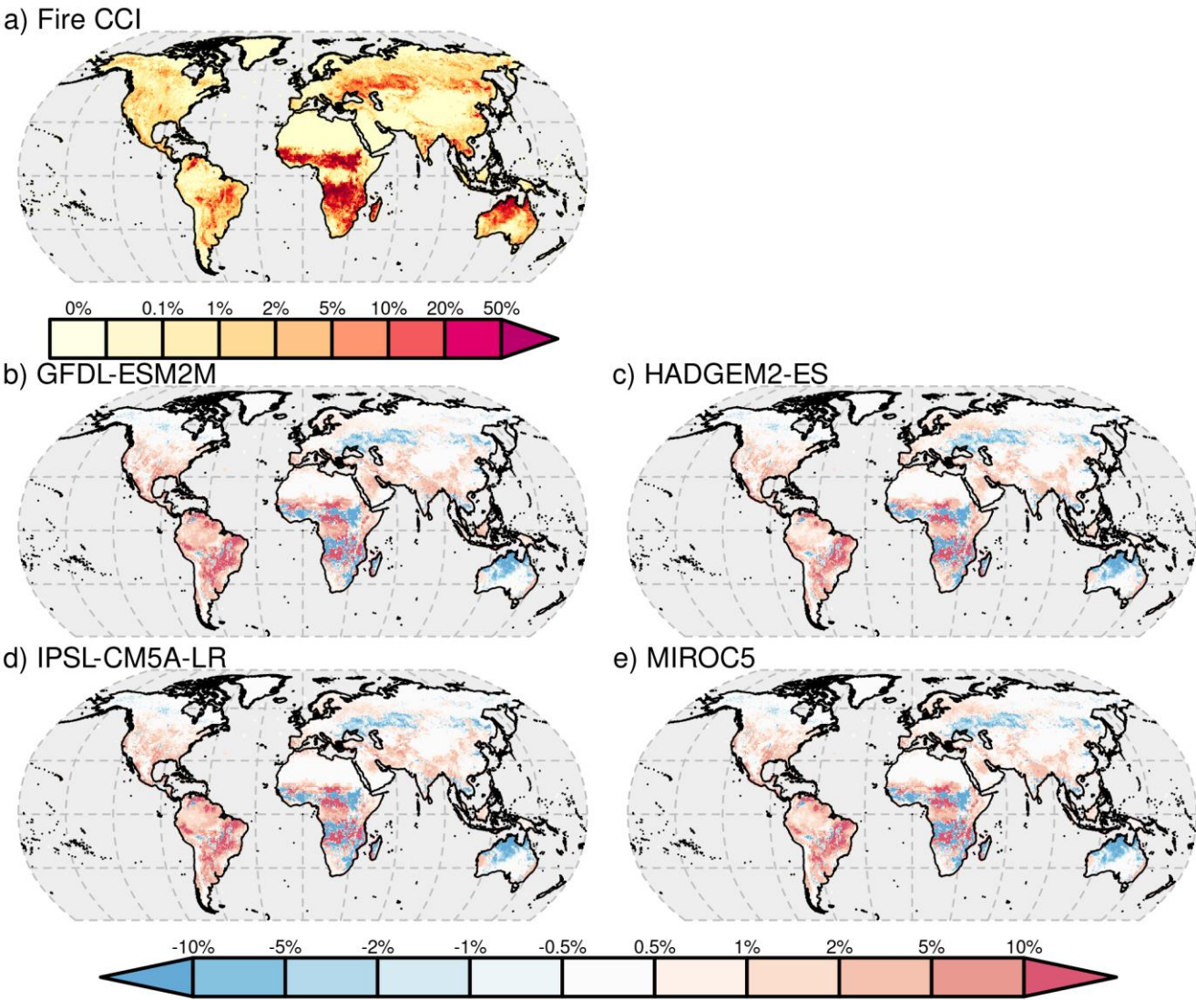
Figure 5: Present day percentage burned area (2000-2020) from and Fire CCI observations (a) and modelled by JULES driven by GFDL-ESM2M (b), HadGEM2-ES (c), IPSL-CM5A-LR (d), MIROC5(e)
