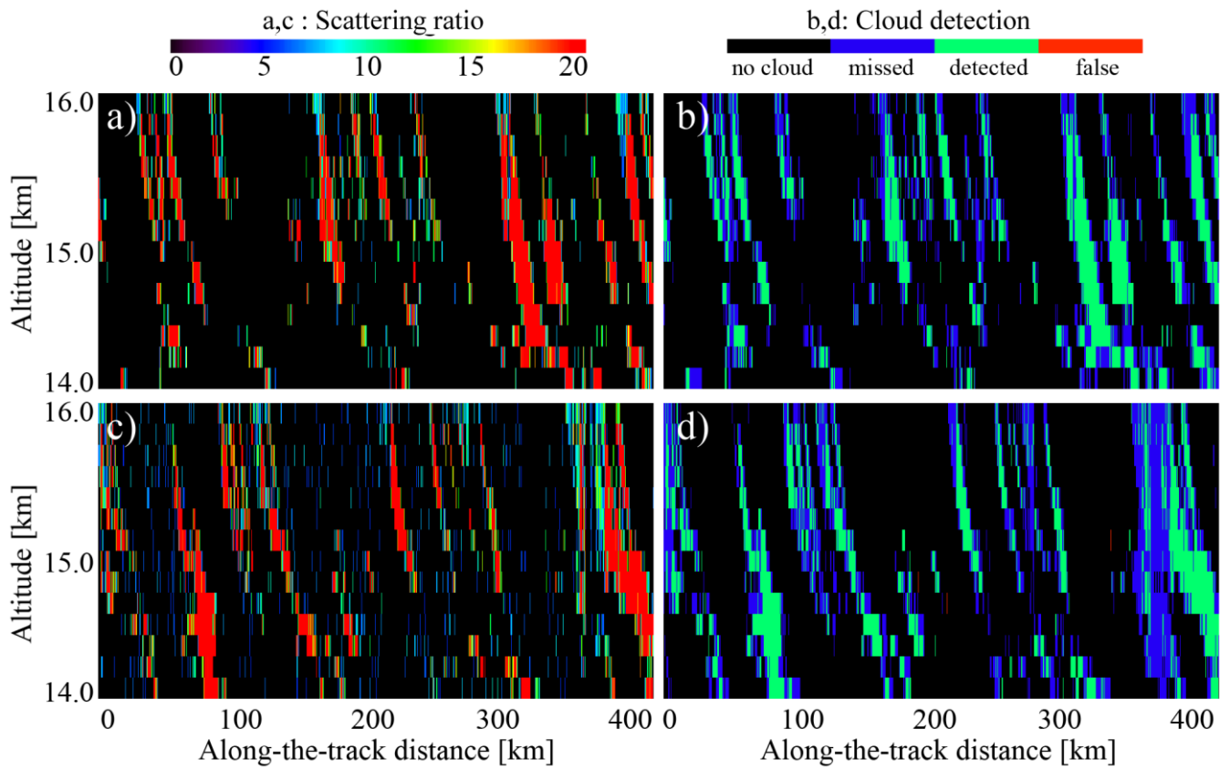
Figure 11: Same as figure 10, but for ATLID
