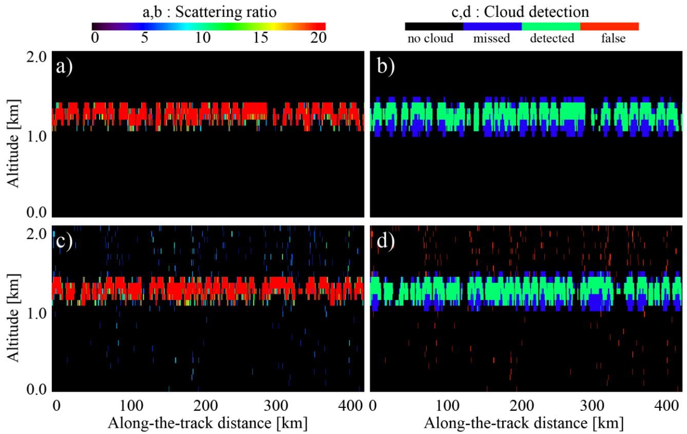
830 Figure A3: Scattering ratio and cloud detection statistics estimated for stratocumulus clouds observed by CALIOP using Eq. 6: (a) scattering ratio, night; (b) cloud detection, night; (c) scattering ratio, day; (d) cloud detection, day.
