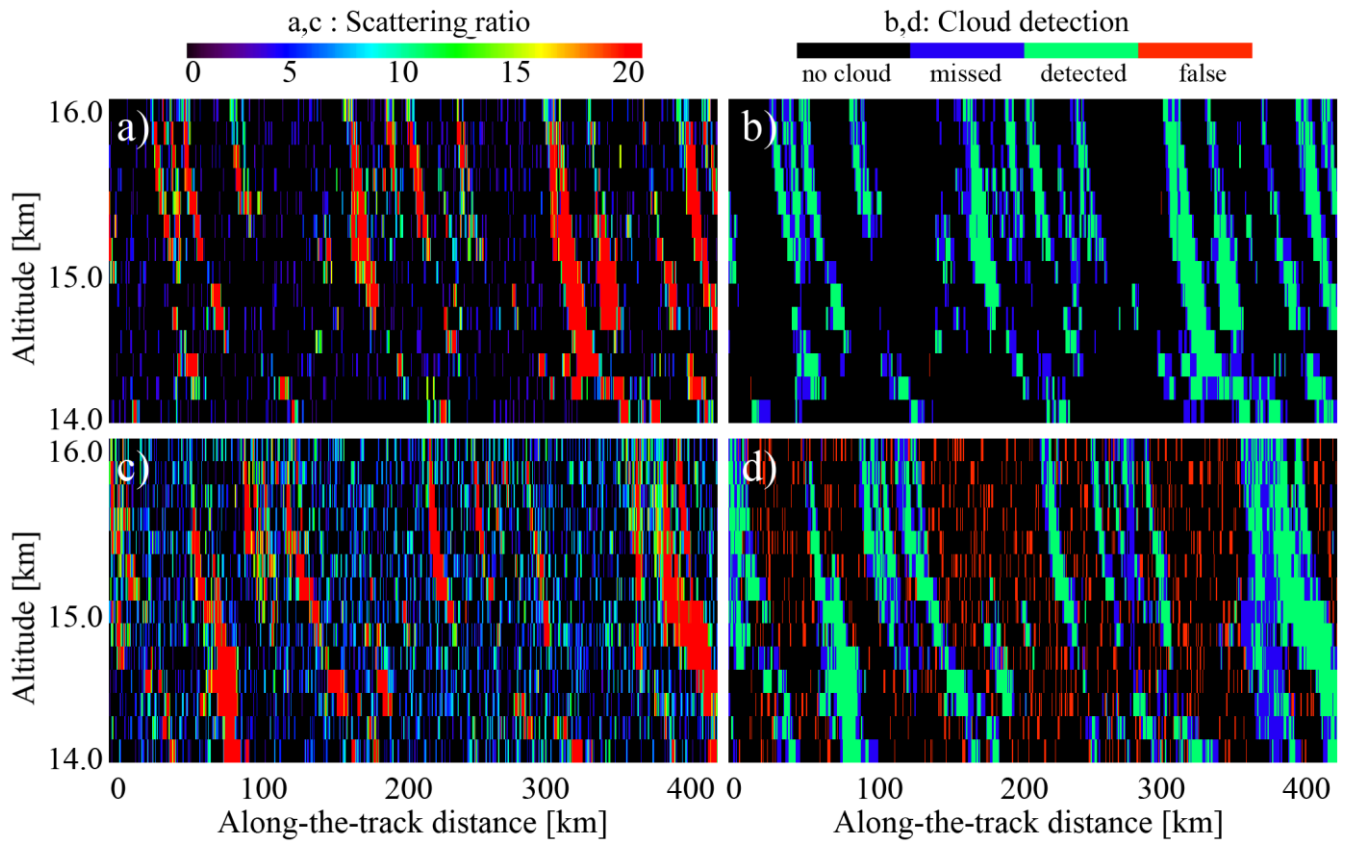
Figure 8: Scattering ratio and cloud detection estimated for cirrus clouds observed by CALIOP using Eq. 36: (a) scattering ratio, night; (b) cloud detection, night; (c) scattering ratio, day; (d) cloud detection, day. Note the color scale difference for (ac) and (bd).
