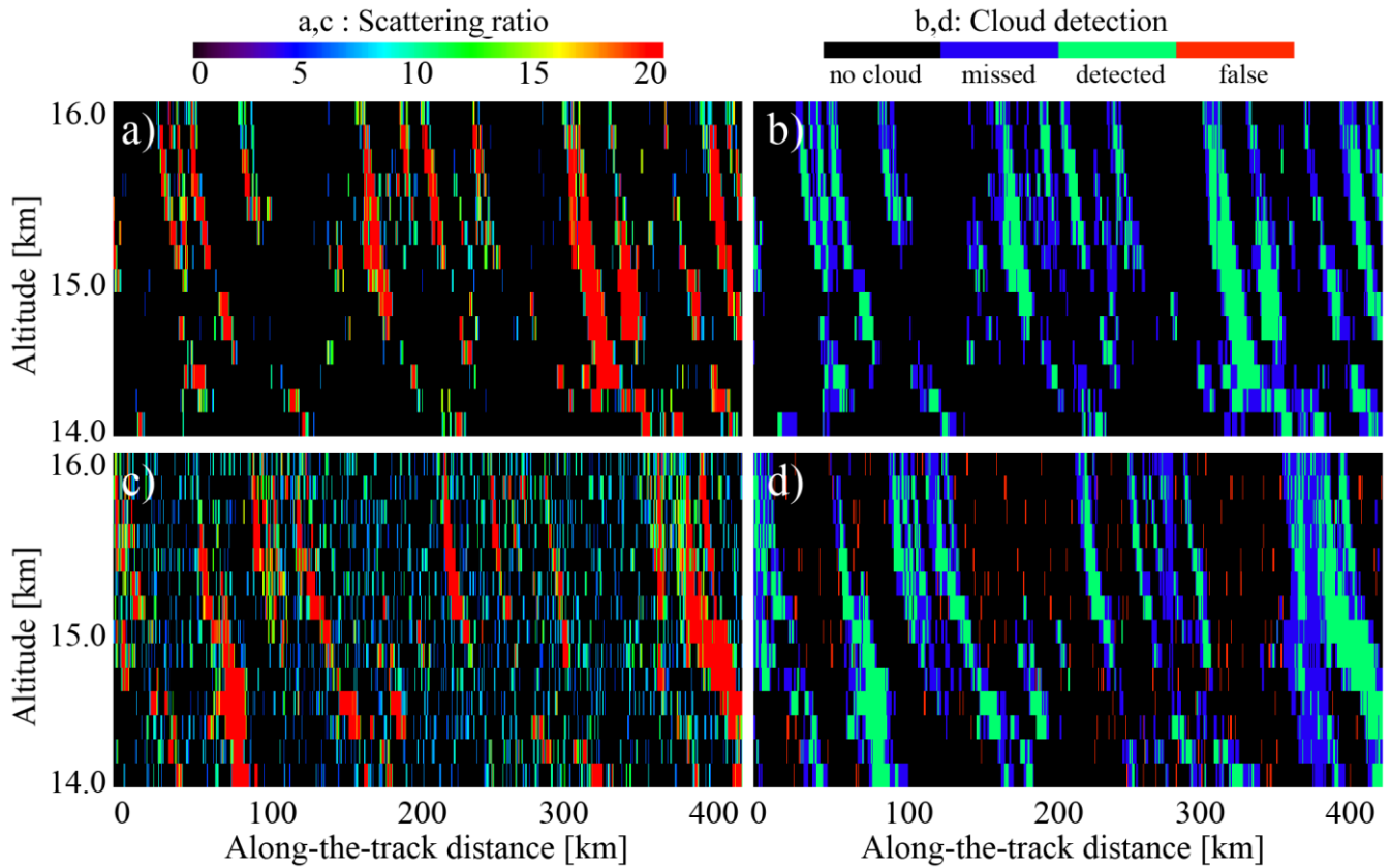
635 Figure 10: Scattering ratio and cloud detection statistics estimated for cirrus clouds observed by CALIOP using Eq. 6: (a) scattering ratio, night; (b) cloud detection, night; (c) scattering ratio, day; (d) cloud detection, day. Note the color scale difference for (ac) and (bd).
