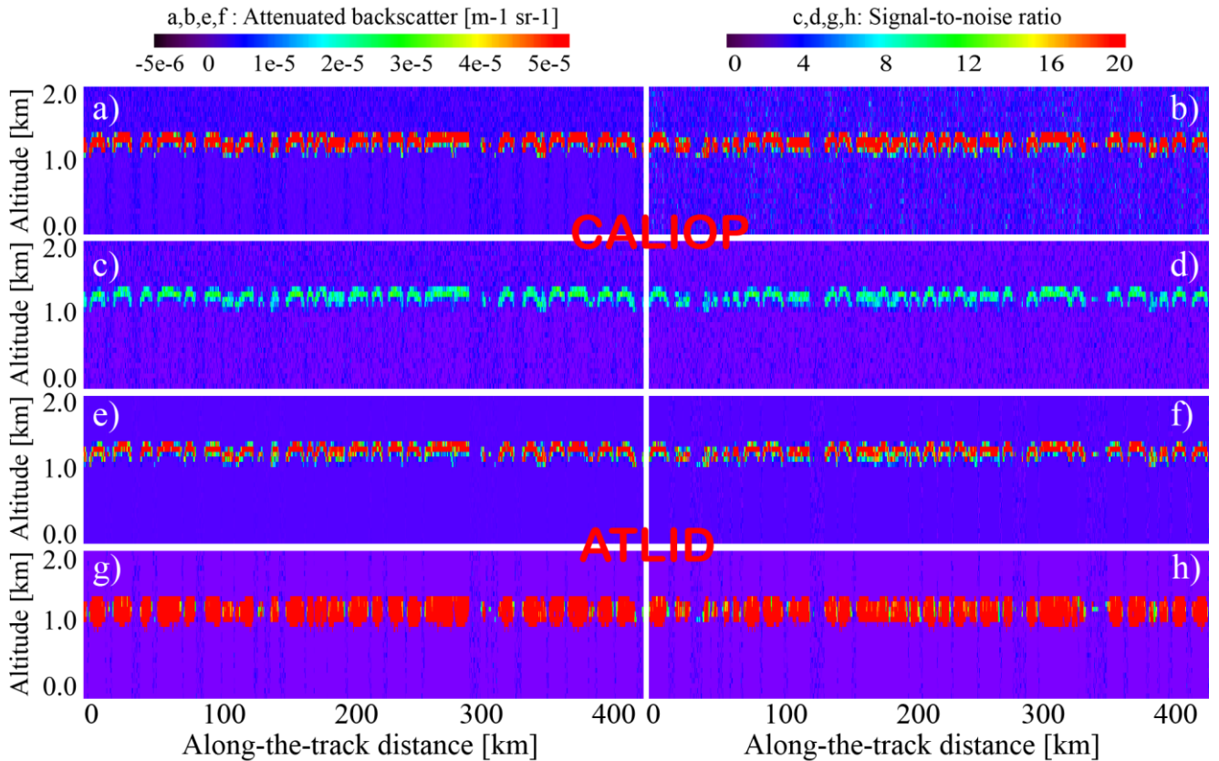
510 Figure 7: Same as Fig. 6, but for stratocumulus cloud scenes.
