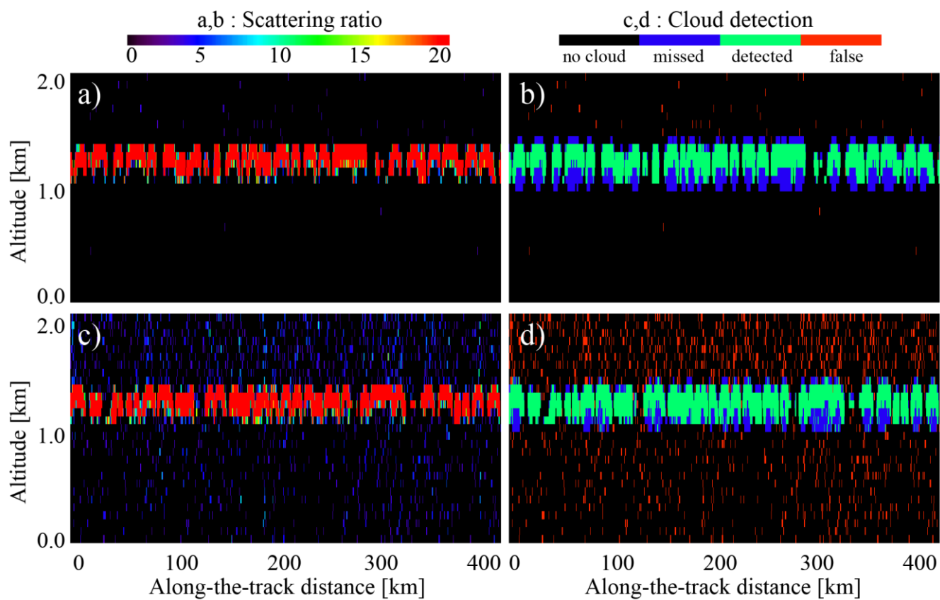
825 Figure A1: Scattering ratio and cloud detection statistics estimated for stratocumulus clouds observed by CALIOP using Eq. 36: (a) scattering ratio, night; (b) cloud detection, night; (c) scattering ratio, day; (d) cloud detection, day.
