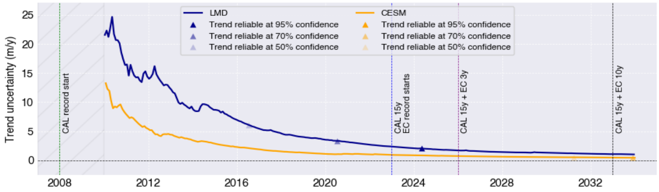
Figure 13 : Same as Fig. 12, but for the altitude of opacity Z_{opaque} instead of C_{opaque} .
