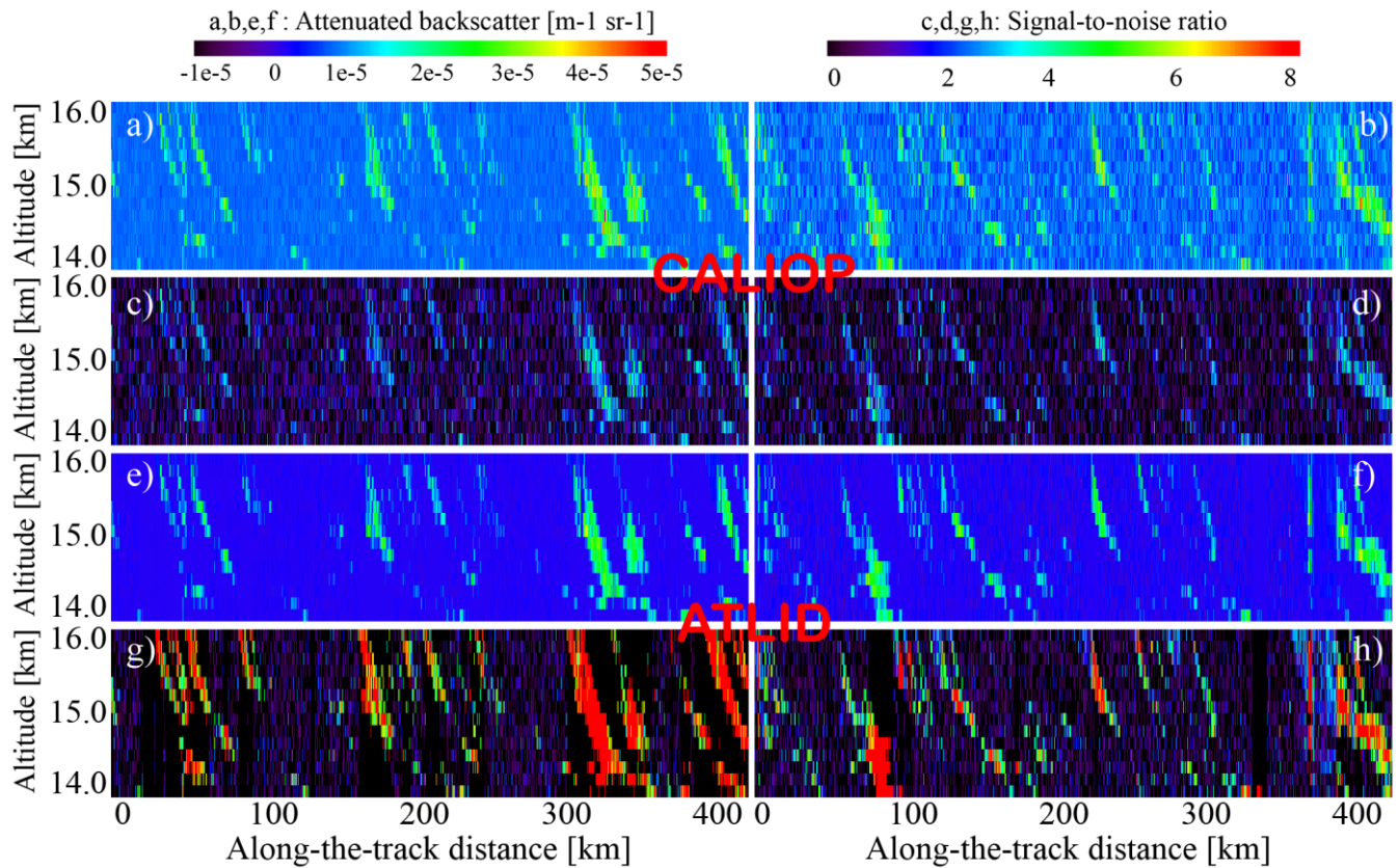
505 Figure 6: Signals and signal-to-noise ratio for cirrus cloud scene. CALIOP: (a) ATB(532nm, z), night for one piece of orbit; (b) ATB(532nm, z) day for another piece of pseudo-orbit; (c) SNR, night; (d) SNR, day; ATLID: (e) APB(355nm, z), night; (f) APB(355nm, z) day; (g) SNR, night; (h) SNR, day. Note that the scene contains only these clouds and a clear sky below. For the reflective clouds beneath the cirrus layer, the daytime noise will be higher (see the right-hand-side panels of Fig. 7).
