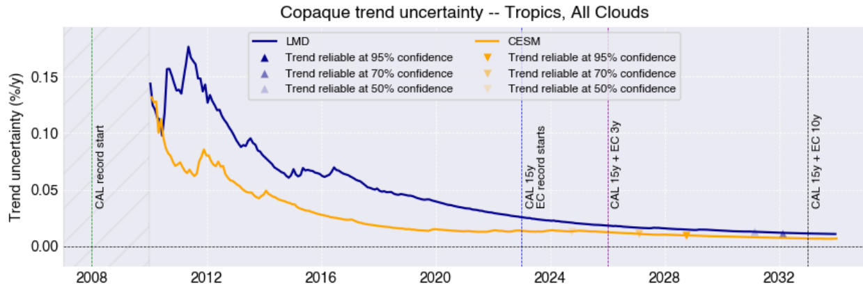
715 Figure 12: Evolution of the uncertainty in the C_{\text{opaque}} trend as a function of the length of the spaceborne lidar record, according to atmospheric conditions predicted by IPSL-CM6 (blue) and CESM (orange) in the period between 2008 and 2034 following the RCP85 scenario. The first two years of the record (2008-2010) are considered in the analysis, but trend uncertainties during that period are very large, and are masked in the figure to improve the legibility of later years. CALIPSO's planned end of operation (2023) is marked by a vertical blue line. Supposing EarthCARE begins operation right afterward, its nominal 3-years operation point is marked by a vertical purple line, and an optimistic 10-years operation point is marked by a vertical black line.
