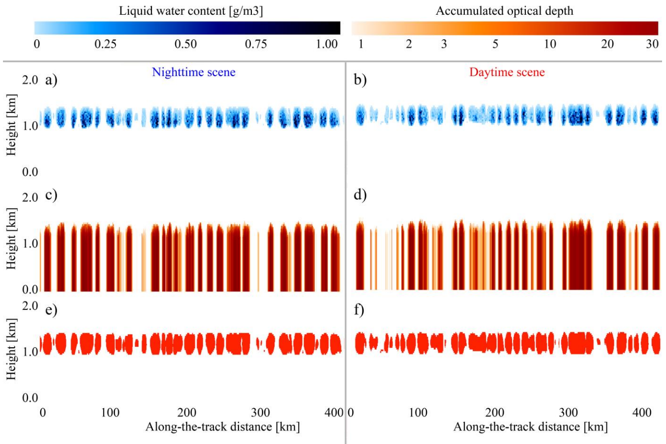
Figure 5: Same as Fig. 4, but for stratocumulus cloud scenes. Note the color scale difference between Fig. 4 and Fig. 5.
