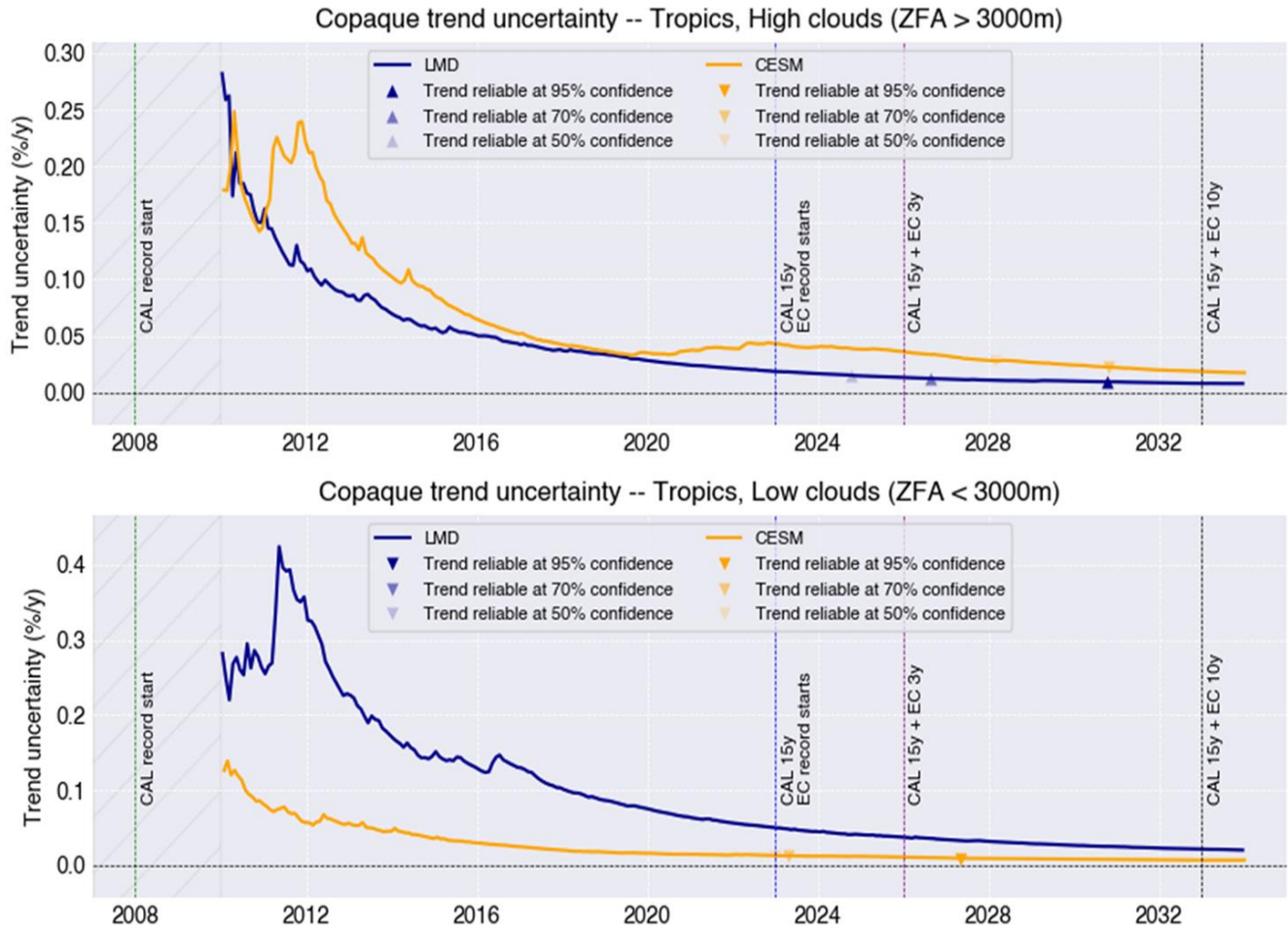
Figure B1: Same as Fig. 12, but with a separate analysis of high-levels clouds (top) and low-level clouds (bottom)
