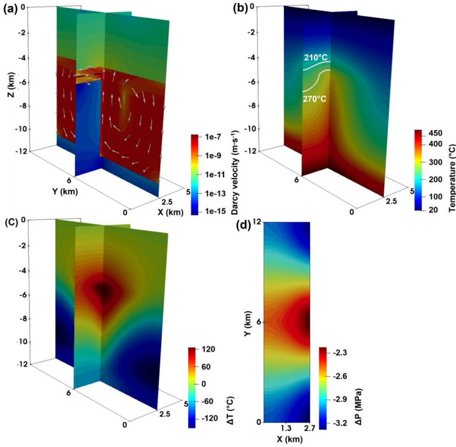
Figure 5. Fluid flow, temperature, and pore pressure change fields of the \kappa_{MF} = 10^{-15} \text{ m}^2 case at 1 Myr. Cross-sectional view of the (a) flow field with arrows representing the preferential fluid flow pathways; (b) resulting temperature field. The 210 °C and 270 °C are highlighted to indicate the dominant heat transfer types; (c) temperature differences compared to the initial conductive temperature distribution; (d) top view of the pore pressure change compared to the initial hydrostatic pore pressure (43.3 MPa) in the western sandstone, transfer faults, and main fault at a depth of 4.4 km. The 1.3 km and 2.7 km along the X-axis follow the west boundary of the Piesberg Quarry and the eastern boundary of the main fault, respectively.
