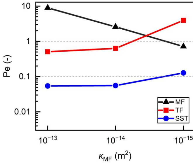
Figure 6. Effects of the main fault permeability ( \kappa_{MF} ) on the Pe (median Peclet numbers) of the main fault (MF), transfer faults (TF), and sandstone (SST).
