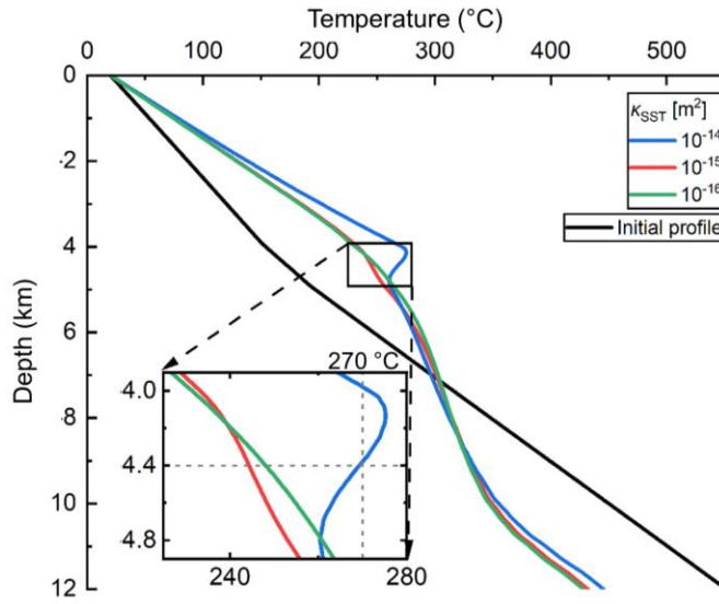
Figure 10. Effects of the sandstone permeability ( \kappa_{\text{SST}} ) on the temperature-depth profiles. The \kappa_{\text{SST}} = 10^{-15} \text{ m}^2 case represents the reference case.
