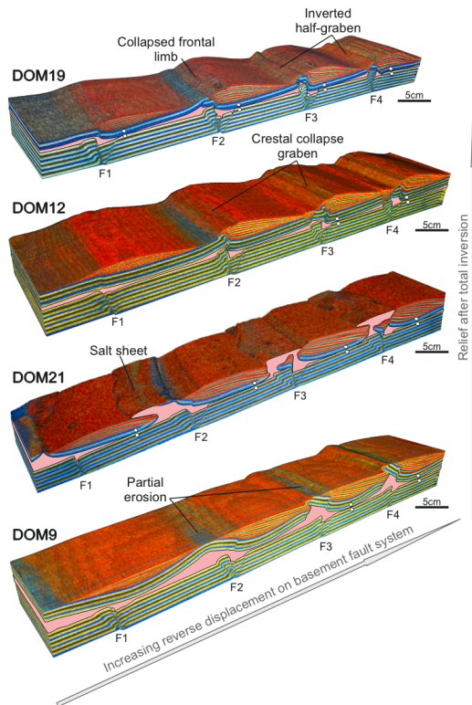
1660 Figure 8. 3D Voxels of DOM19, DOM12, DOM21, DOM9 displaying the effect that the decoupling layer is having in the development of overburden structural relief after total inversion. Notice how faults close to the moving wall display more reverse displacement due to the apparatus design.
