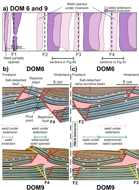
Figure 9. Weld reactivations. a) Map overlapping the weld distribution after extension and inversion. b) Weld reactivation example located above a basement extensional fault , c) Weld reactivation example located below the salt-detached ramp-syncline basin . See figure 5 for fault labeling.
