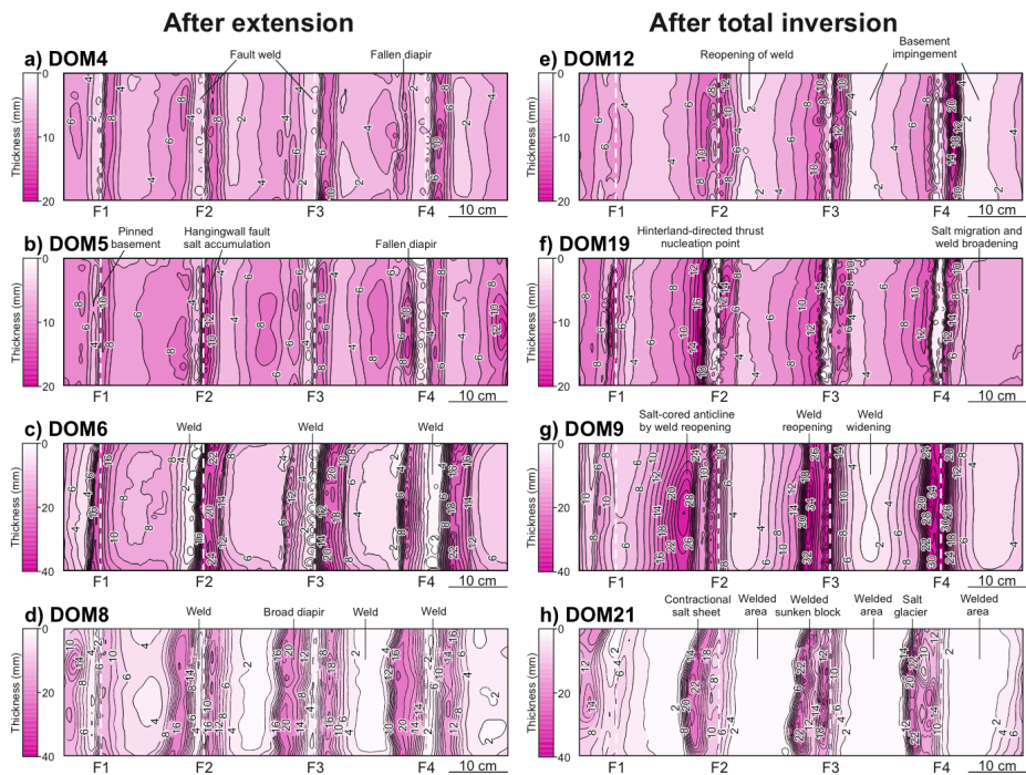
1645 Figure 6. Salt isopach maps after extension (a to d) and after total inversion (e to h). Notice how the scale range in models DOM6, DOM8, DOM 9 and DOM21 (c, d, g and h) is double the range of the other models.
