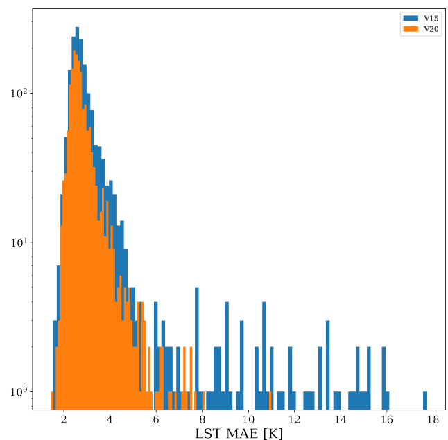
Figure 8. Distribution of prediction errors in the LST for all grid points in the Lake Updates category for VESPER_V15 and VESPER_V20. Each prediction errors is in turn the average of 4 trained iterations of the VESPER model. The predictions of VESPER_V20 are evidently and improvement over VESPER_V15, especially for grid points with large LST errors.
