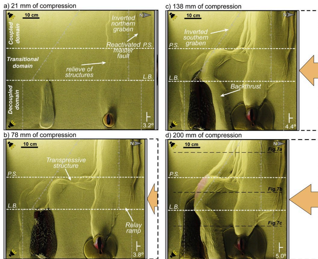
890 Figure 6: Overhead pictures showing the evolution of Model-2. Illumination comes from the left. The position of the basement rigid blocks is shown in grey dotted lines and the pinch out of the polymer (P.S.) and the limit of basement blocks (L.B.) in white dotted lines. a) Overhead view after 21 mm of shortening. b) Overhead view after 78 mm of shortening. c) Overhead view after 138 mm of shortening. d) Overhead view at the end of the experiment (200 mm shortening). No syn-tectonic sedimentation was performed during the compressional phase of this experiment.
