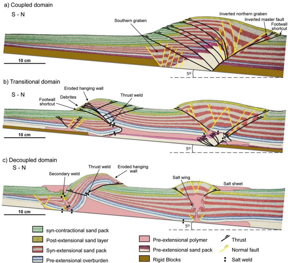
915 Figure 9: Cross-sections at the end of the Model-3 (after 200 mm of shortening) showing the structural style at the different domains. a) Coupled domain; b) Transitional domain; c) Decoupled domain. See figure 8d for location. After the deposition of each syn-compressional sand layer, the rig was tilted 0.2^\circ to the north up to additional 2.2^\circ to simulate the orogenic flexure of the Basque – Cantabrian Pyrenees.
