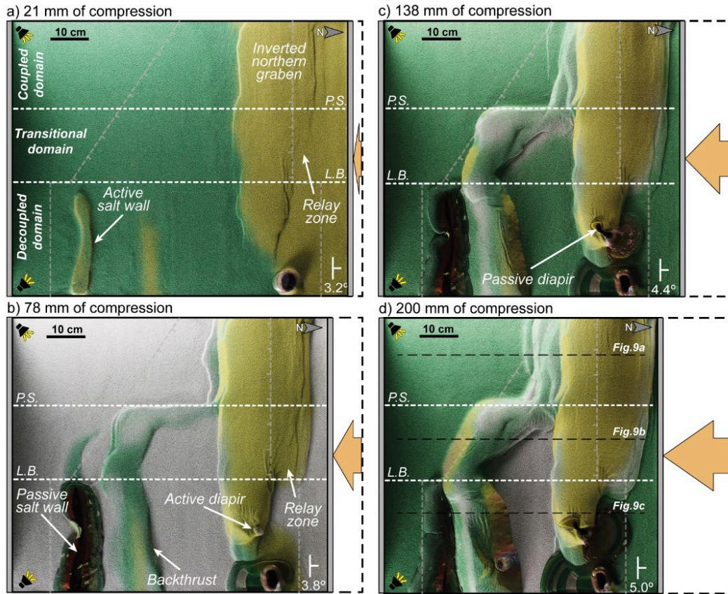
Figure 8: Overhead pictures showing the evolution of Model-3. Illumination comes from the left. The position of the basement rigid blocks is shown in grey dotted lines and the pinch out of the polymer (P.S.) and the limit of basement blocks (L.B.) in white dotted lines. a) Overhead view after 21 mm of shortening. b) Overhead view after 78 mm of shortening. c) Overhead view after 138 mm of shortening. d) Overhead view at the end of the experiment (200 mm shortening). Syn-orogenic sedimentation has been performed during the compressional phase of this experiment by adding alternating green and white sand layers every 3 hours.
