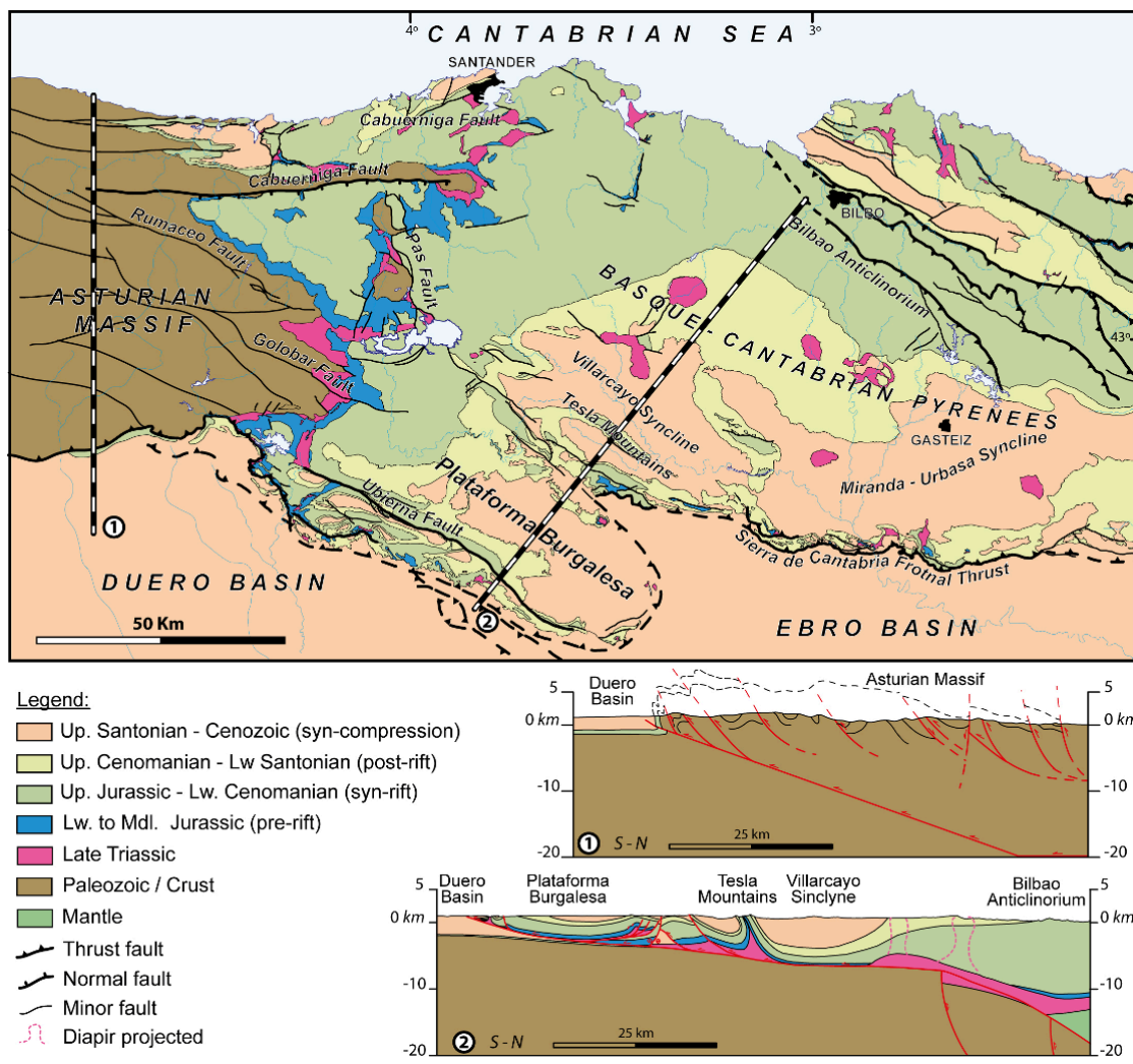
850 Figure 2: Tectonostratigraphic map of the Basque – Cantabrian Pyrenees – Asturian Massif junction (modified from Miró et al., 2021), and geological cross-section showing the along-strike variability of the structural style, from thick-skinned to the West to thin-skinned to the East. Cross-section 1 from Espina (1996) and cross-section 2 from Miró et al., 2021. BF: Becerril Fault, GF: Golobar Fault, RF: Rumaceo Fault, CF: Cabuérniga Fault.
