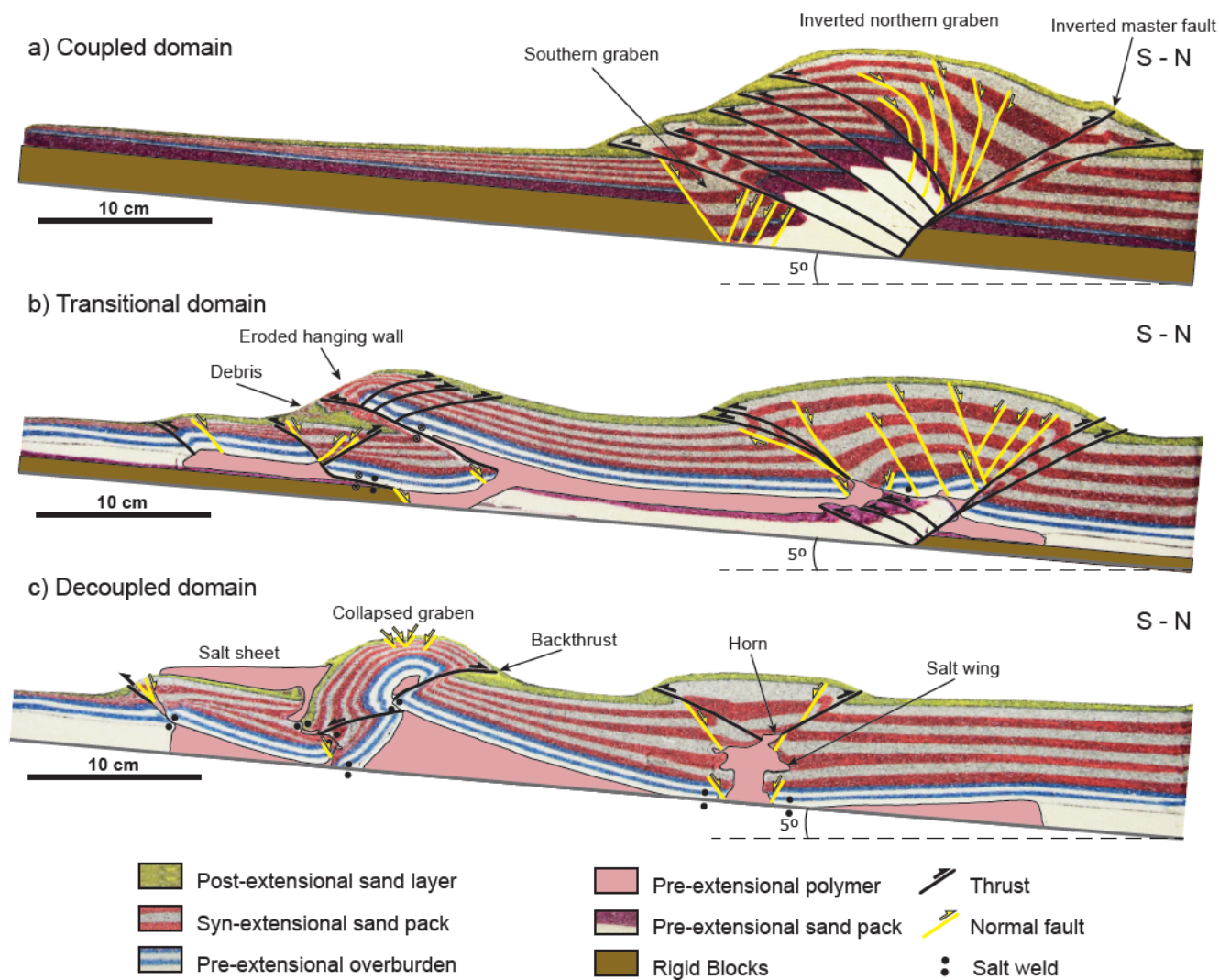
Figure 7: Cross-sections at the end of the Model-2 (after 200 mm of shortening) showing the structural style at the different domains. a) Coupled domain; b) Transitional domain; c) Decoupled domain. See figure 6d for location. The rig was tilted to the north up to additional 2.2° to simulate the orogenic flexure of the Basque – Cantabrian Pyrenees.
