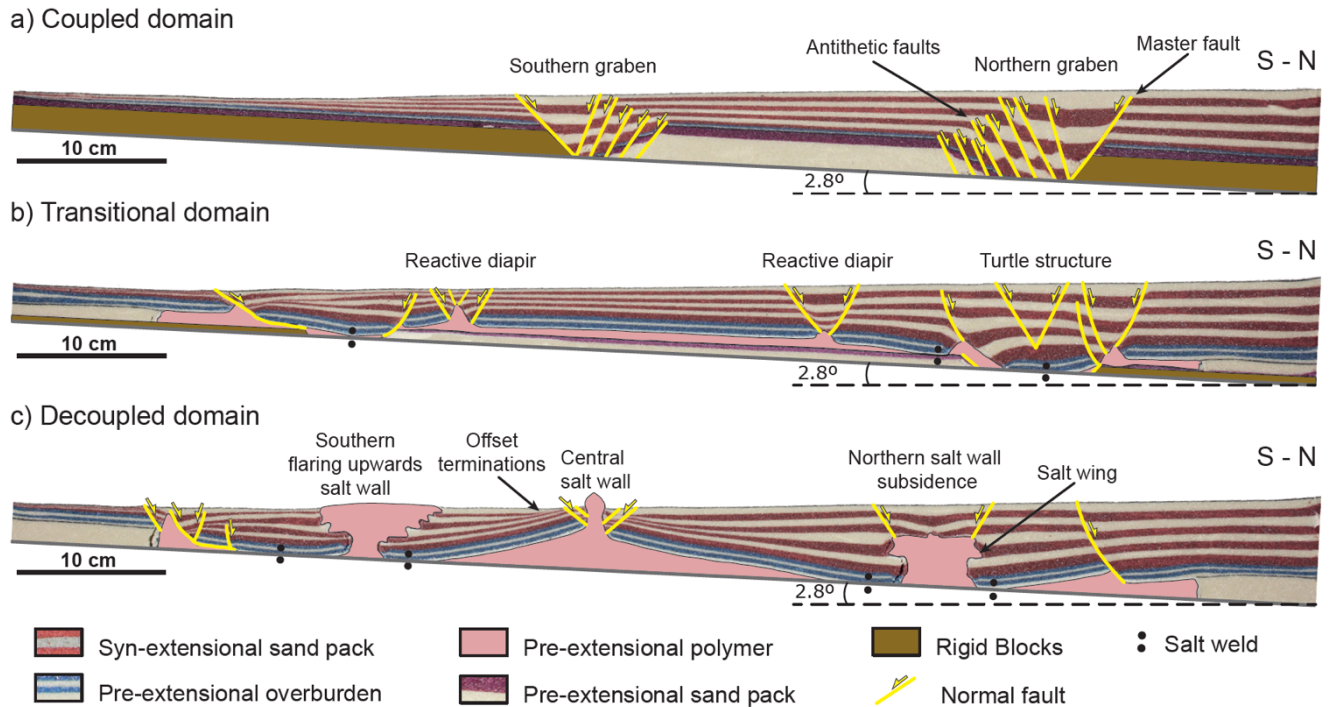
885 Figure 5: Cross-sections at the end of the extensional deformation (127 mm) across the different structural domains of Model-1. a) Coupled domain; b) Transitional domain; c) Decoupled domain. See Figure 4d for location. Before the sedimentation of each syn-extensional layer, the rig was tilted 0.35° northwards to simulate the progressive tilting of an extensional rifted margin reaching a regional dip of 2.8° at the end of the extensional phase.
