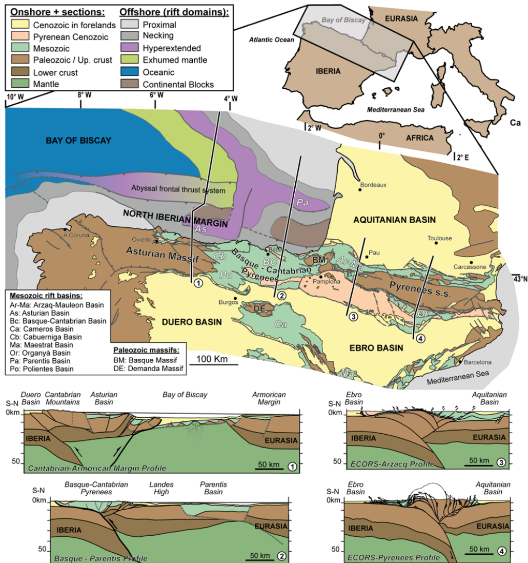
845 Figure 1: Structural map of the Pyrenean Orogen and surrounding areas with crustal cross-sections depicting the main along-strike structural changes. Rift domains are also mapped offshore. 1) Asturian Massif – Armorican Margin (Cadenas et al., 2018); 2) Basque – Cantabrian Pyrenees – Parentis (Ferrer et al., 2008 and Roca et al. 2011); 3) ECORS-Arzacq (Teixell, 1998); and 4) ECORS-Pyrenees (Muñoz, 1992).
