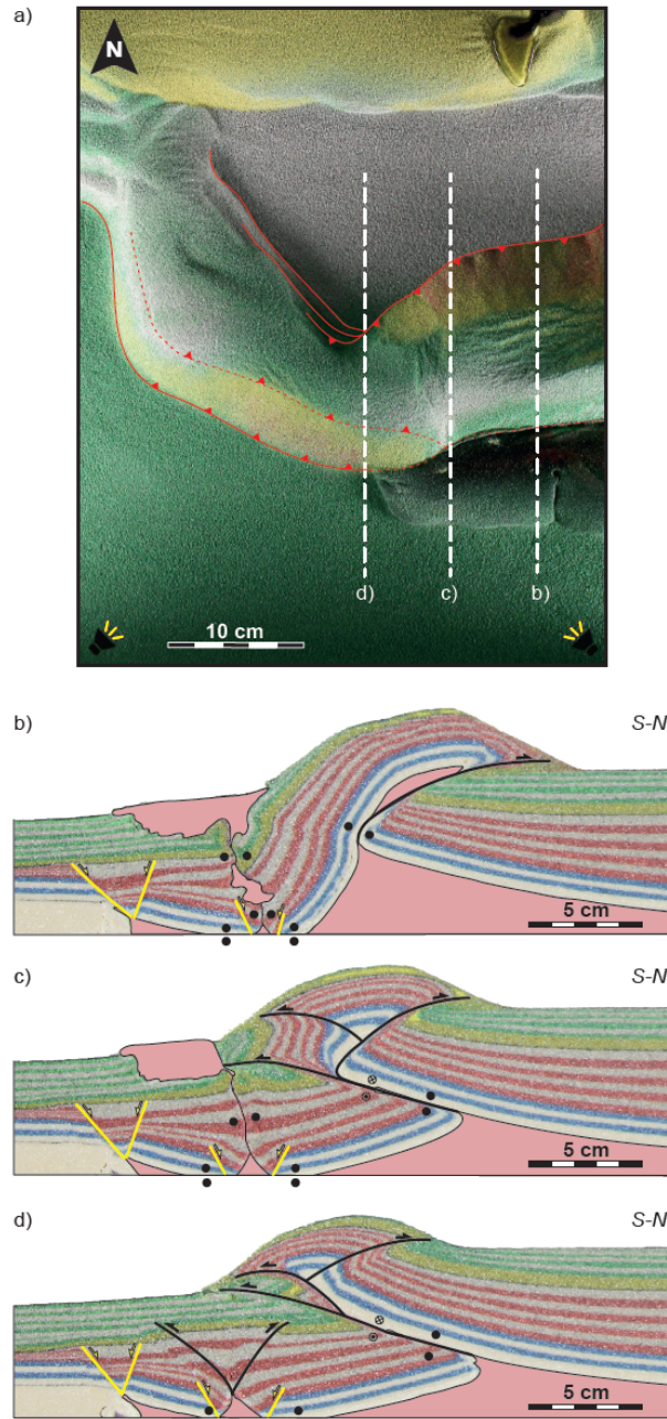
Figure 11: Detailed overhead view of Model-3 at the end of compressional deformation. b) to d) Detailed cross-sections showing the vergence variation between the decoupled and the transitional domains. See section's location in Figure 11a.
