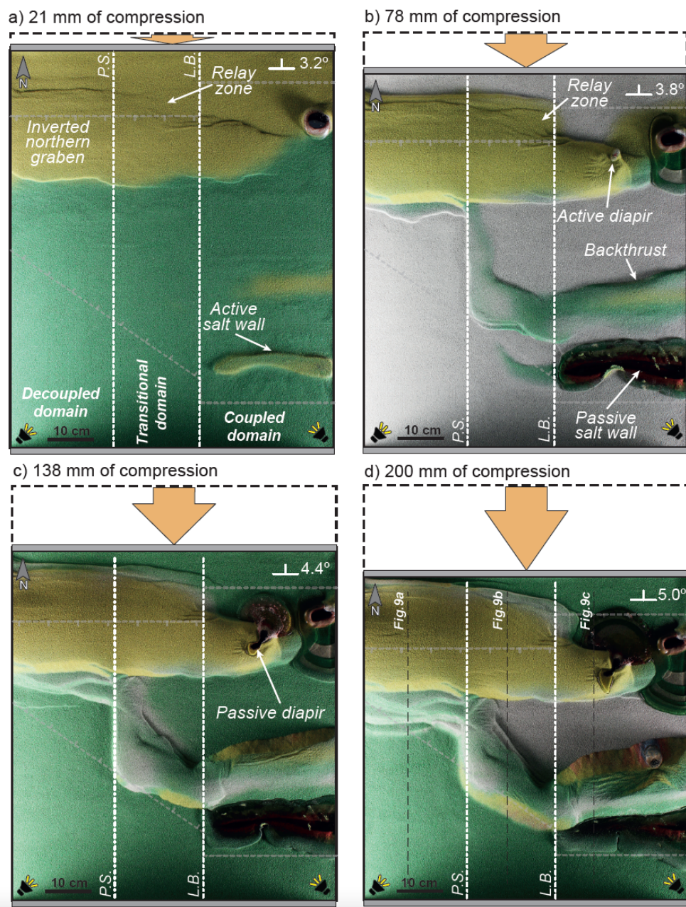
Figure 8: Overhead pictures showing the evolution of Model-3. Illumination comes from the left. The position of the basement rigid blocks is shown in grey dotted lines and the pinch out of the polymer (P.S.) and the limit of basement blocks (L.B.) in white dotted lines. a) Overhead view after 21 mm of shortening. b) Overhead view after 78 mm of shortening. c) Overhead view after 138 mm of shortening. d) Overhead view at the end of the experiment (200 mm shortening). Syn-orogenic sedimentation has been performed during the compressional phase of this experiment by adding alternating green and white sand layers every 3 hours.
