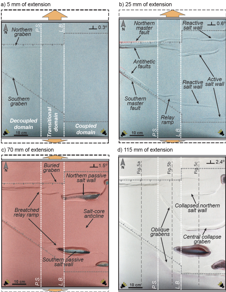
875 Figure 4: Overhead evolution of Model-1 during extension. Illumination comes from the left. The shadow areas are surface- breaching faults dipping to the right (North) and the illuminated ones are surface-breaching faults dipping to the left (South). The position of the basement rigid blocks is shown in grey dotted lines, and the polymer pinch out (P.S.) and the limit of basement blocks (L.B.) in white dotted lines. a) Overhead view after 5 mm of extension. b) Overhead view after 25 mm of extension. c) Overhead view after 70 mm of extension. d) Overhead view after 115 mm of extension. The external dashed reference rectangle corresponds to the dimensions of the experiment after 115mm of extension (step d) to show the movement of the two walls through time. The northern wall moved at a higher velocity than the southern one as represented by the arrows. 8 different layers (alternating red and white sand) were added during the extension.
