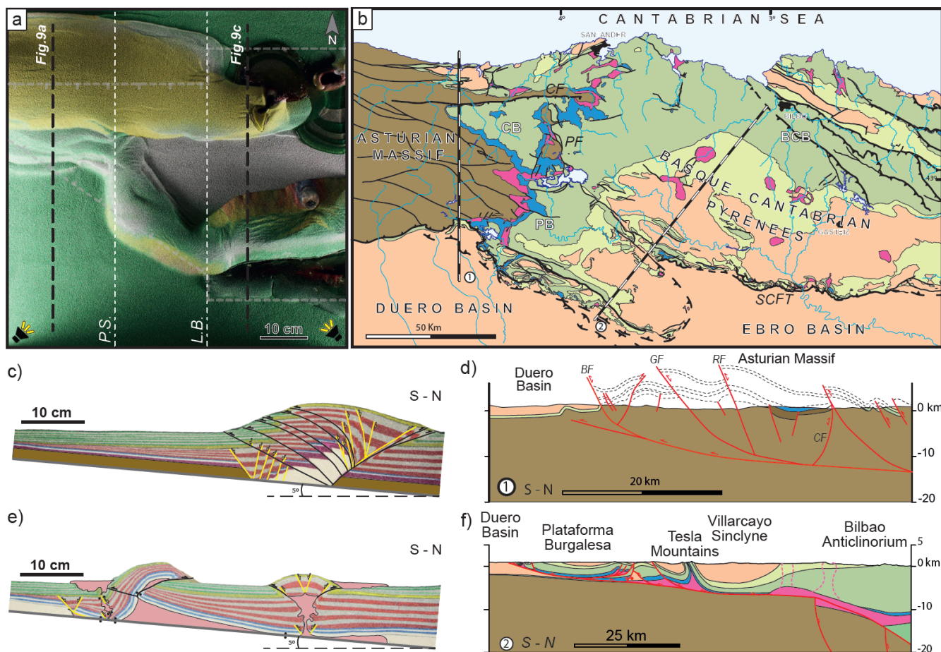
940 Figure 12: a) Overhead view of Model-3 at the end of the experiment. b) Tectonostratigraphic map of the Basque–Cantabrian Pyrenees – Asturian Massif junction (modified from Miró et al., 2021). c) Cross-section of the coupled domain showing the thick- skinned deformation in Model-3. d) Cross-section through the Asturian Massif (modified from Espina, 1996) showing the thick- skinned deformation similar to what was observed in the model. e) Cross-section through the decoupled domain in Model-3. f) 945 Cross-section across the southern Basque–Cantabrian Pyrenees showing the characteristic thin-skinned deformation of the area. BF: Becerril Fault, GF: Golobar Fault, RF: Rumaceo Fault, CF: Cabuérniga Fault.
