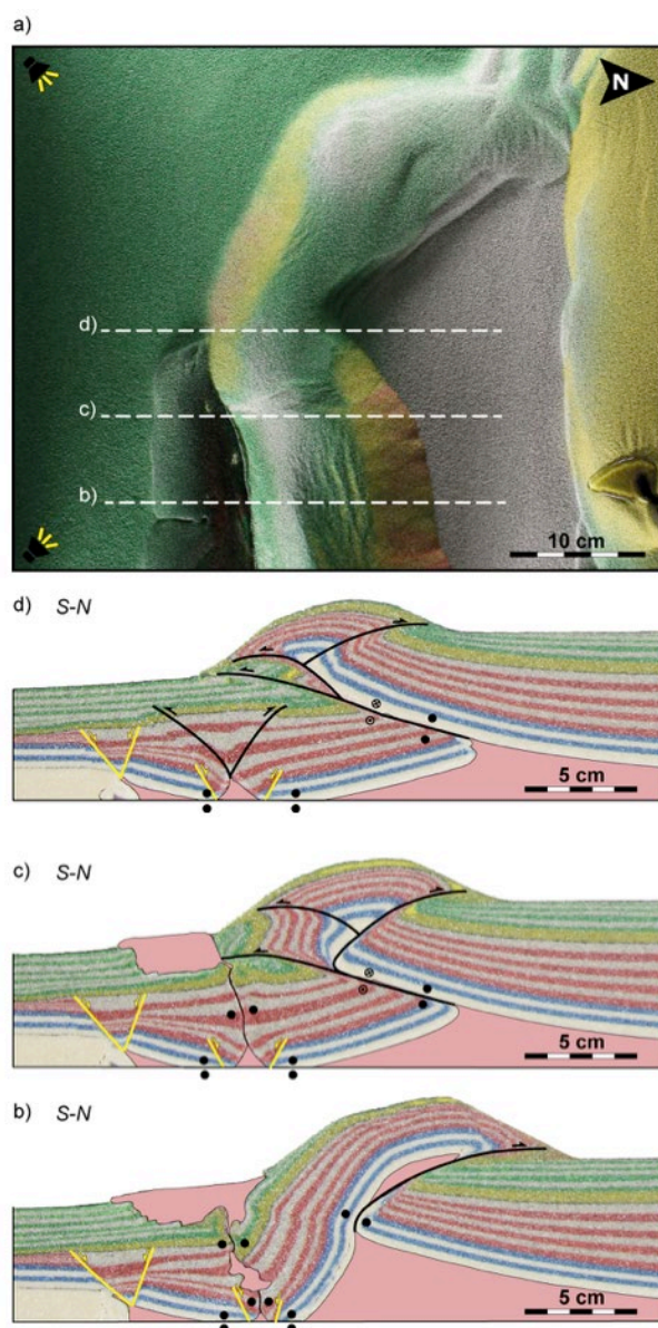
Figure 11: Detailed overhead view of Model-3 at the end of compressional deformation. b) to d) Detailed cross-sections showing the vergence variation between the decoupled and the transitional domains. See section's location in Figure 11a.
