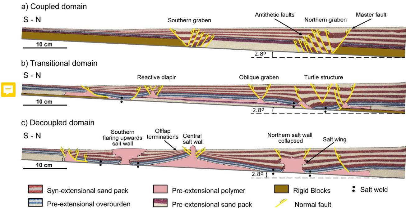
Figure 5: Cross-sections at the end of the extensional deformation (127 mm) across the different structural domains of Model-1. A) Coupled domain; B) Transitional domain; C) Decoupled domain. See Figure 4D for location.
