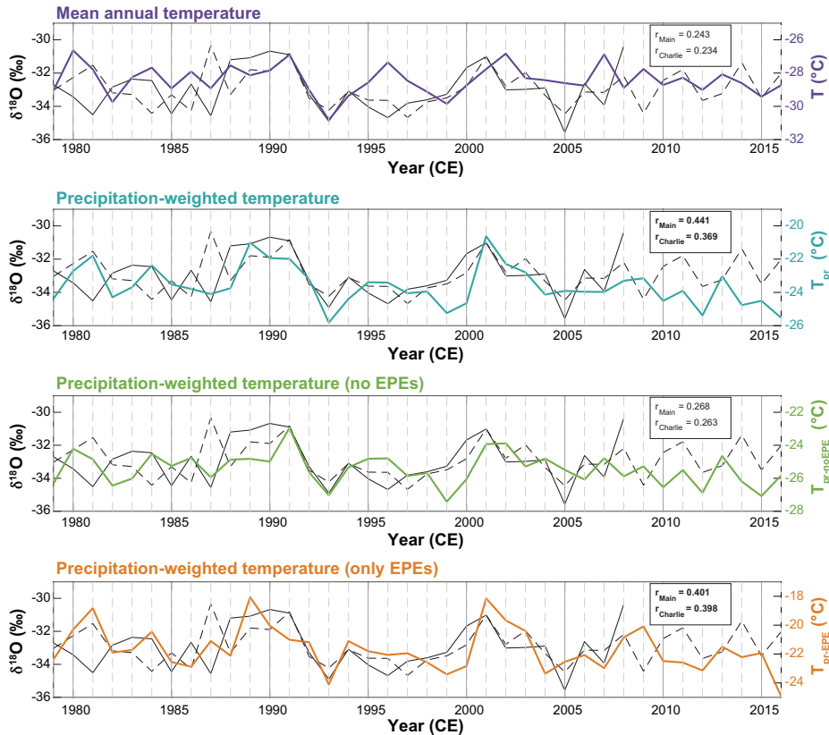
Figure 8: Annually-averaged \delta^{18}\text{O} from MBS-Main (solid black line) and MBS-Charlie (dashed black line) and a) mean annual temperature ( T ; purple line); b) precipitation-weighted temperature ( T_{pr} ; teal line); c) precipitation-weighted temperature with accumulation from EPEs removed ( T_{pr-noEPE} ; green line); and d) precipitation-weighted temperature based only on accumulation from EPEs ( T_{pr-EPE} ; orange line). All temperature time-series are constructed using daily mean temperature and total daily precipitation from ERA-5. Pearson's correlation coefficients r for MBS-Main and MBS-Charlie with the temperature time-series are shown for each panel, with significant correlations ( p < 0.05 ) in bold.
