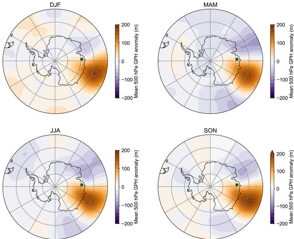
030 Figure A3: Mean 500 hPa geopotential height anomaly for all EPE days identified using RACMO2.3p2 from 1979-2016 for each 035 season (DJF, MAM, JJA, SON) relative to the mean from ERA-5. Grey bars indicate the regions between which the blocking index 040 is calculated.
