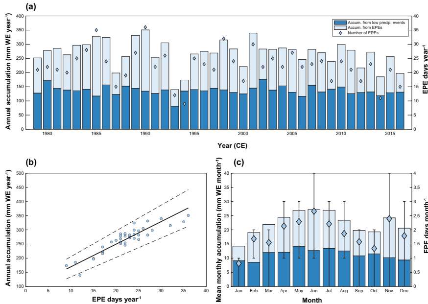
450 Figure 3: a) Annual accumulation at MBS from ERA-5 for 1979-2016. Accumulation from non-EPE precipitation days is shown in 455 dark blue, and accumulation from EPE's in light blue. The blue diamonds indicate the number of EPE days in a year. b) Annual accumulation at MBS versus number of extreme precipitation days in a year. The solid line indicates the linear regression, with dashed lines indicating uncertainty in the regression ( r = 0.91 ). c) Mean monthly precipitation at MBS from ERA-5 for 1979-2016. Colours are as in a). Blue diamonds represent the mean number of EPE days per month, with error bars indicating the upper and lower quartiles.
