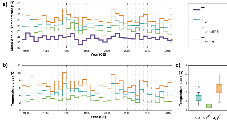
760 Figure 6: a) Mean annual temperature from ERA-5 for 1979-2016 at MBS (bold purple line) and the mean annual precipitation- 765 weighted temperature time-series for the same period ( T_{pr} : blue line; T_{pr-noEPE} : green line; T_{pr-EPE} : orange line). b) Temperature difference between the mean annual precipitation-weighted temperature time-series ( T_{pr} : blue line; T_{pr-noEPE} : green line; T_{pr-EPE} : orange line) and mean annual temperature. c) Box plot showing the temperature difference between the mean annual precipitation-weighted temperature time-series ( T_{pr} : blue box; T_{pr-noEPE} : green box; T_{pr-EPE} : orange box) and mean annual temperature.
