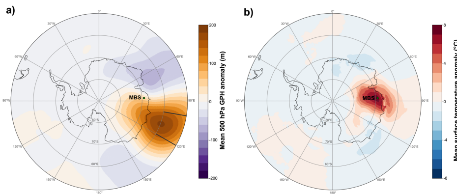
485 Figure 4: a) Mean 500 hPa geopotential height anomaly relative to the seasonal mean for all EPE days identified using ERA-5 from 1979-2016. Grey bars indicate the regions between which the blocking index is calculated. b) Mean surface temperature anomaly relative to the seasonal mean for all EPE days identified using ERA-5 from 1979-2016.
