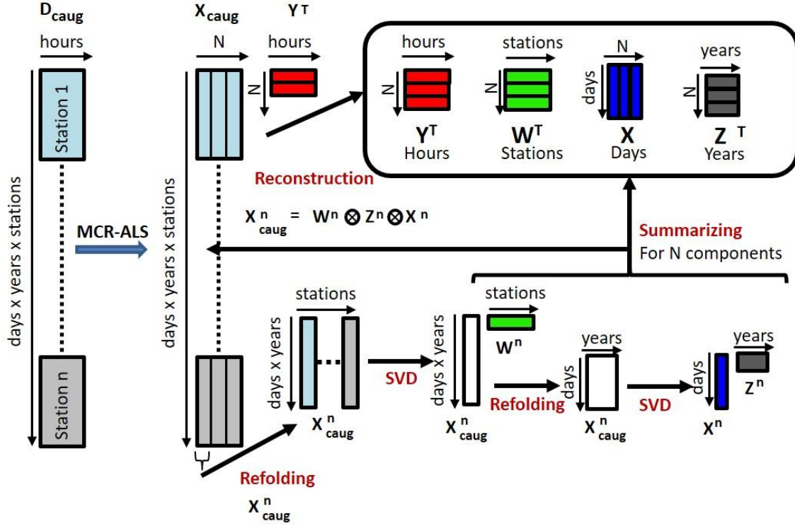
Figure 2. MCR-ALS with the quadrilinearity constraint. Graphical description of the implementation of the quadrilinearity constraint during the Alternating Least Squares optimization. See Eq. (4-7) and their explanation in the manuscript.
