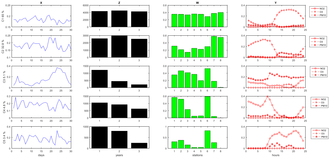
Figure 7. MCR-ALS analysis of NO_2 , O_3 and PM_{10} concentrations in the column-wise super-augmented incomplete April data matrix DA12_{craug} (see Eq. (9)) using non-negativity and quadrilinearity constraints. Profiles of the four different data modes are given in different colors: (X) in blue days of the year; (Z) in black year 1=2018, 2=2019 and 3= 2020; (W) in green stations 1: Vall d'Hebron, 2: Granollers, 3: Manlleu, 4: Juneda, 5: Bellver, 6: Gràcia, 7: Begur, 8: Observatori Fabra; and (Y) in red, hours of the day.
