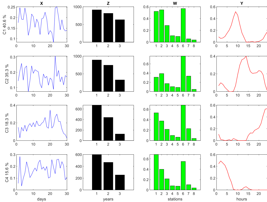
Figure 4. MCR-ALS analysis of NO 2 concentrations in the column-wise super-augmented data matrix D_{\text{caug-April-NO}_2} (Eq. (3)) using non-negativity and quadrilinearity constraints. Profiles of the four different data modes are given in different colors: (X) in blue days of April; (Z) in black year 1=2018, 2=2019 and 3= 2020; (W) in green stations 1: Vall d’Hebron, 2: Granollers, 3: Manlleu, 4: Juneda, 5: Bellver, 6: Gràcia, 7: Begur, 8: Observatori Fabra; and (Y) in red, hours of the day.
