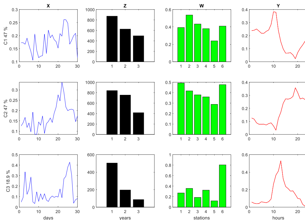
Figure 6. MCR-ALS analysis of PM 10 concentrations in the column-wise super-augmented data matrix \mathbf{D}_{\text{caug-April-PM}_{10}} (Eq. (3)) using non-negativity and quadrilinearity constraints. Profiles of the four different data modes are given in different colors: (X) in blue days of April; (Z) in black year 1=2018, 2=2019 and 3= 2020; (W) in green stations 1: Vall d'Hebron, 2: Granollers, 3: Manlleu, 4: Juneda, 5: Bellver, 6: Gràcia; and (Y) in red, hours of the day.
