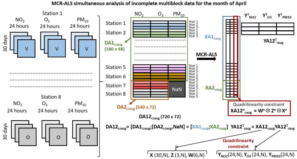
Figure 3. MCR-ALS with the quadrilinearity constraint for the simultaneous analysis of the three contaminants in the incomplete multiblock data set of the month of April. See Eq. (9) and their explanation in the manuscript.
