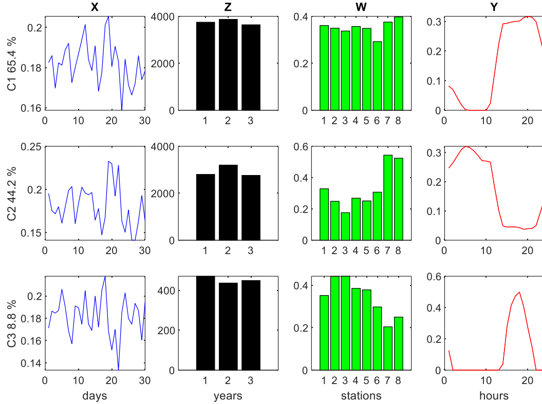
Figure 5. MCR-ALS analysis of O_3 concentrations in the column-wise super-augmented data matrix D_{\text{caug-April-}O_3} (Eq. (3)) using non-negativity and quadrilinearity constraints. Profiles of the four different data modes are given in different colors: (X) in blue days of April; (Z) in black year 1=2018, 2=2019 and 3= 2020; (W) in green stations 1: Vall d'Hebron, 2: Granollers, 3: Manlleu, 4: Juneda, 5: Bellver, 6: Gràcia, 7: Begur, 8: Observatori Fabra; and (Y) in red, hours of the day.
