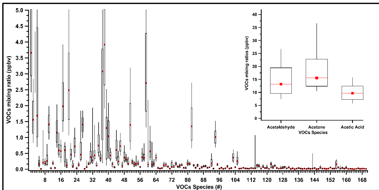
Figure S2: Box plots showing the concentrations individual NMVOCs over the whole study period. The Box represents the 25-75% inter-quartiles of the data with highest and lowest points as whiskers. The middle red box is the mean of the concentrations of individual NMVOCs.
