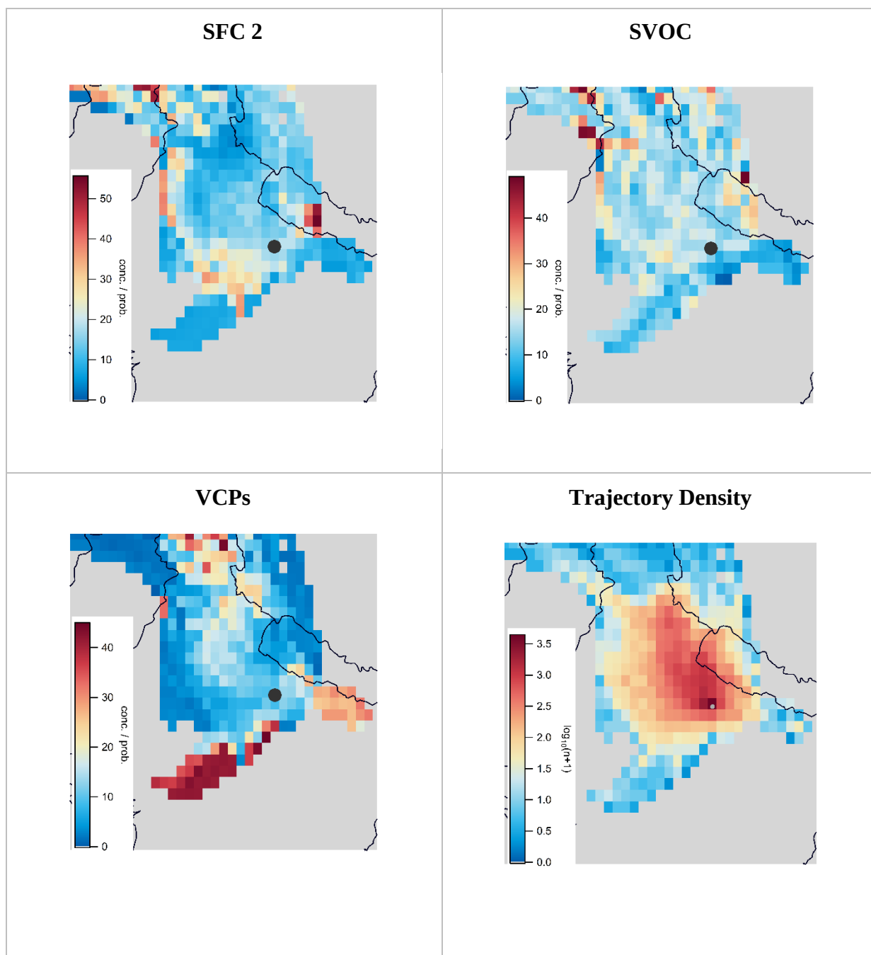
Figure S3: Graphs showing concentration weighted trajectories for individual factors (Traffic, SFC1, SFC 2, SVOC, VCPs), and trajectory density also for the sampling site in Lucknow.
