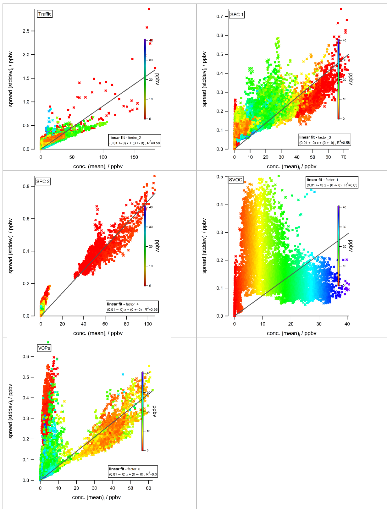
Figure S5: Mass estimation error for individual factors after bootstrap analysis.
