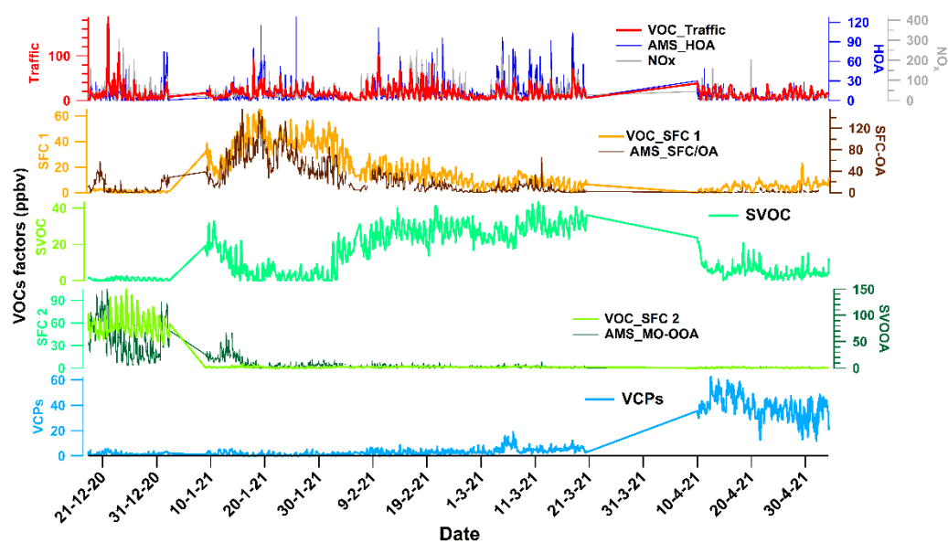
Figure S7: Timeseries of 5-factor solution of NMVOCs, correlated with AMS_organic aerosols resolved factors and NOx
