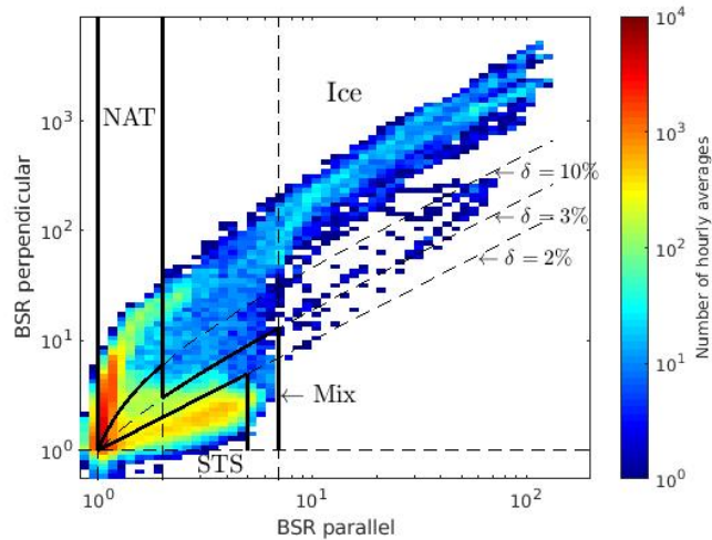
Figure 2. Frequency of backscatter ratios (BSR) of parallel versus perpendicular channel for all PSC observations with the IRF lidar. Parameter ranges for PSC types NAT, STS, and Ice are indicated by thick, solid lines. Lines for some constant depolarisation ratio \delta and some constant backscatter ratios are added for reference (dashed lines).
